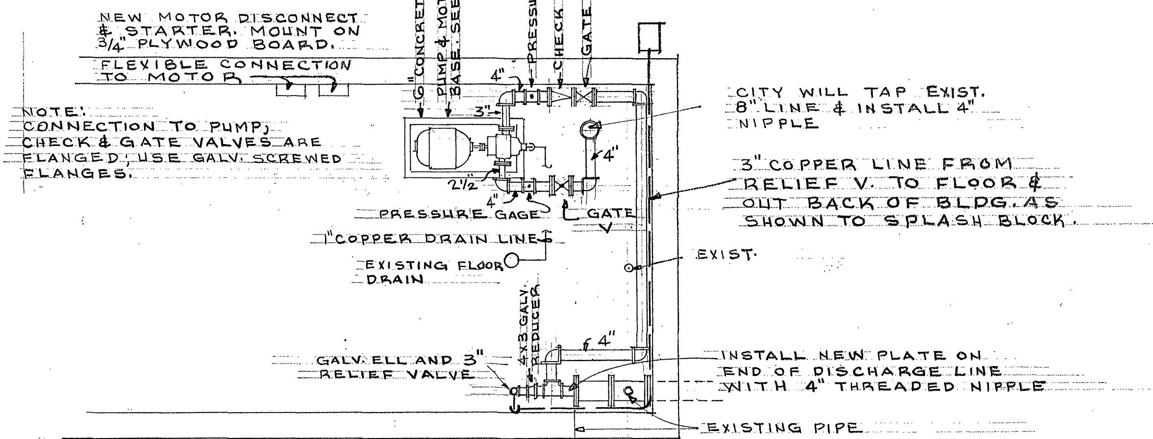
PARTIAL GROUND FLOOR PLAN SCALE: 1/4" = 1'-0"
