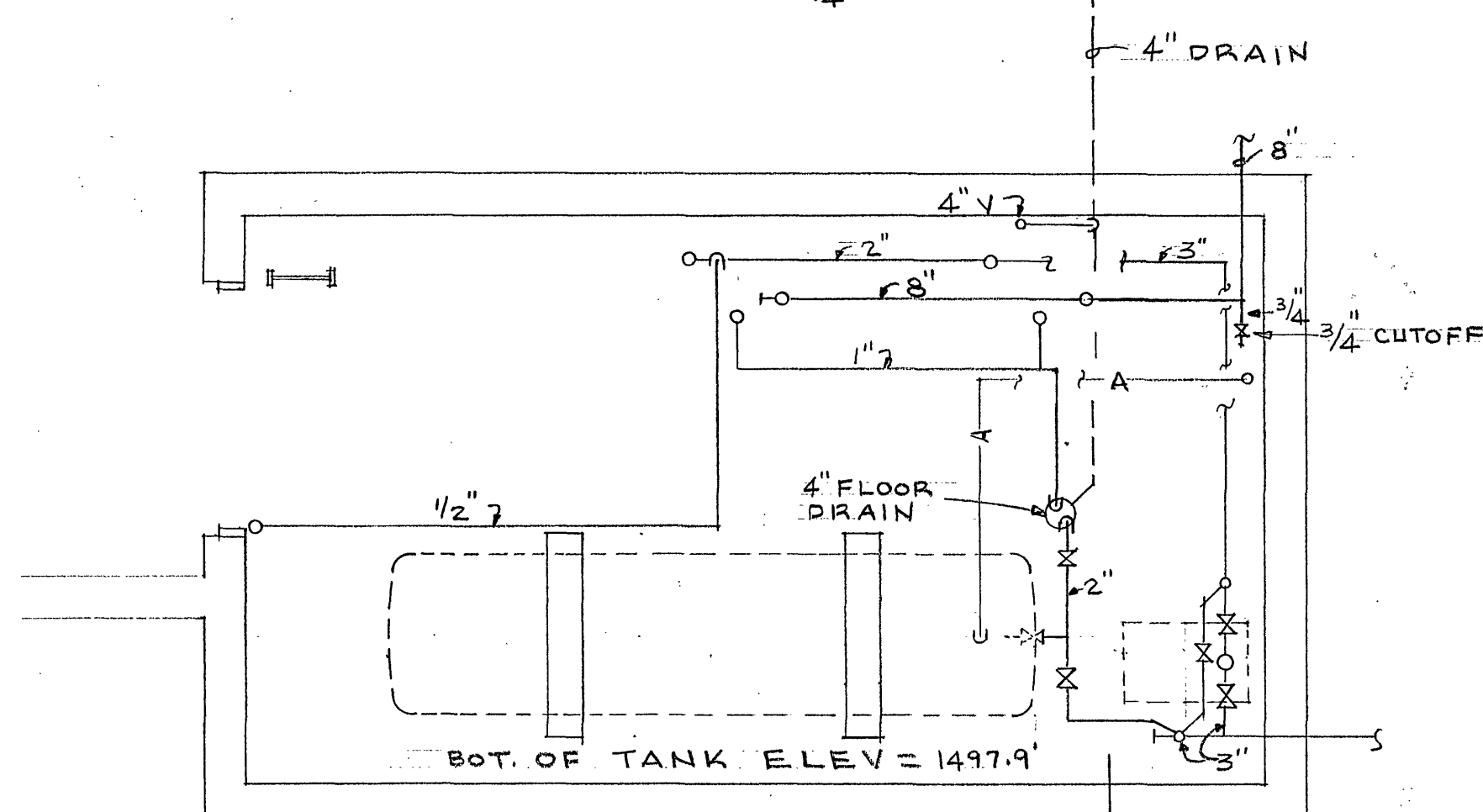
PLUMBING GROUND FLOOR PLAN SCALE: 1/4" = 1'-0"
