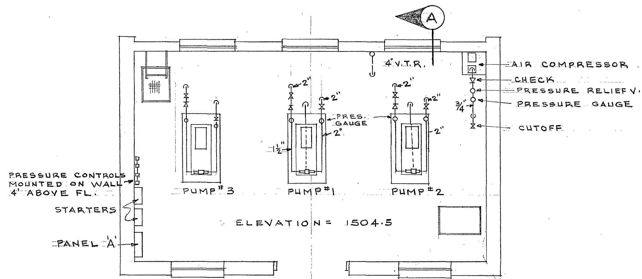
PLUMBING FIRST FLOOR PLAN SCALE: 1/4" = 1'-0"
