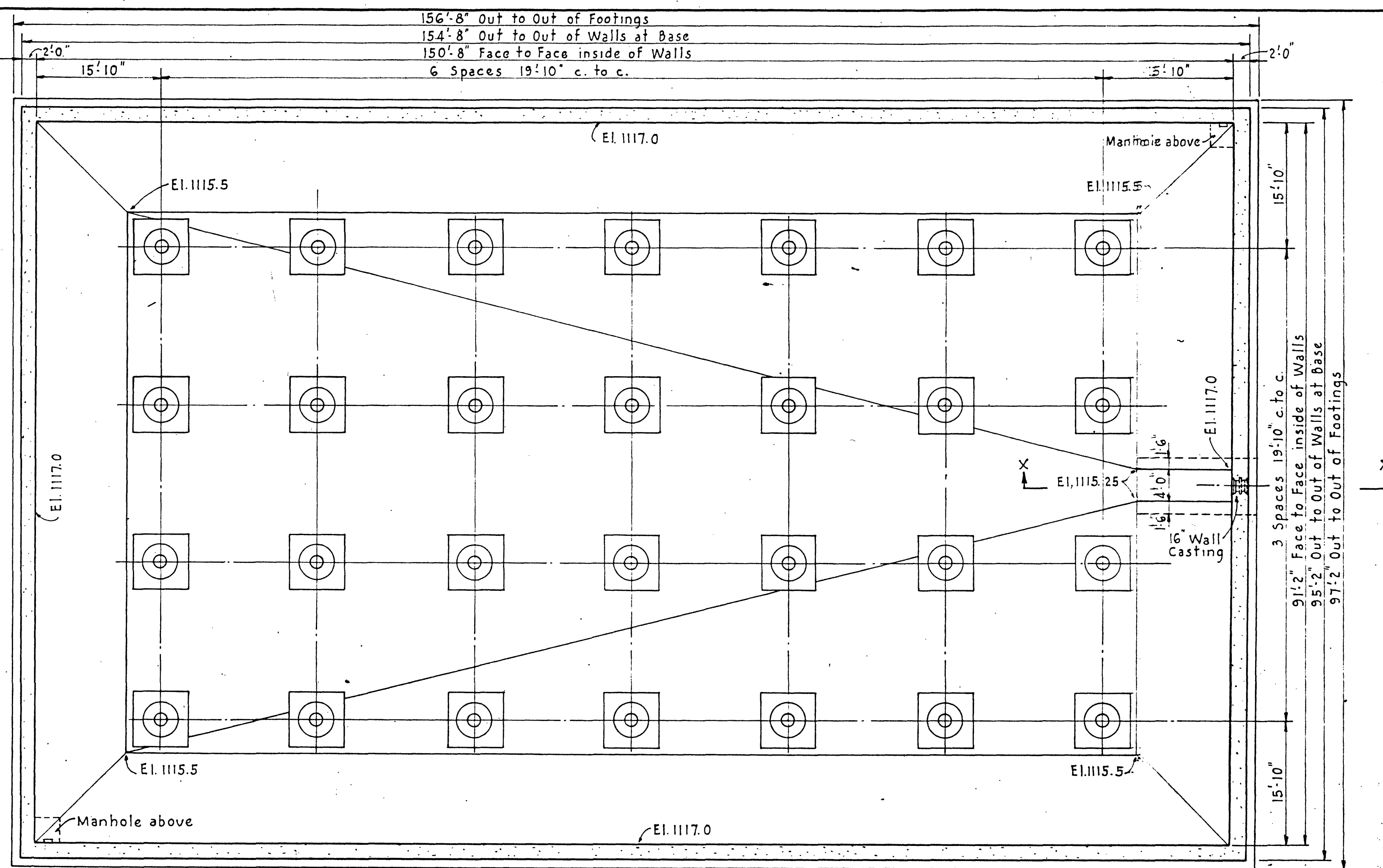
GENERAL PLAN OF 2 M.G. RESERVOIR Scale: 1" = 10' 0"
