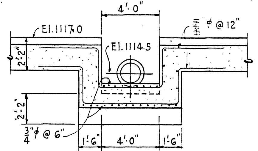
SECTION Y-Y Scale 1/4" = 1' 0"
