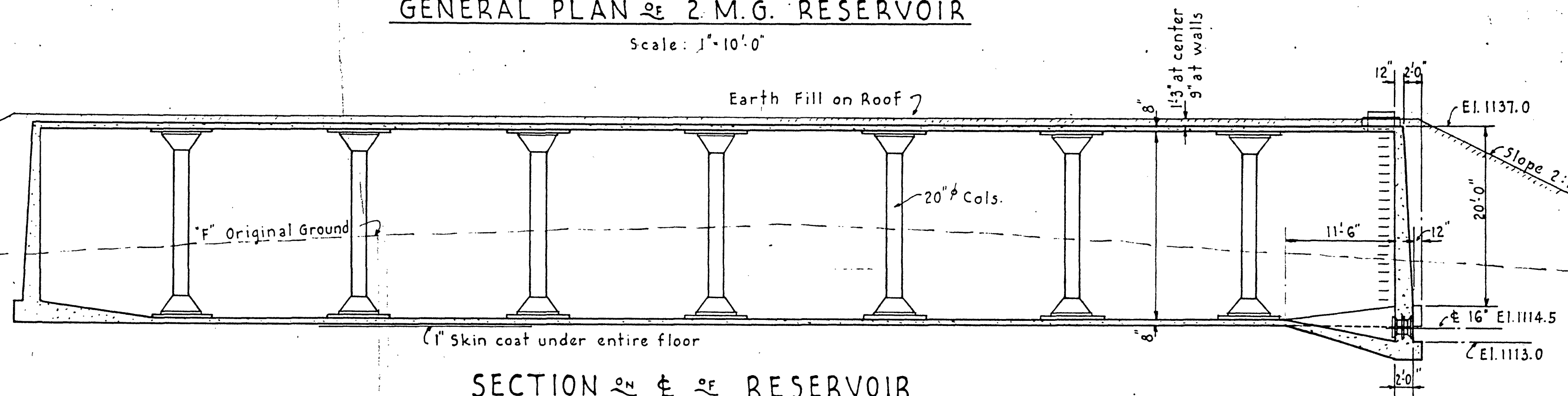
SECTION A-A OF RESERVOIR Scale: 1" = 10' 0"
