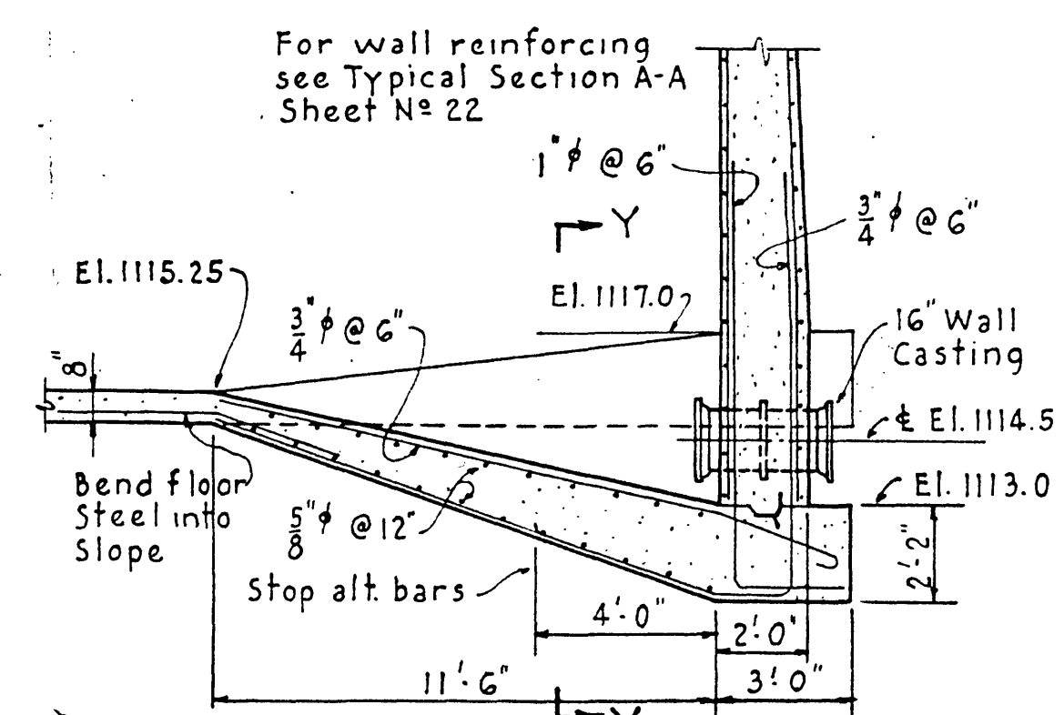
SECTION X-X Scale 1/4" = 1' 0"
