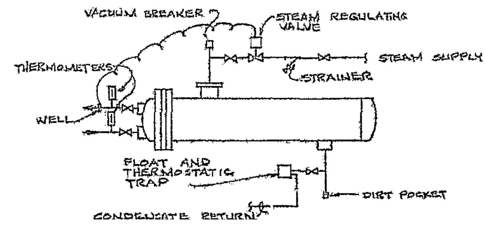
CONVERTER CONNECTION DETAIL SCHEMATIC
