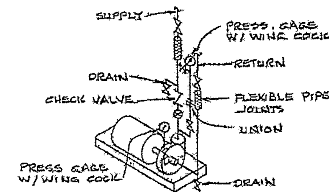
PUMP CONNECTION DETAIL SCHEMATIC
