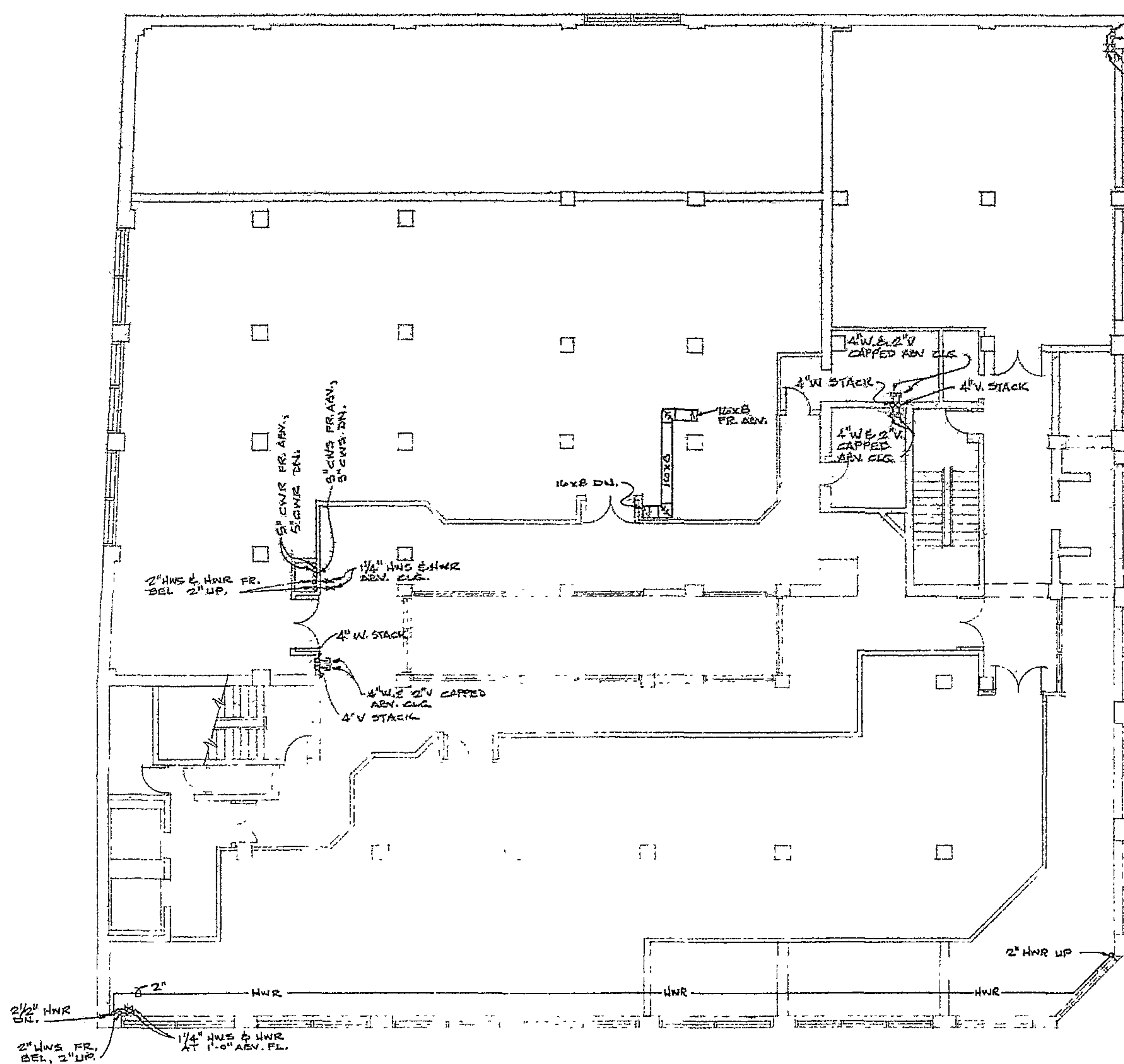
SECOND FLOOR PLAN SCALE: 1/8" = 1'-0"
