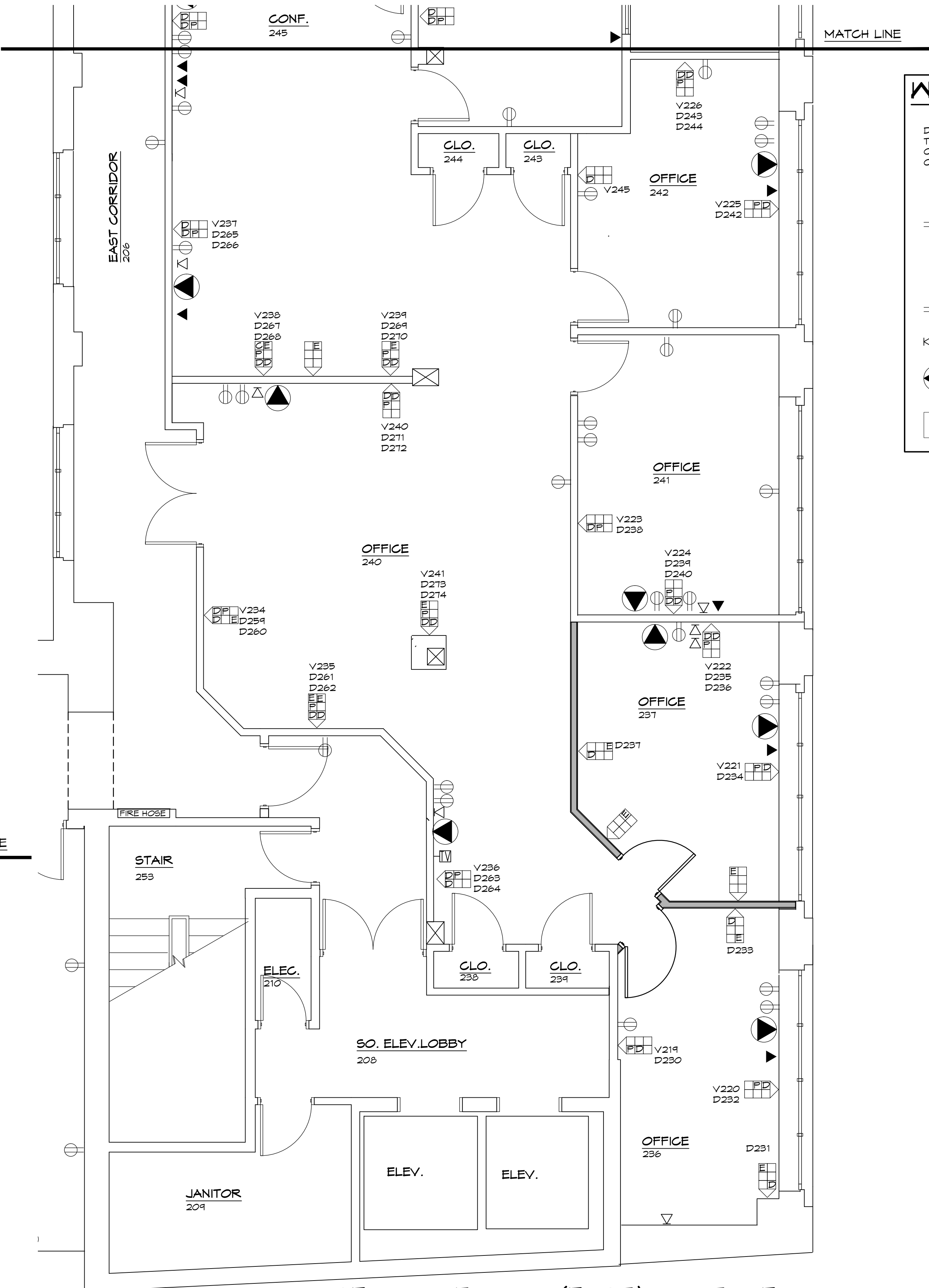
SECOND FLOOR (EAST) CONTINUED E1-5.1 E1-5 SCALE: 1/4" = 1'-0"
