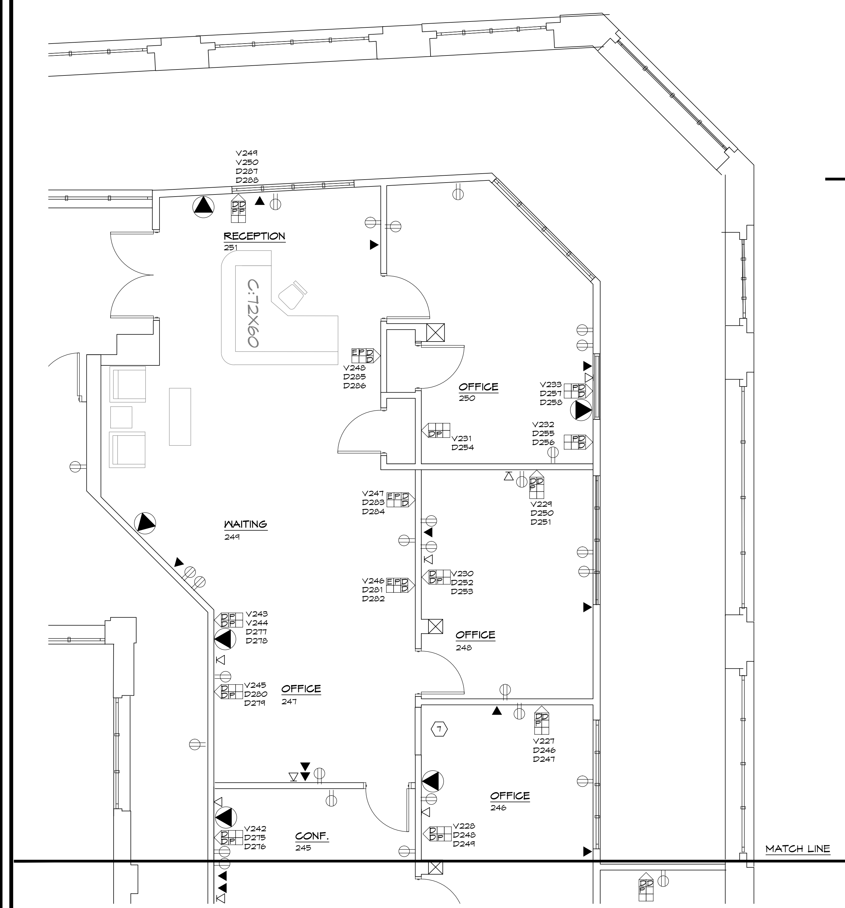
SECOND FLOOR (EAST) E1-5.1 E1-5 SCALE: 1/4" = 1'-0"
