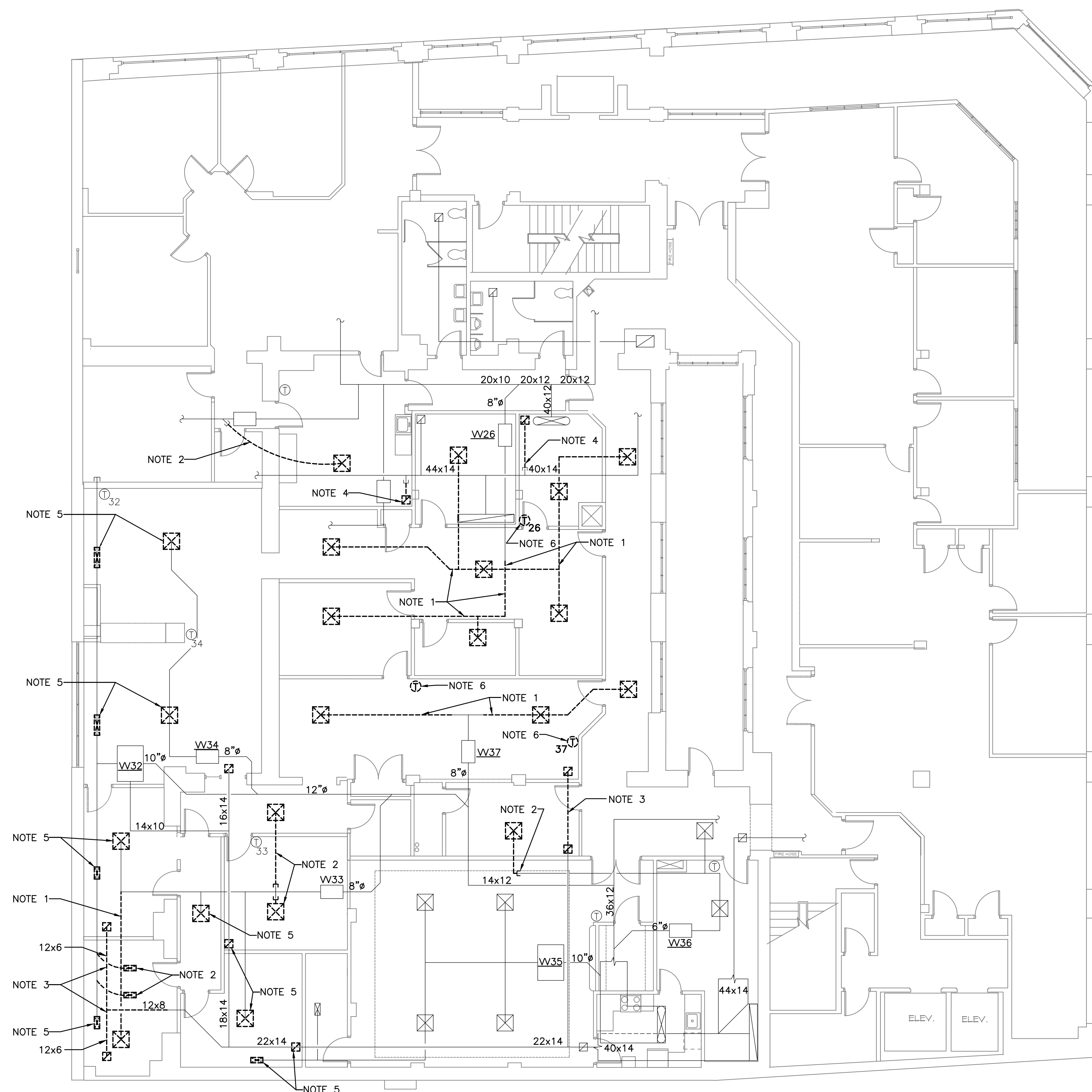
SECOND FLOOR PLAN - DEMOLITION
