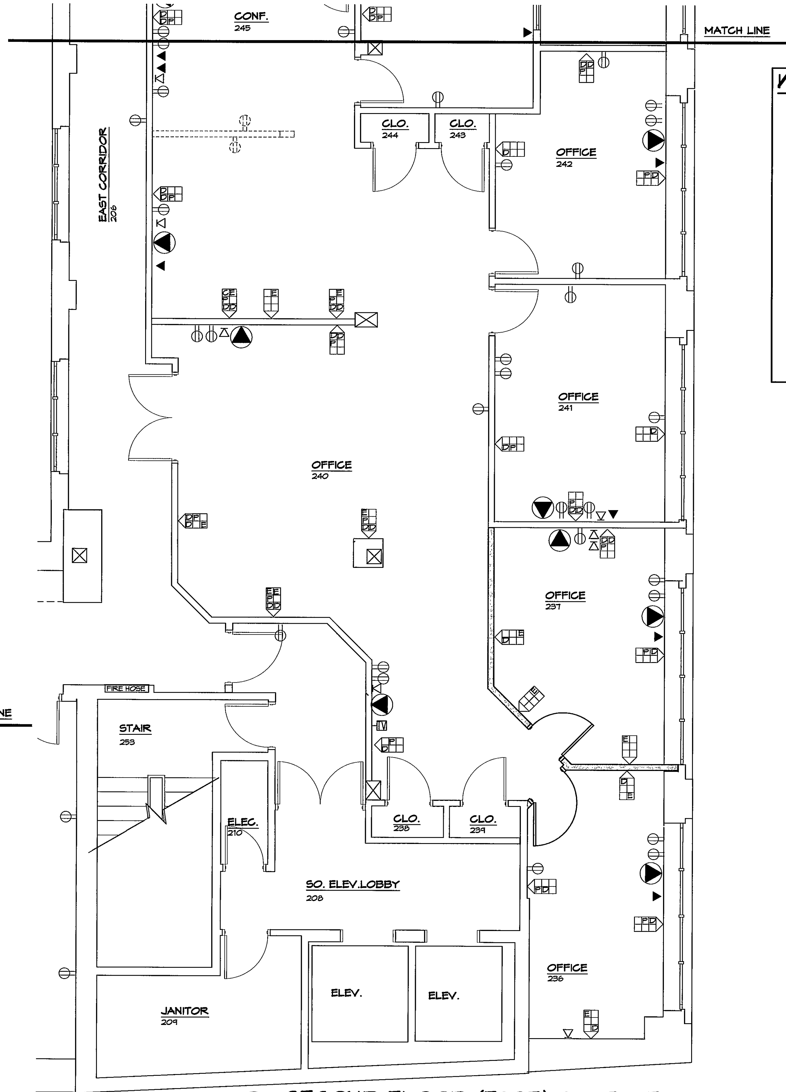
E1-5.1 E1-3 SECOND FLOOR (EAST) CONTINUED SCALE: 1/4" = 1'-0"
