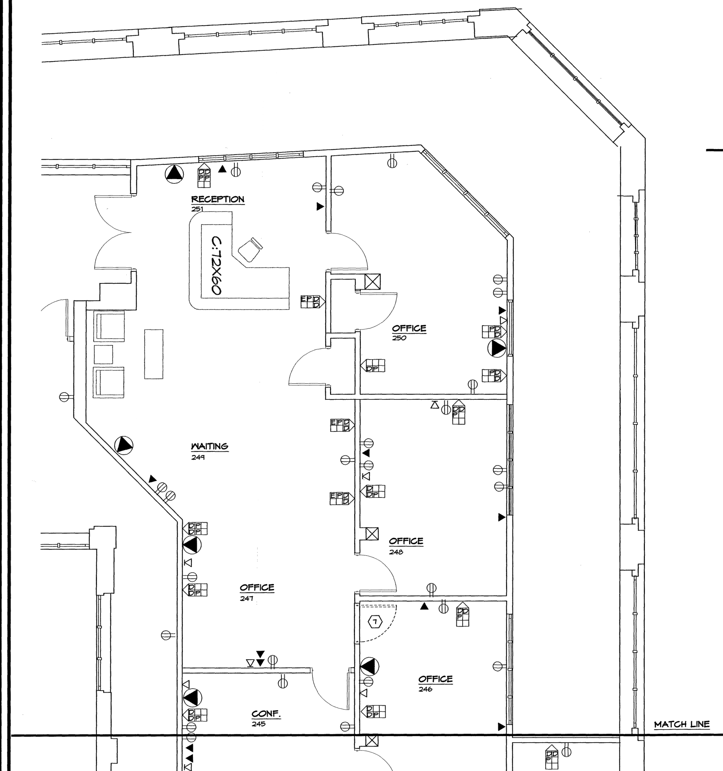
SECOND FLOOR (EAST) E1-5.1 E1-3 SCALE: 1/4" = 1'-0"
