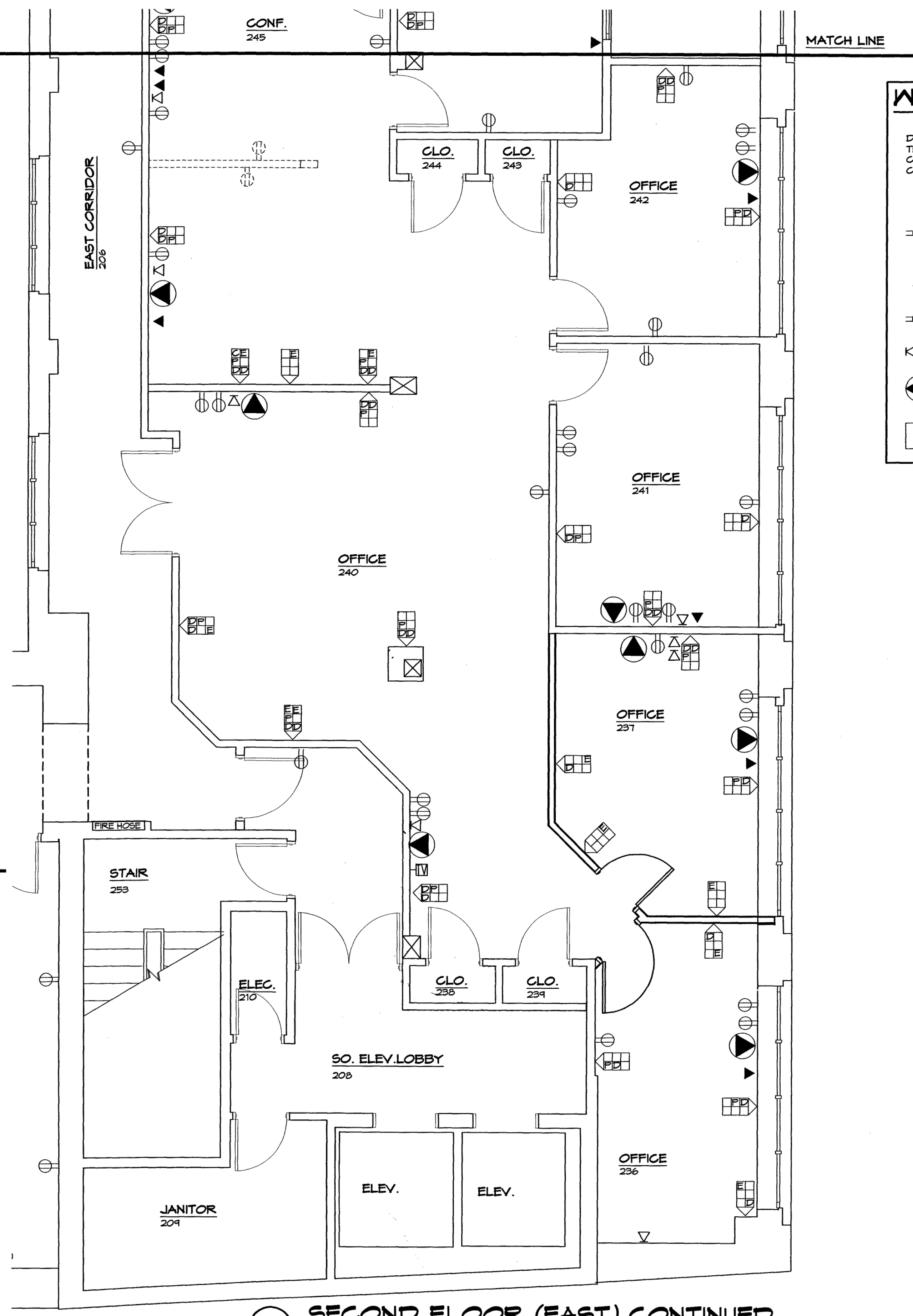
SECOND FLOOR (EAST) CONTINUED E1-5.1 E1-3 SCALE: 1/4" = 1'-0"
