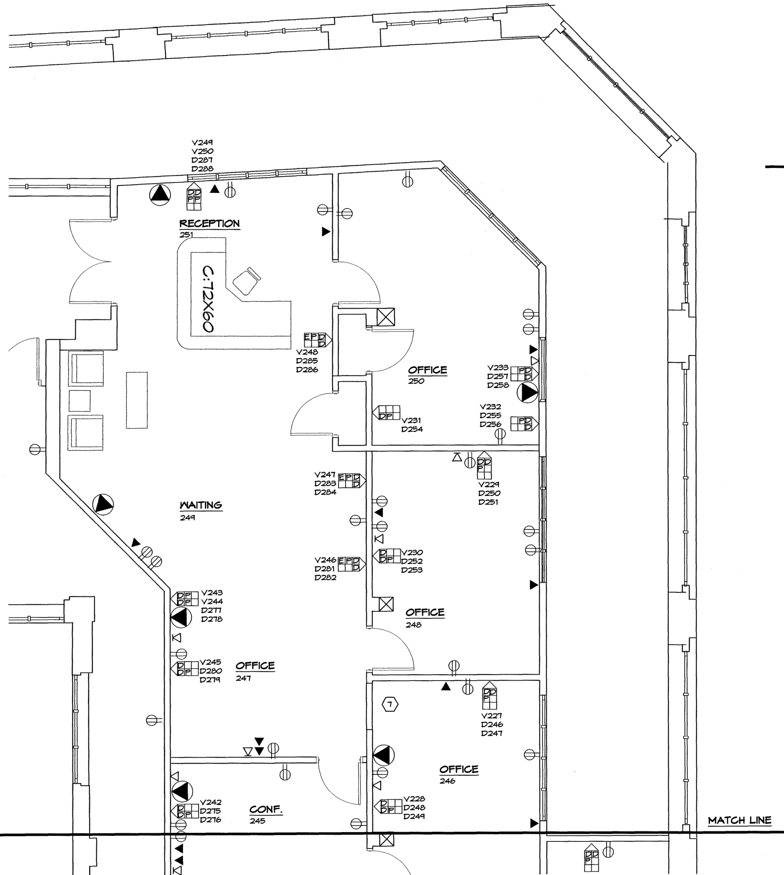
SECOND FLOOR (EAST) SCALE: 1/4" = 1'-0"
