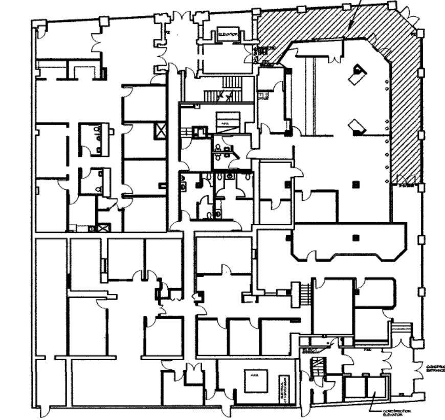
EXISTING SPRINKLERED FLOOR AREA
