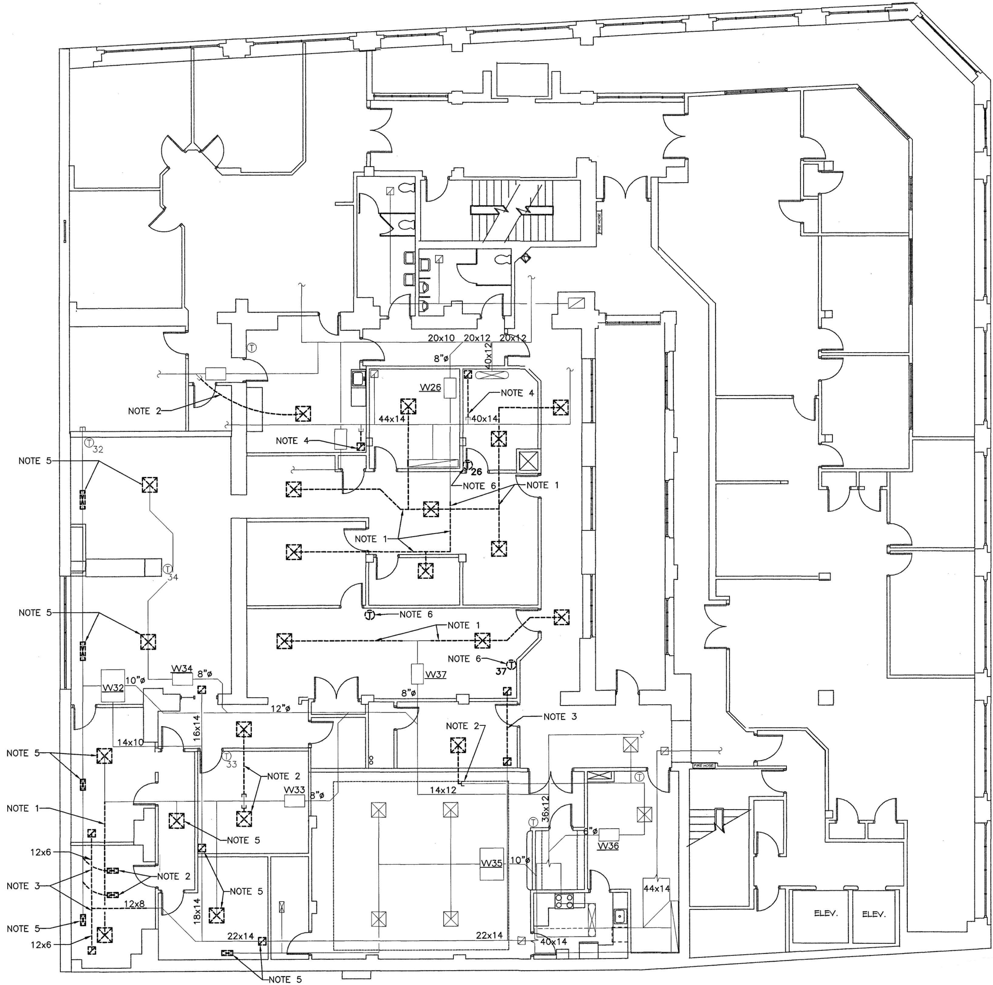
SECOND FLOOR PLAN - DEMOLITION SCALE: 1/8" = 1'-0"
