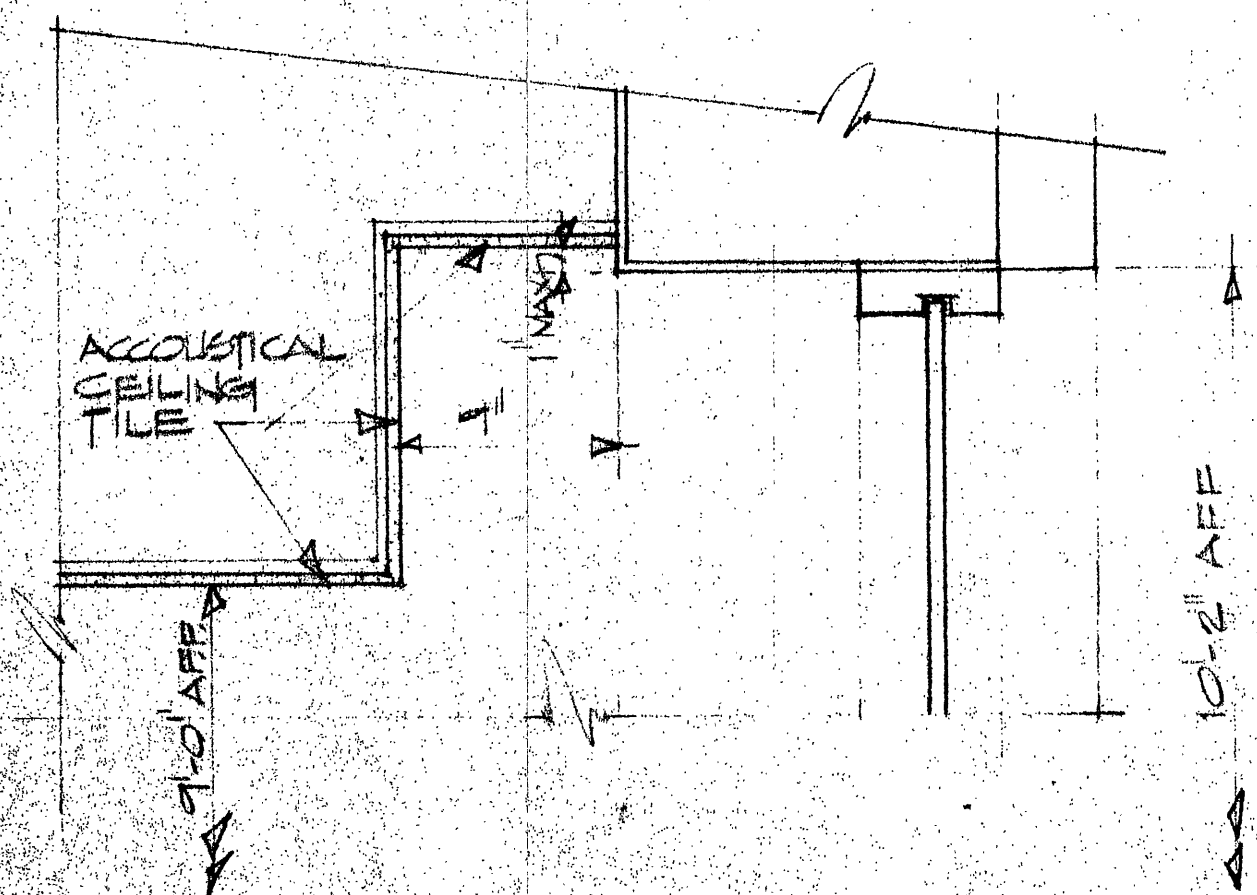
DETAIL - DROPPED CUR @ EXT. WALL 1/2" = 1'-0"
