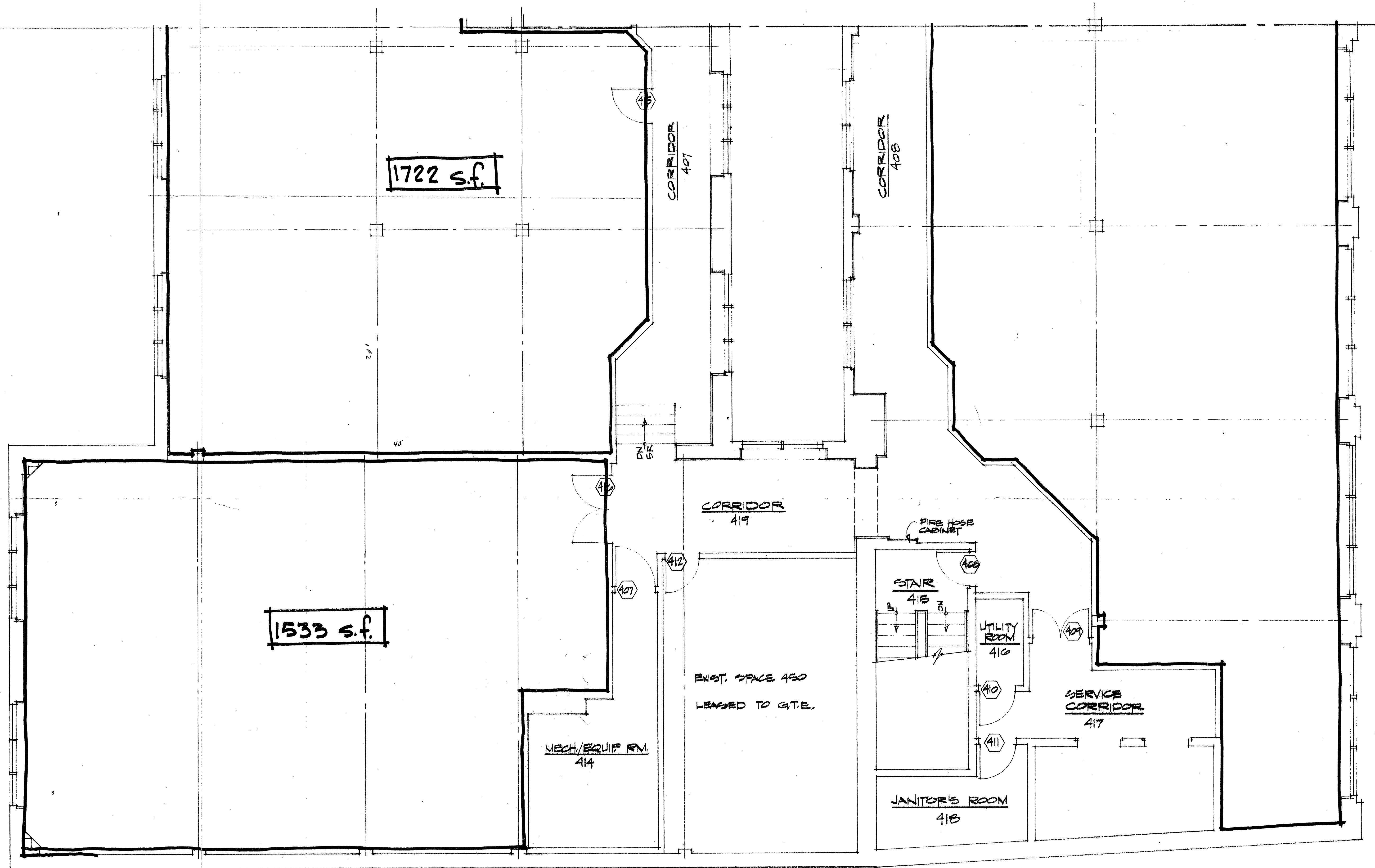
FOURTH FLOOR PLAN - SOUTH 1/4" = 1'-0"
