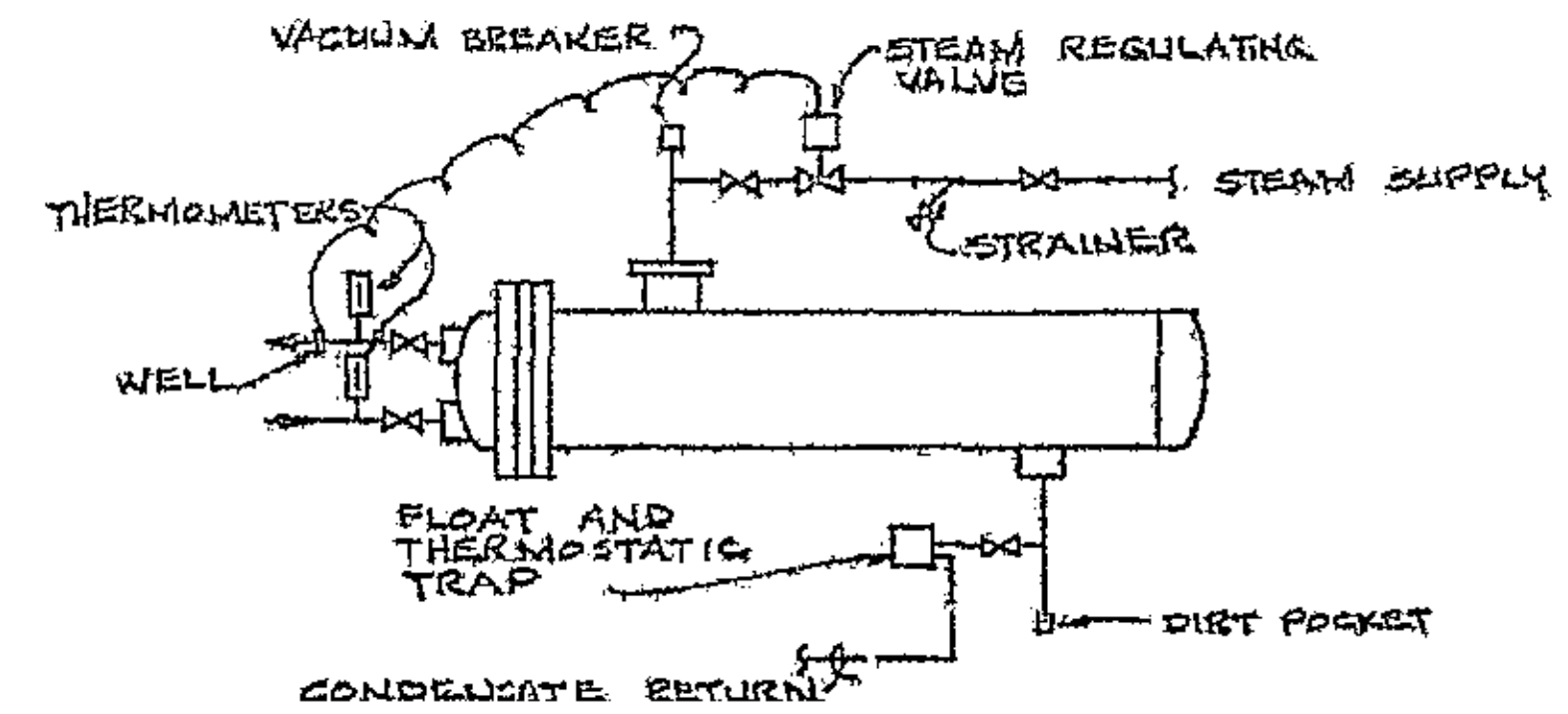
CONVERTER CONNECTION DETAIL SCHEMATIC
