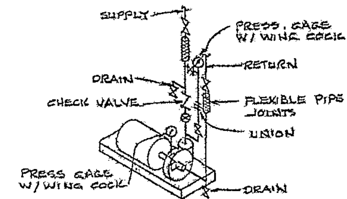
PUMP CONNECTION DETAIL SCHEMATIC
