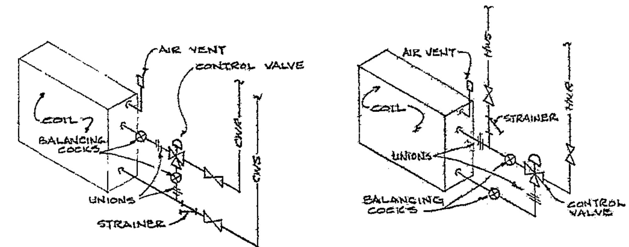
COIL CONNECTION DETAILS SCHEMATIC
