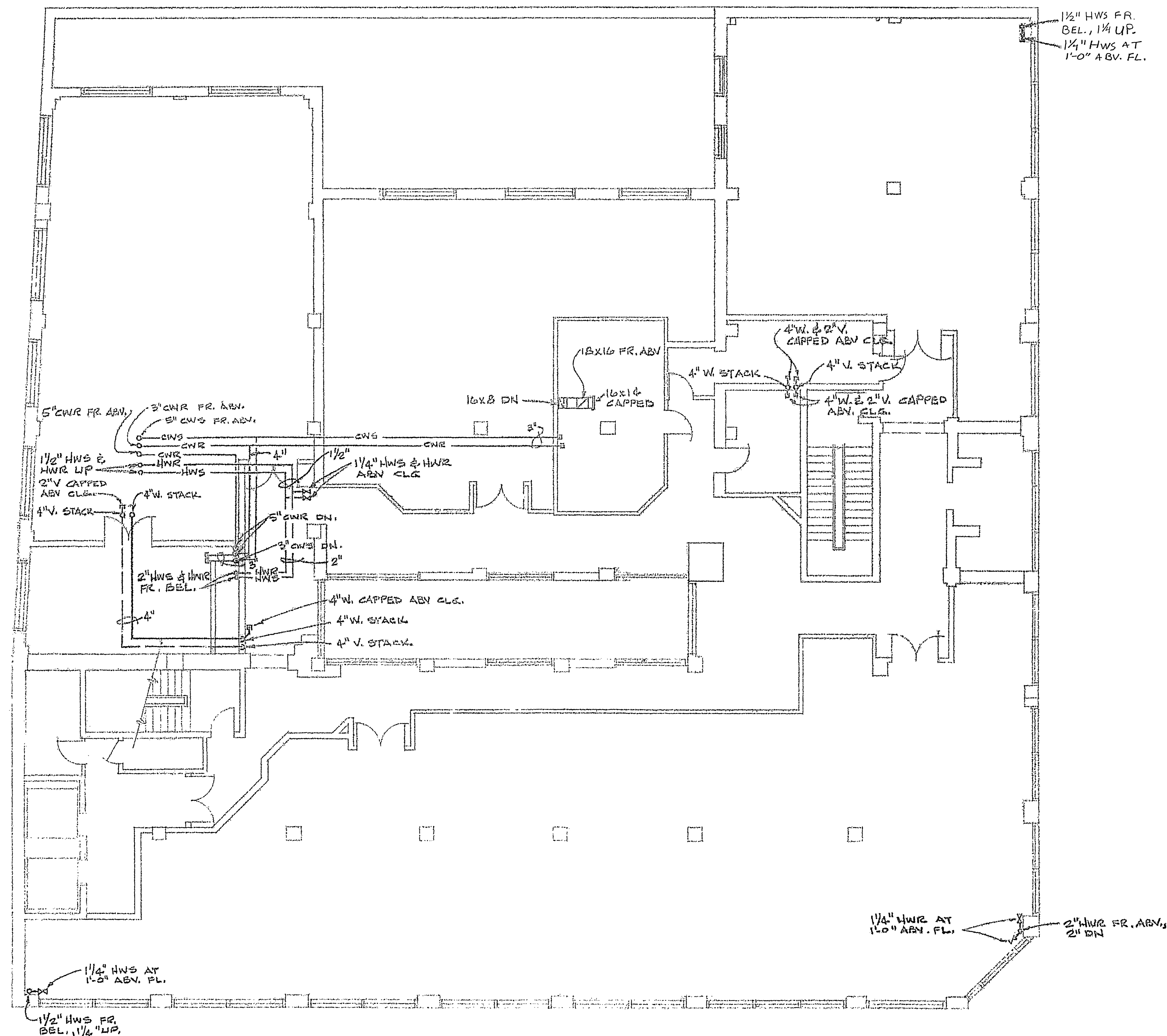
THIRD FLOOR PLAN SCALE: 1/8" = 1'-0"
