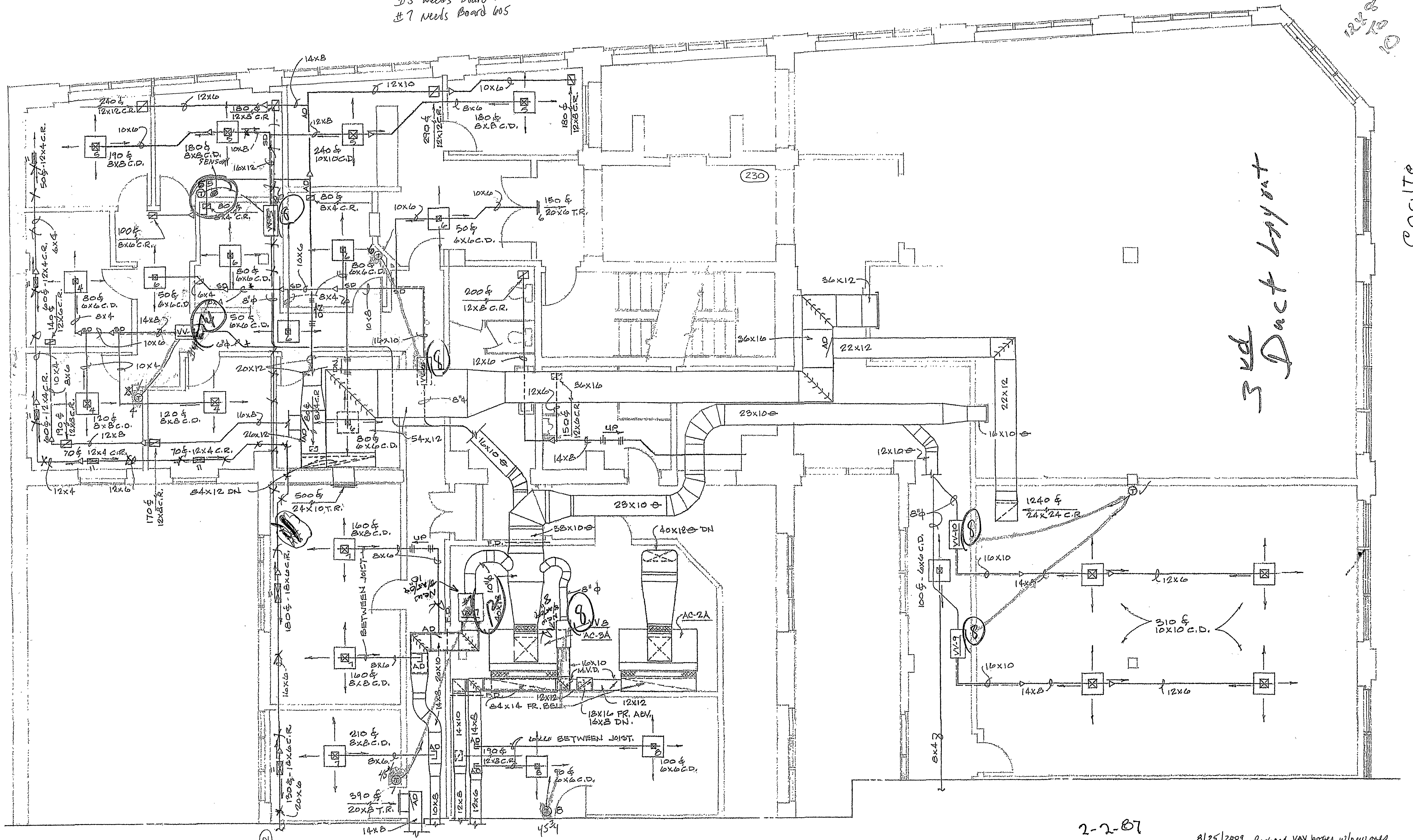
THIRD FLOOR PLAN - NORTH SCALE: 1/4" = 1'-0"
