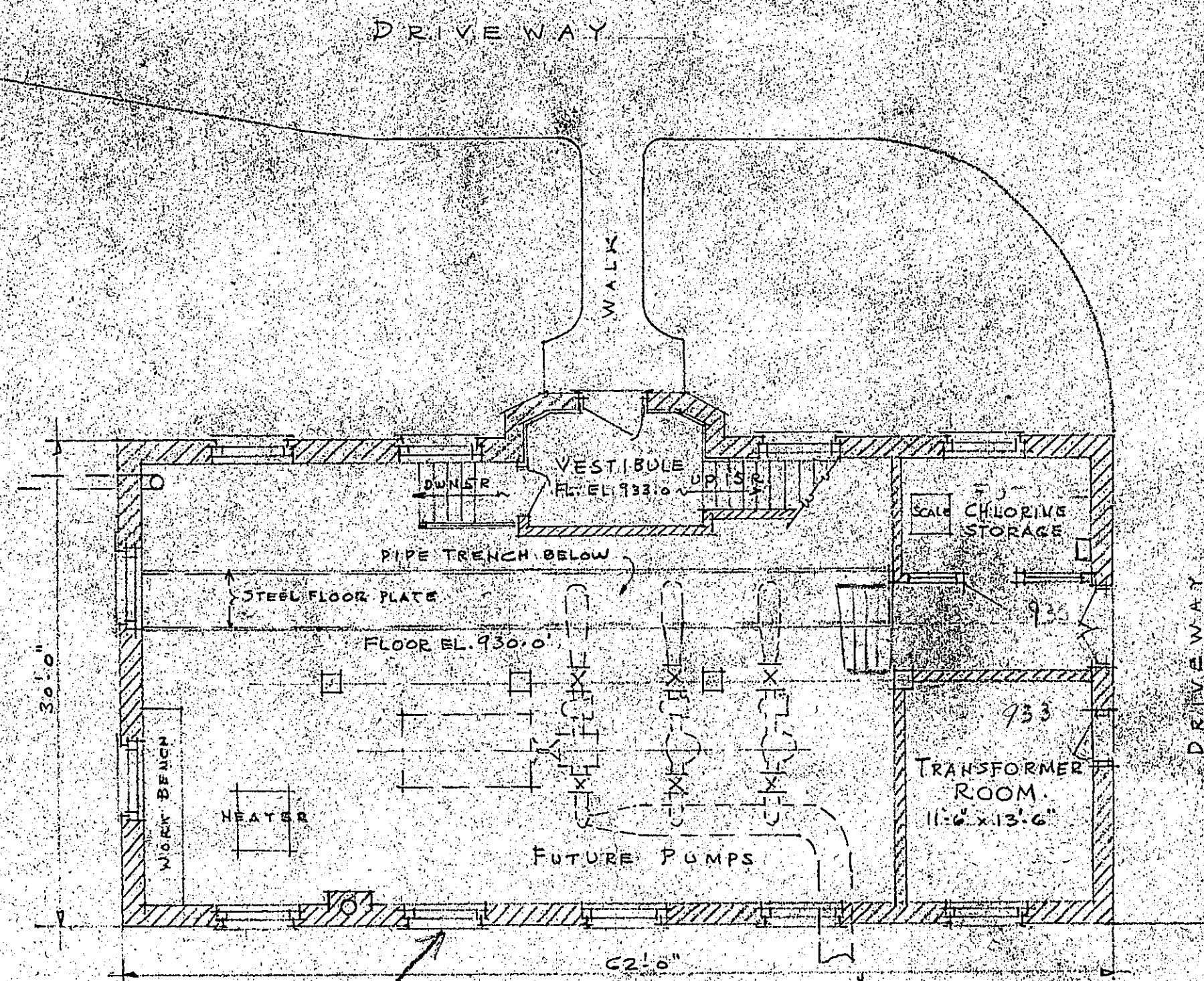
MAIN FLOOR PLAN SCALE 1/8" = 1'-0"
