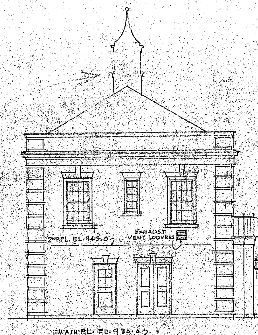
EAST ELEVATION SCALE 1/8" = 1'-0"
