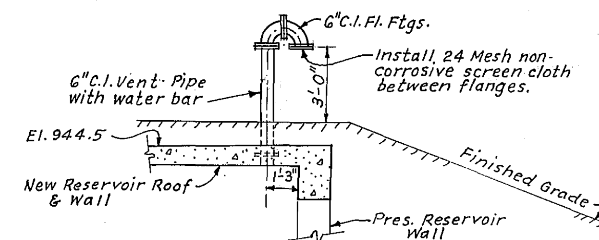
DETAIL OF VENT Scale: 1/4" = 1'-0"
