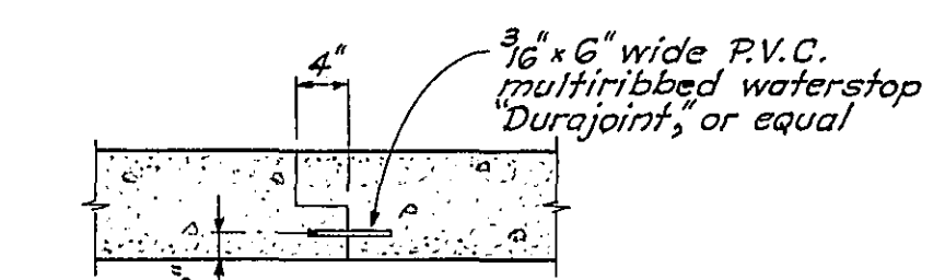
SLAB CONSTR. JOINT Scale: 3/4" = 1'-0"
