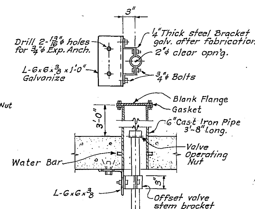
DETAIL OF VALVE STEM BRACKET Scale: 1" = 1'-0"
