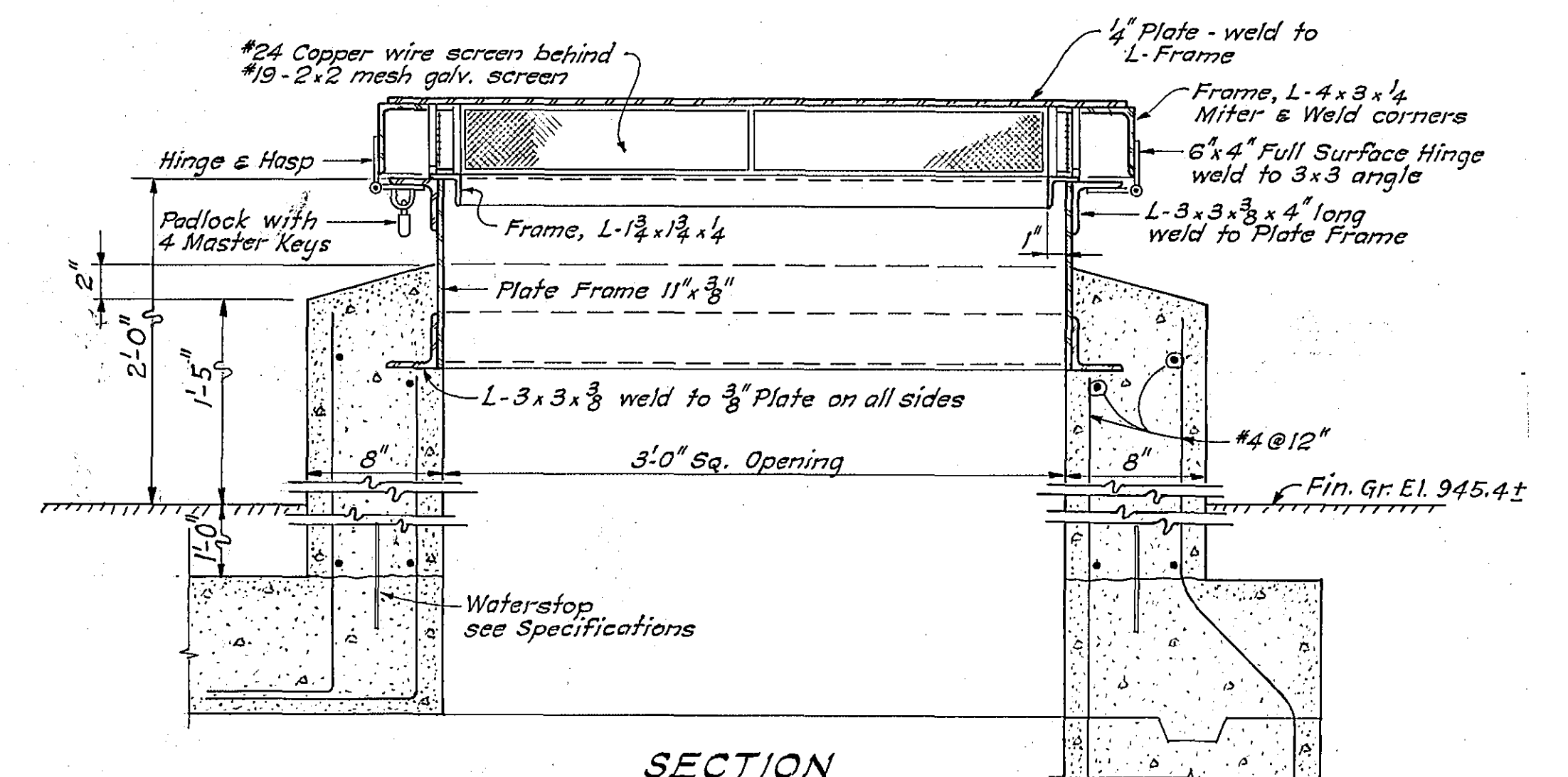
SECTION DETAILS OF MANHOLE FRAME & COVER Scale: 1/2" = 1'-0"
