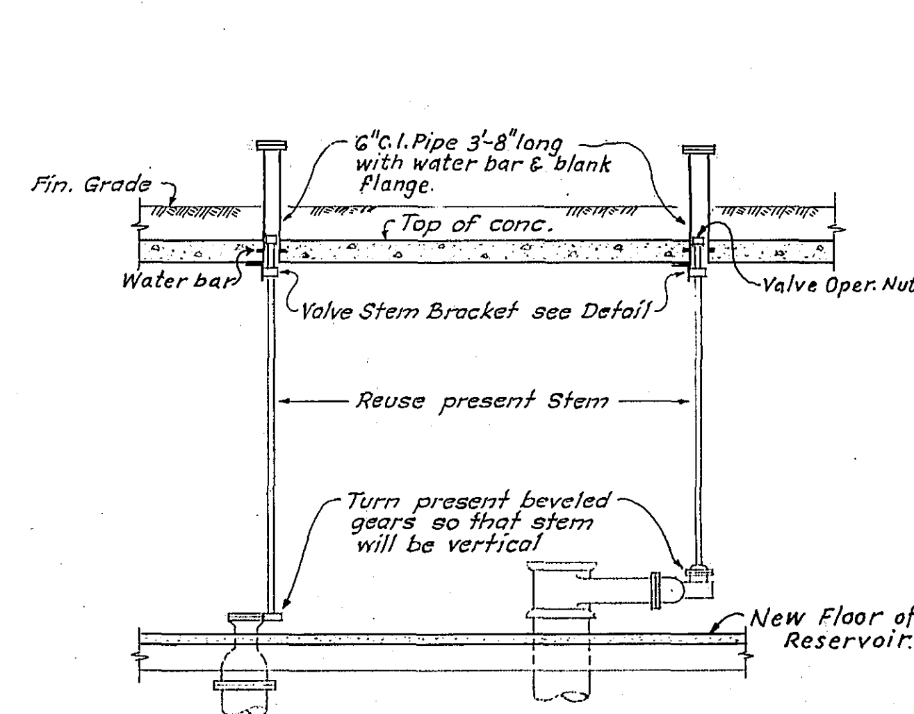
DETAIL OF VALVE EXTENSION PIPE & STEM Scale: 1/4" = 1'-0"
