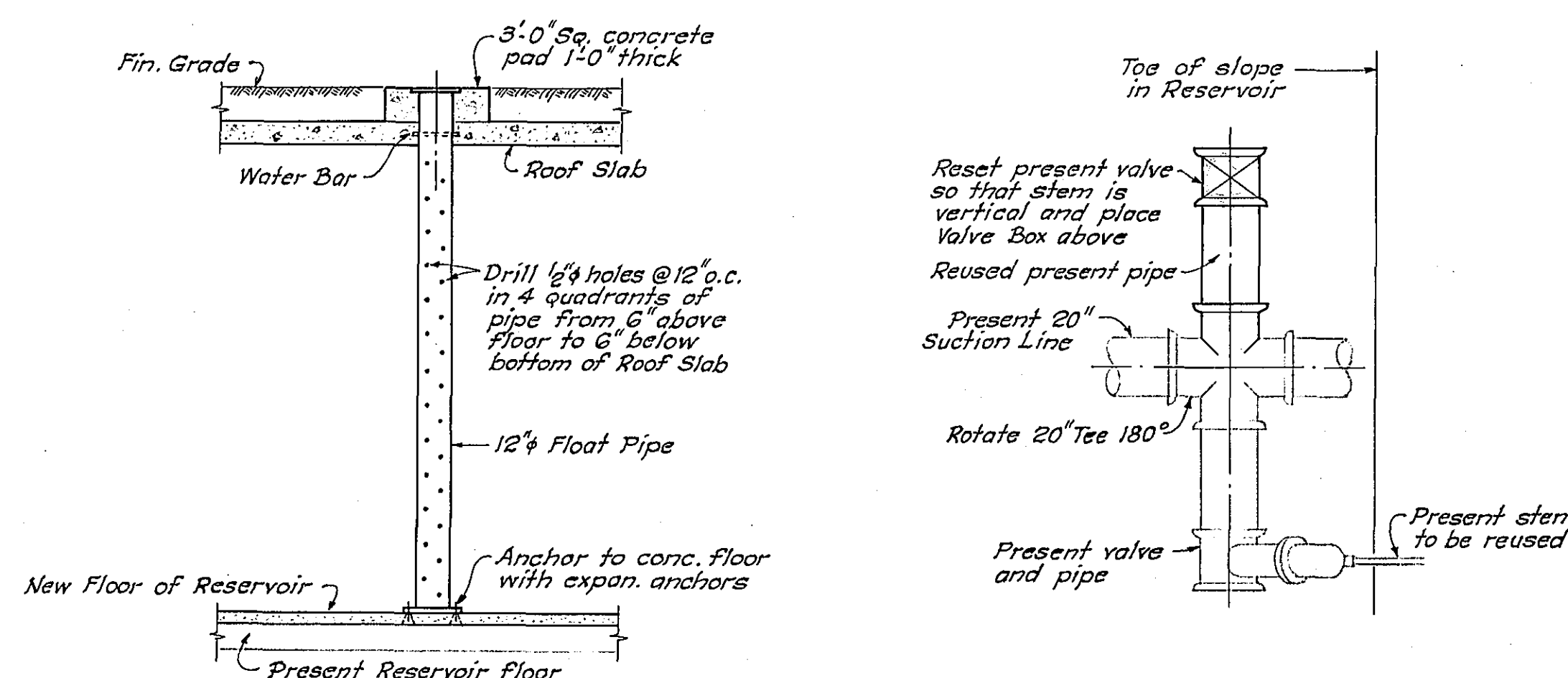
DETAIL OF FLOAT PIPE Scale: 1/4" = 1'-0"
