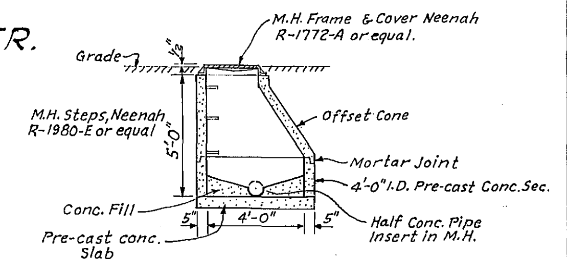
DETAIL OF MANHOLE Scale: 1/4" = 1'-0"
