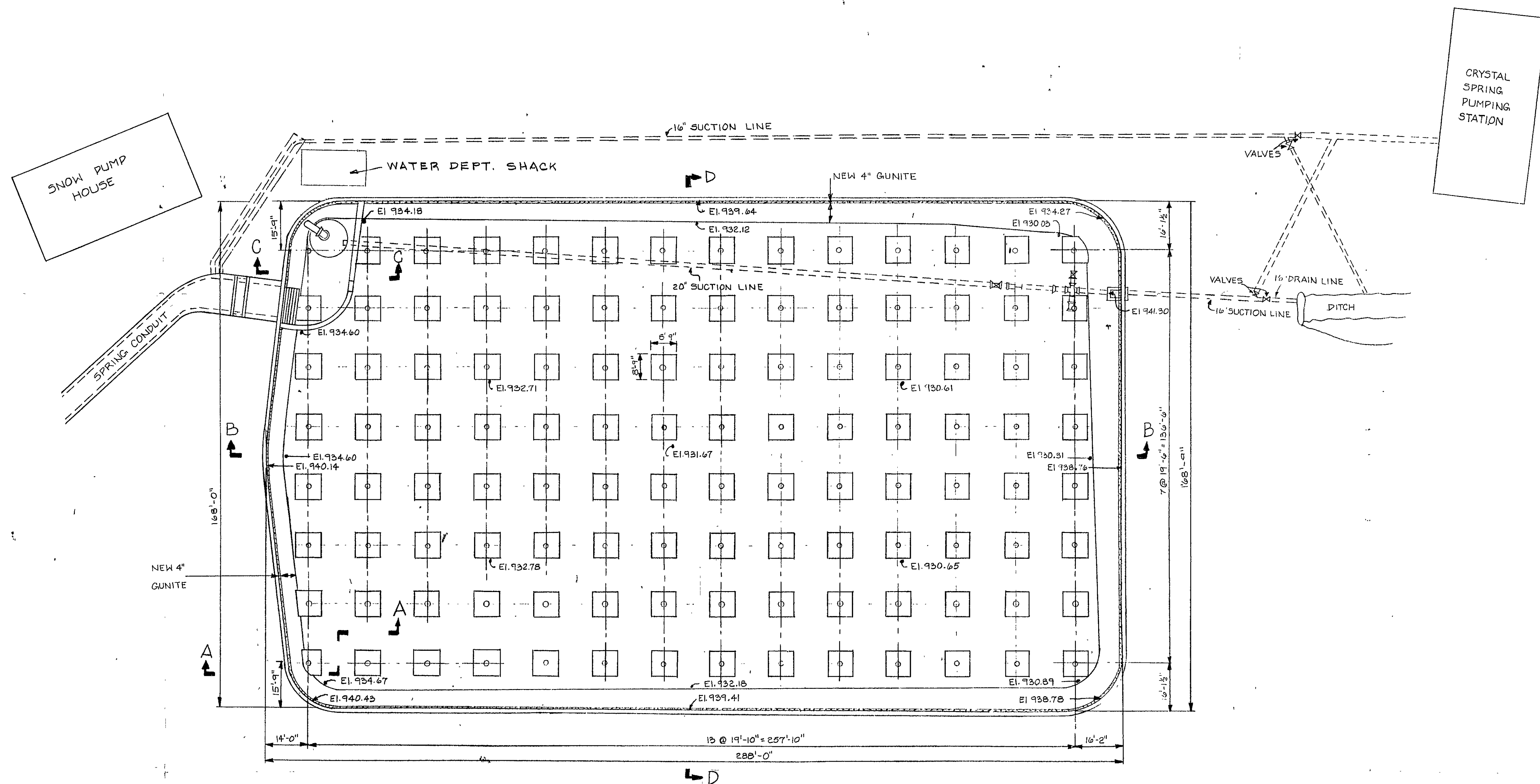
PLAN SCALE: 1"=20'-0" NEW 4" GUNITE ON VERTICAL AND SLOPING WALLS.
