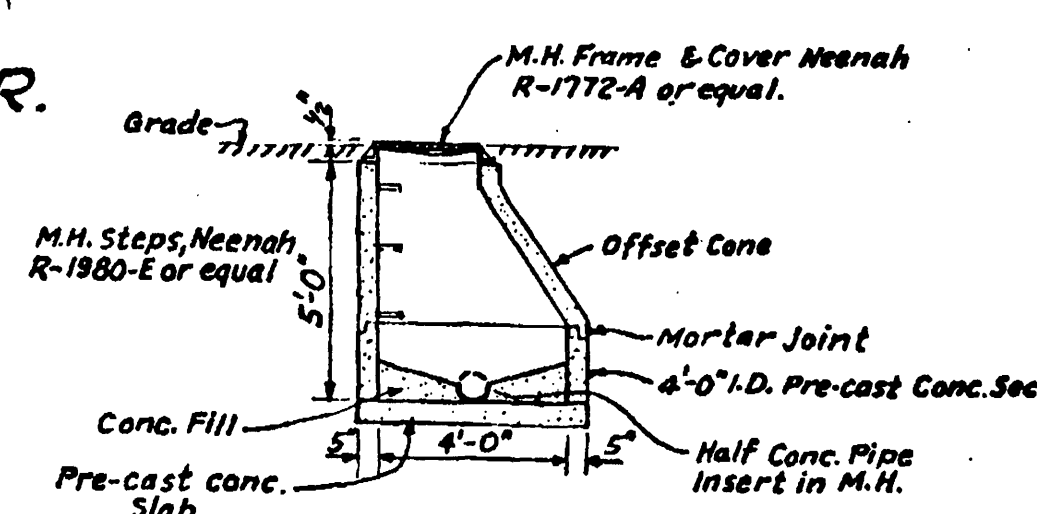
DETAIL OF MANHOLE Scale: 1/4" = 1'-0"
