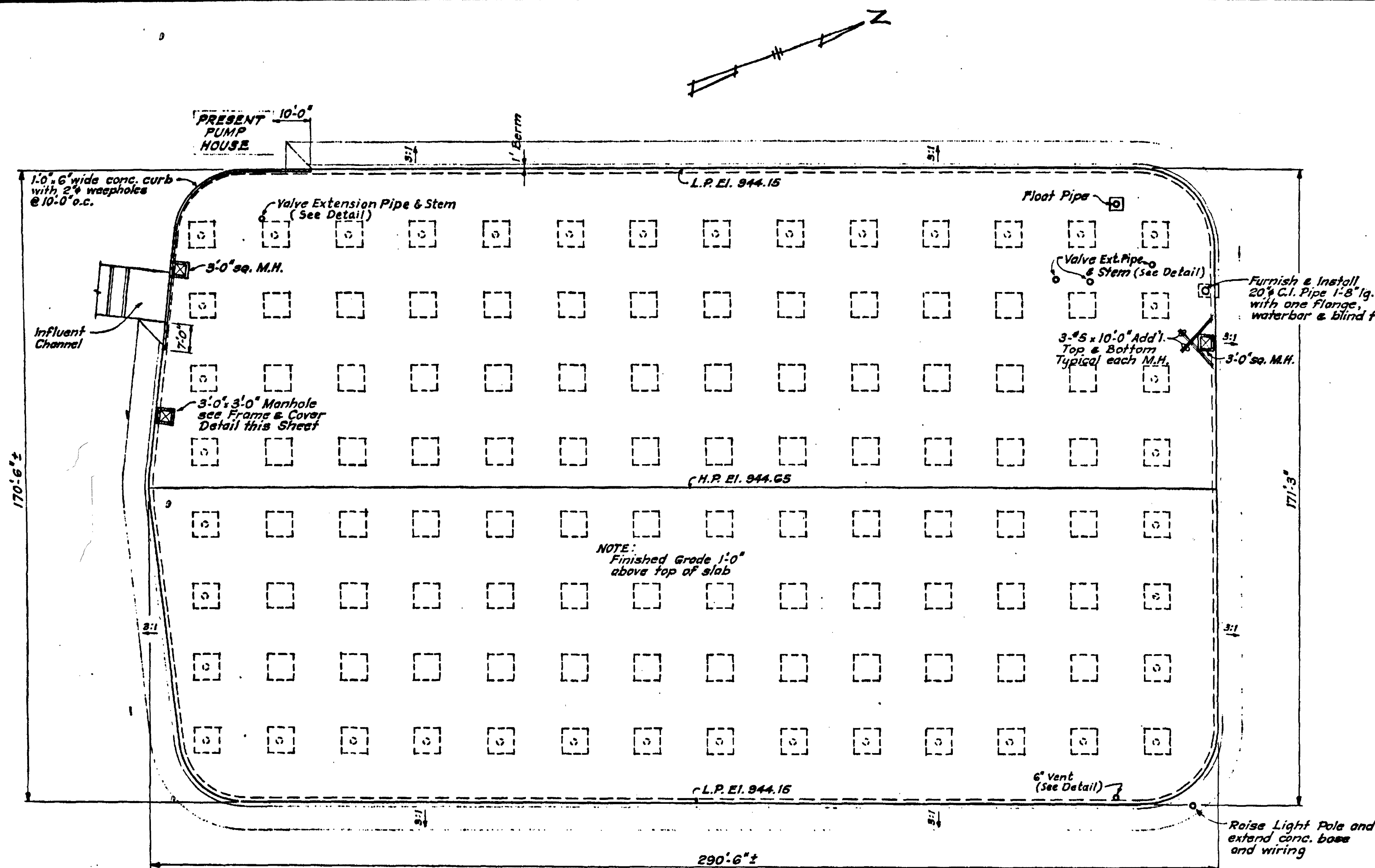
ROOF PLAN Scale: 1" = 20'
