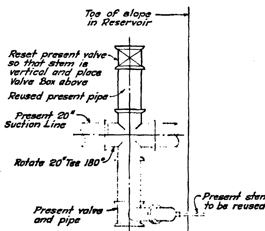
DETAIL OF RELOCATED 20" VALVE & PIPE Scale: 1/4" = 1'-0"
