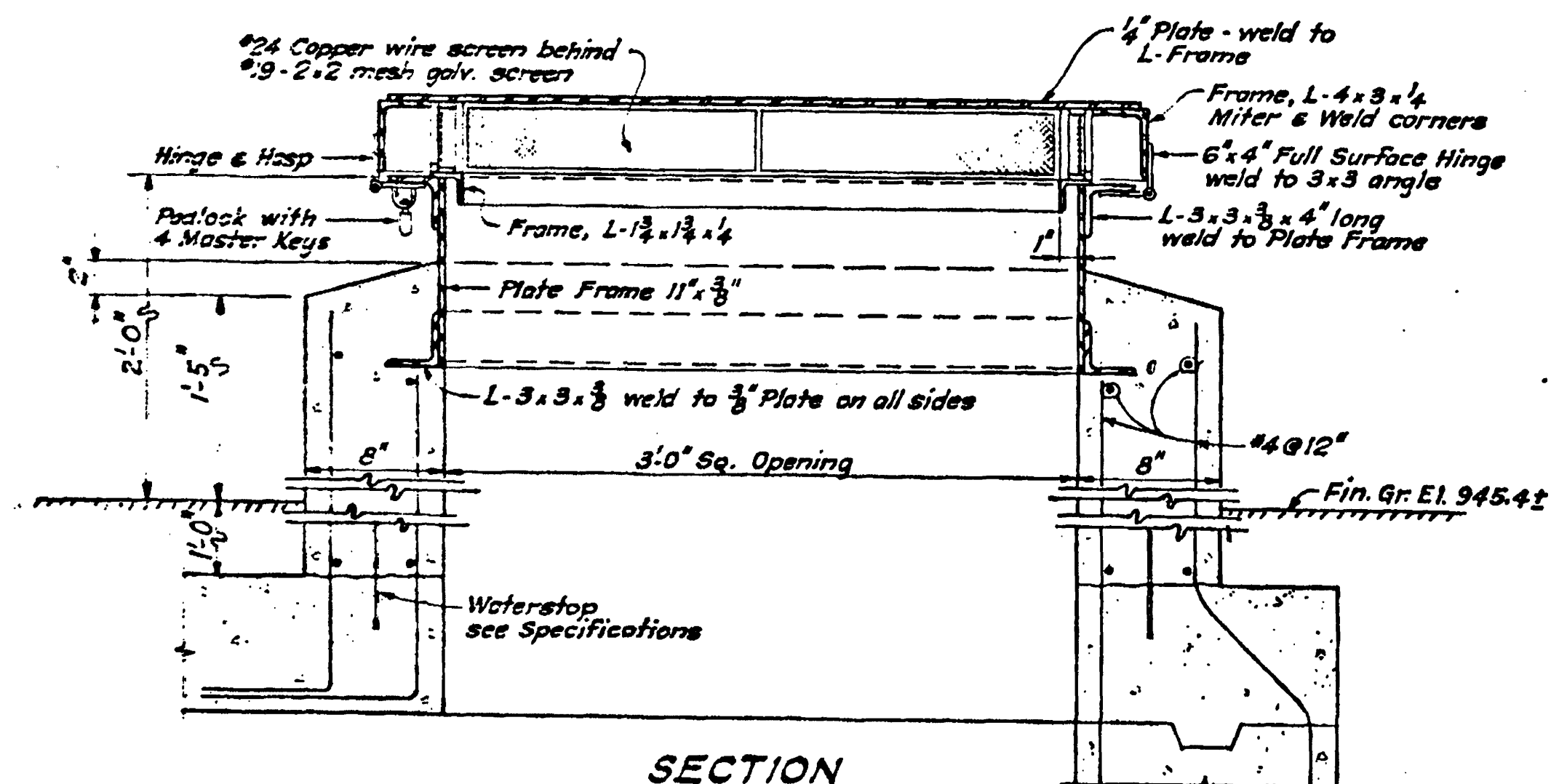
SECTION DETAILS OF MANHOLE FRAME & COVER Scale: 1/2" = 1'-0"
