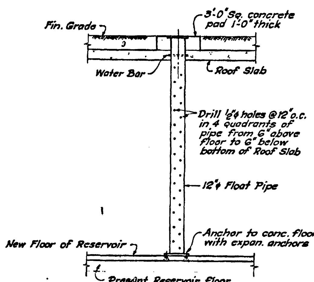
DETAIL OF FLOAT PIPE Scale: 1/4" = 1'-0"
