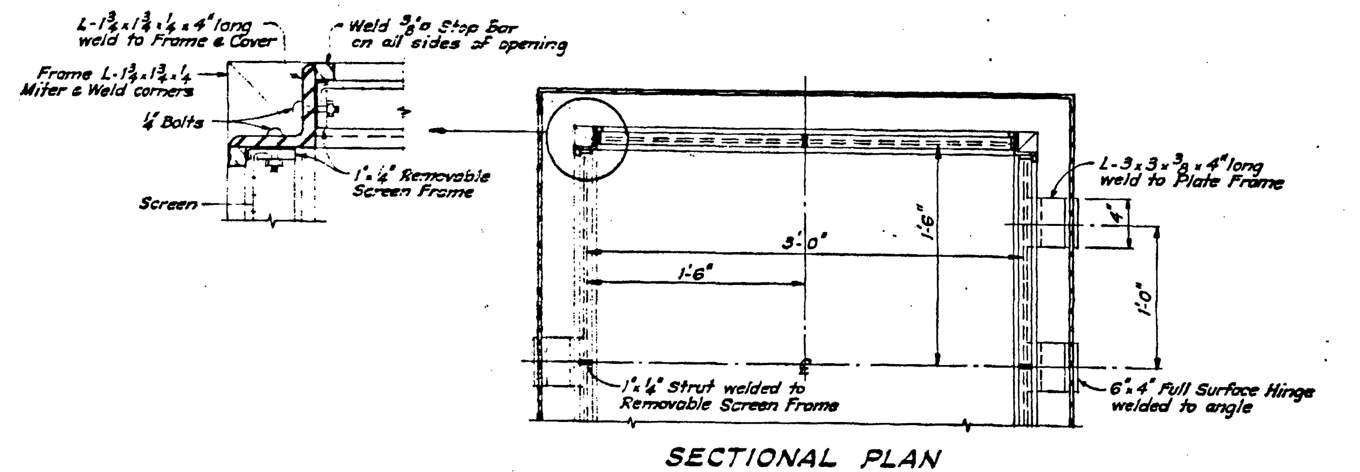
SECTIONAL PLAN
