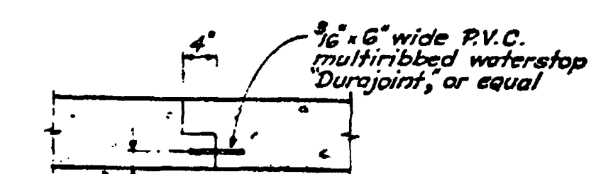
SLAB CONSTR. JOINT Scale: 3/4" = 1'-0"
