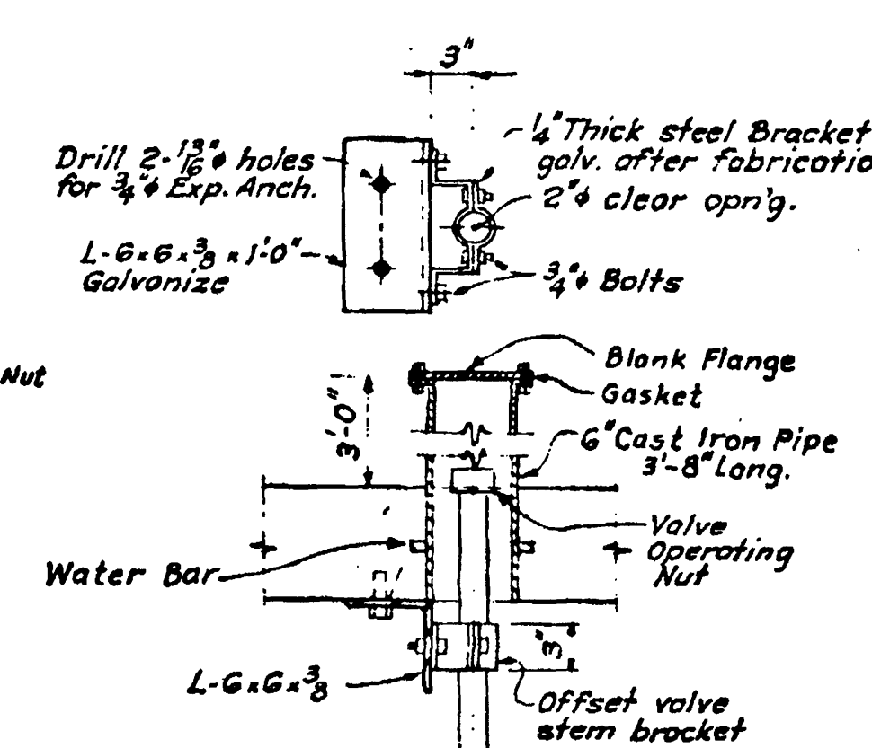
DETAIL OF VALVE STEM BRACKET Scale: 1" = 1'-0"
