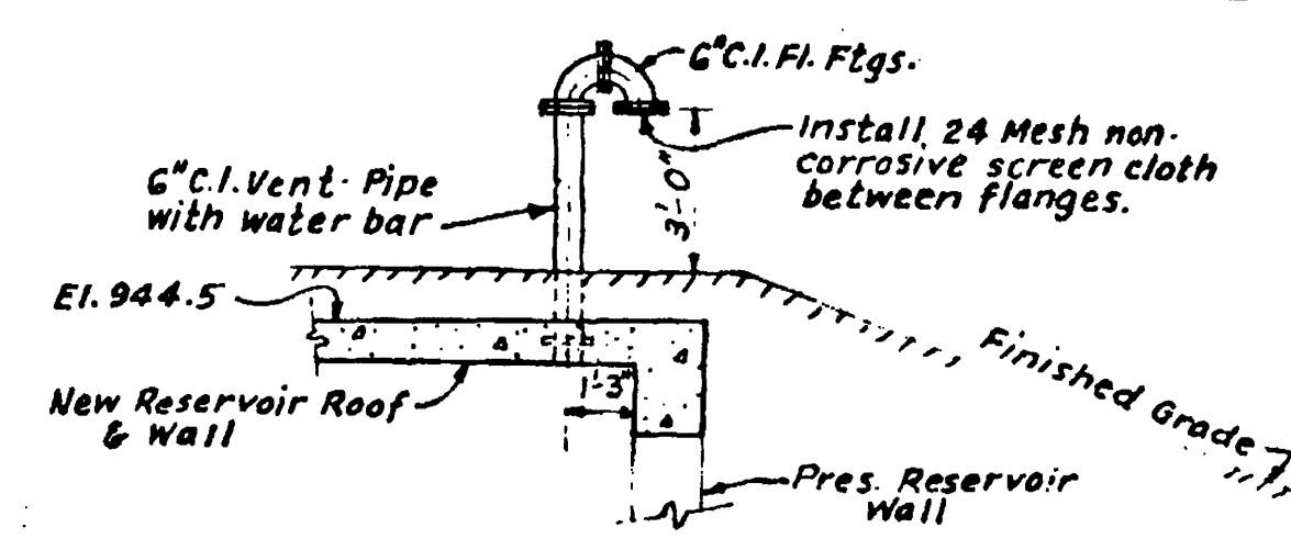
DETAIL OF VENT Scale: 1/4" = 1'-0"
