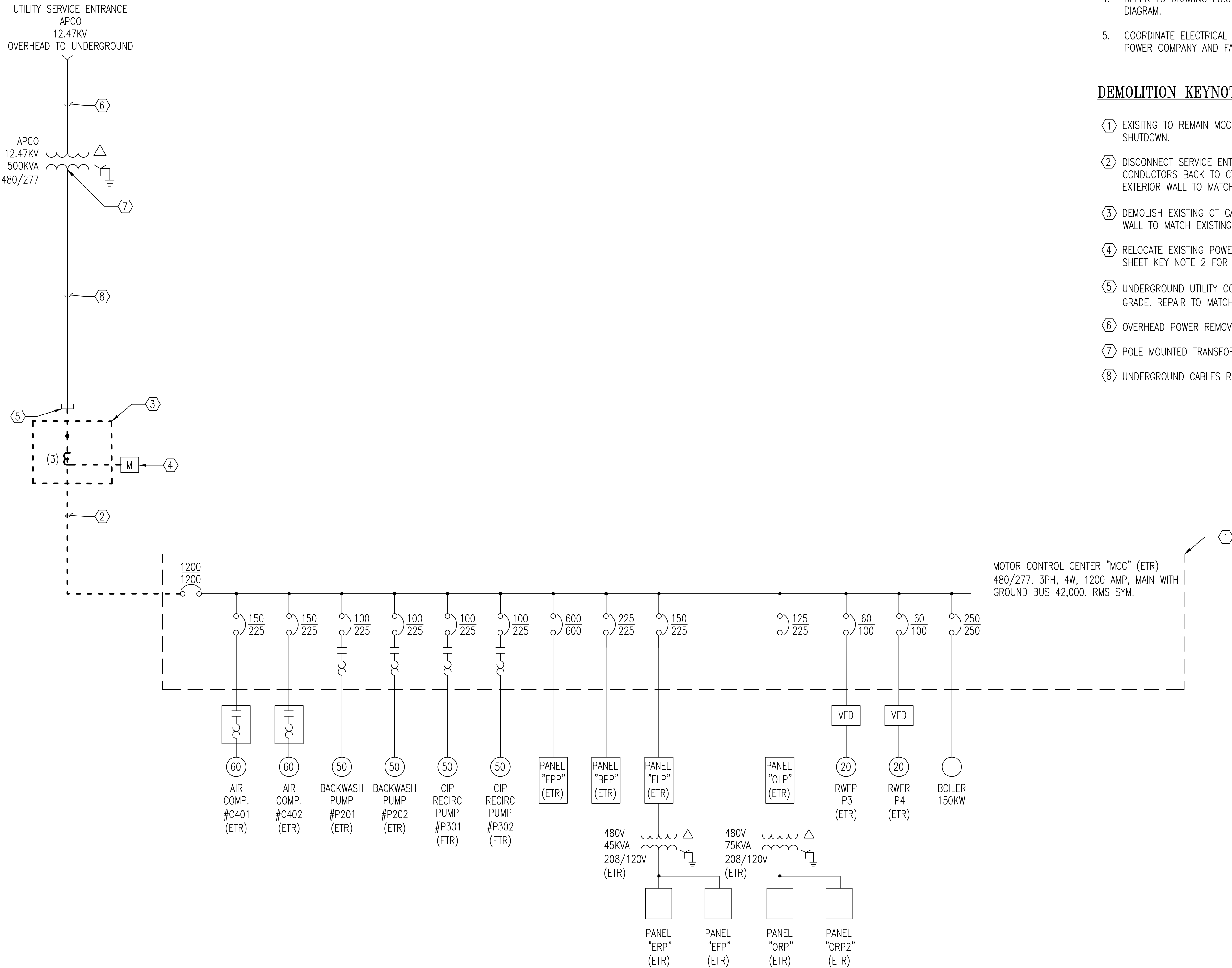
ELECTRICAL DEMOLITION ONE-LINE DIAGRAM SCALE: NONE
