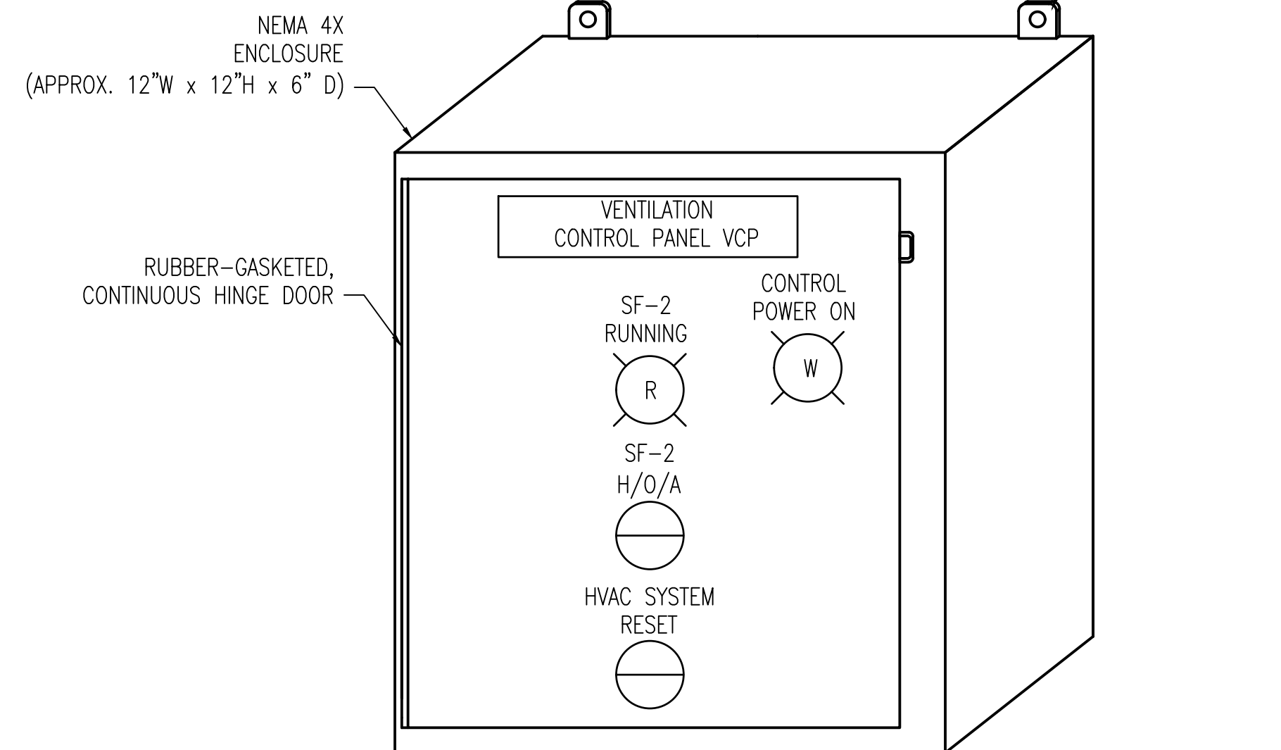
2 VENTILATION CONTROL PANEL ELEVATION SCALE: NONE
