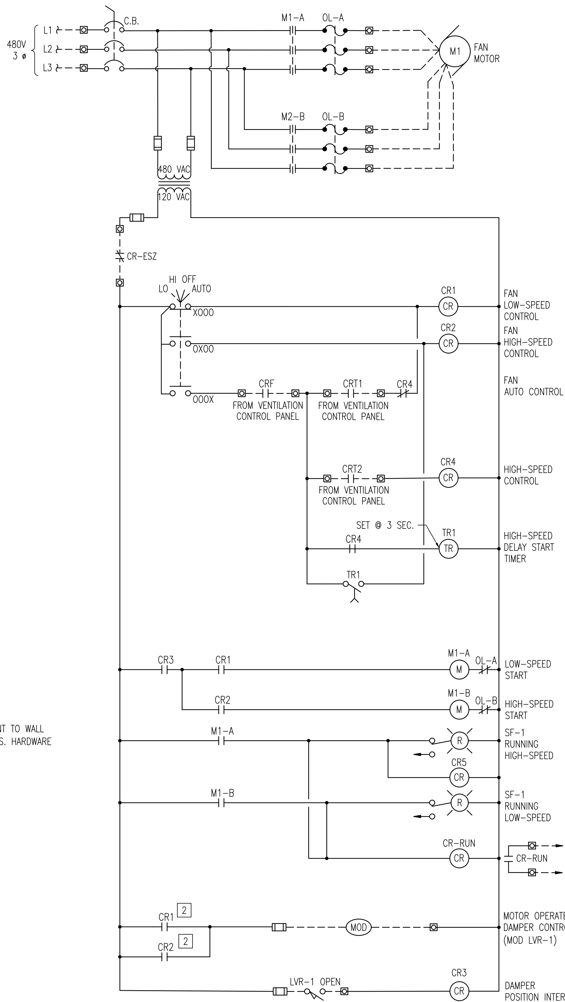
3 2-SPEED FAN MOTOR STARTER ELEMENTARY SCALE: NONE (SF-1 SHOWN, TYP. FOR EF-1)
