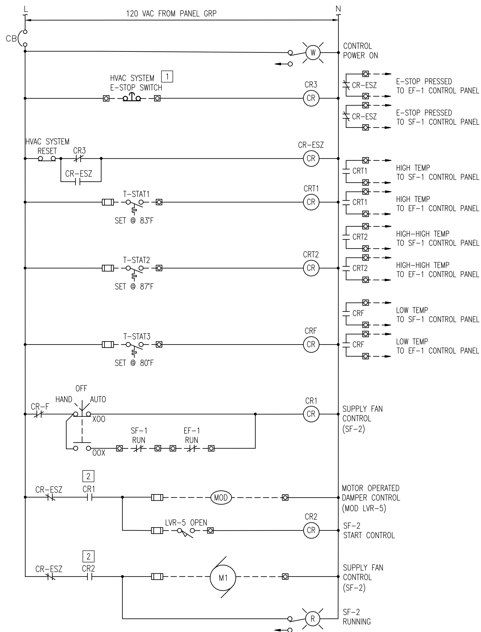
1 VENTILATION CONTROL PANEL ELEMENTARY SCALE: NONE
