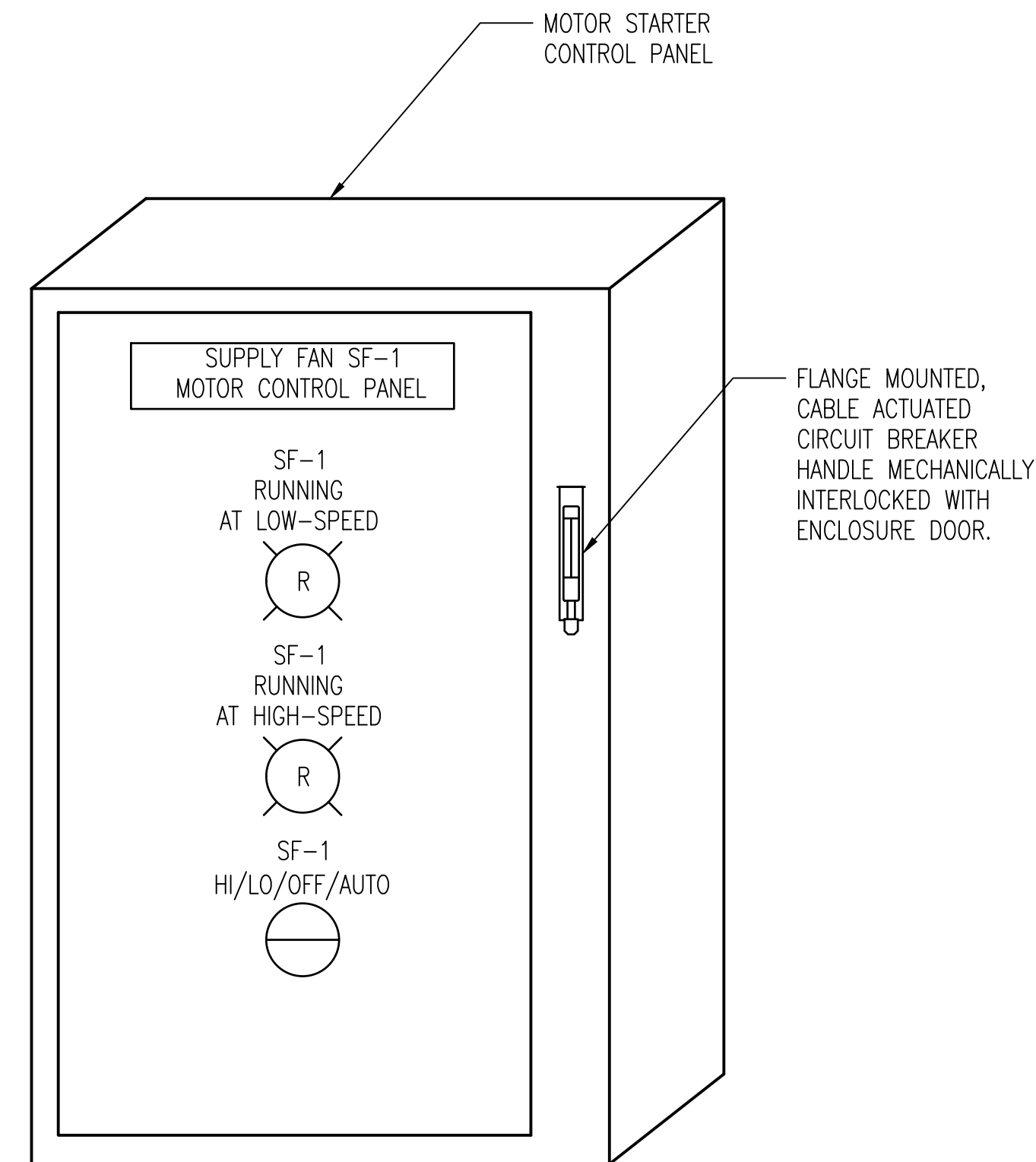
4 2-SPEED FAN MOTOR CONTROL PANEL ELEVATION SCALE: NONE (SF-1 SHOWN, TYP. FOR EF-1)
