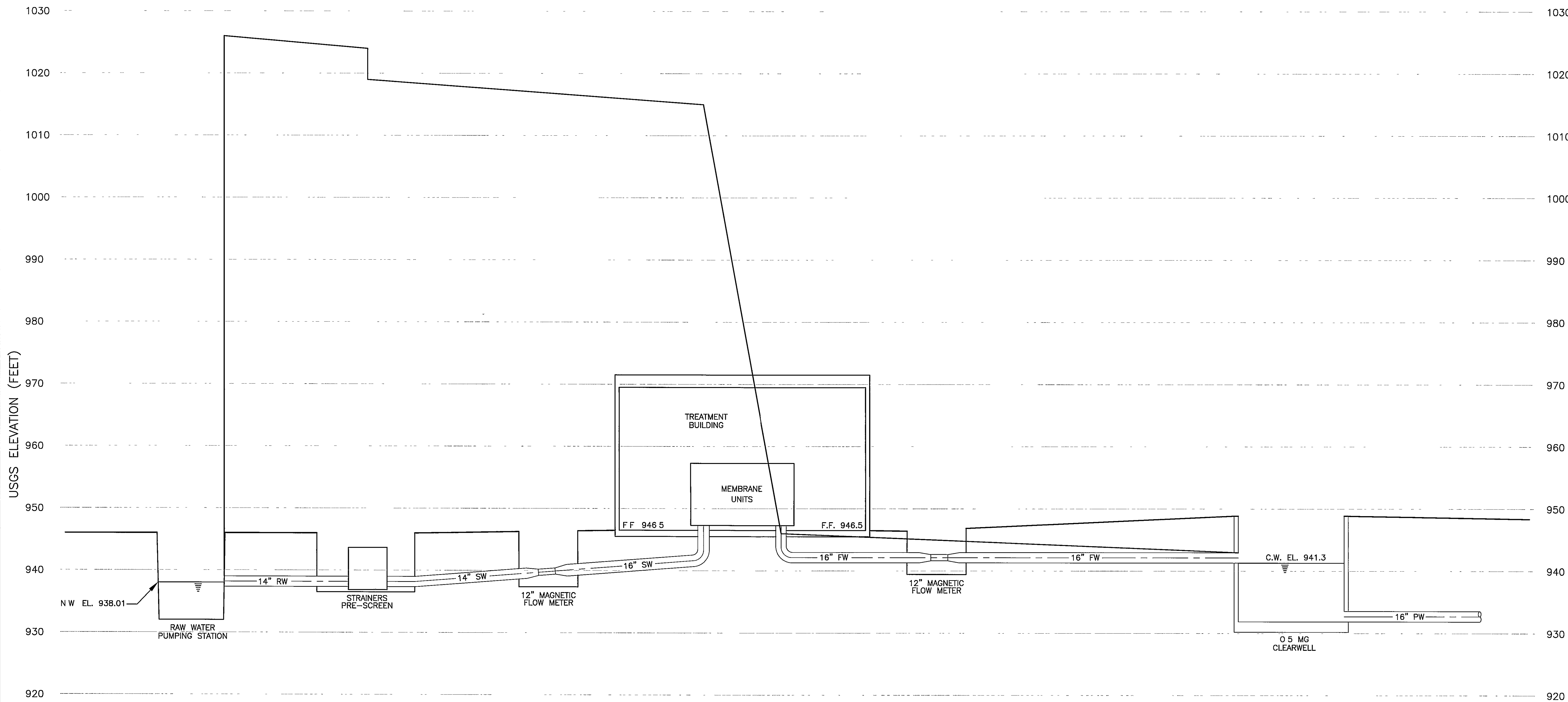
MAIN PROCESS HYDRAULIC PROFILE NO SCALE
