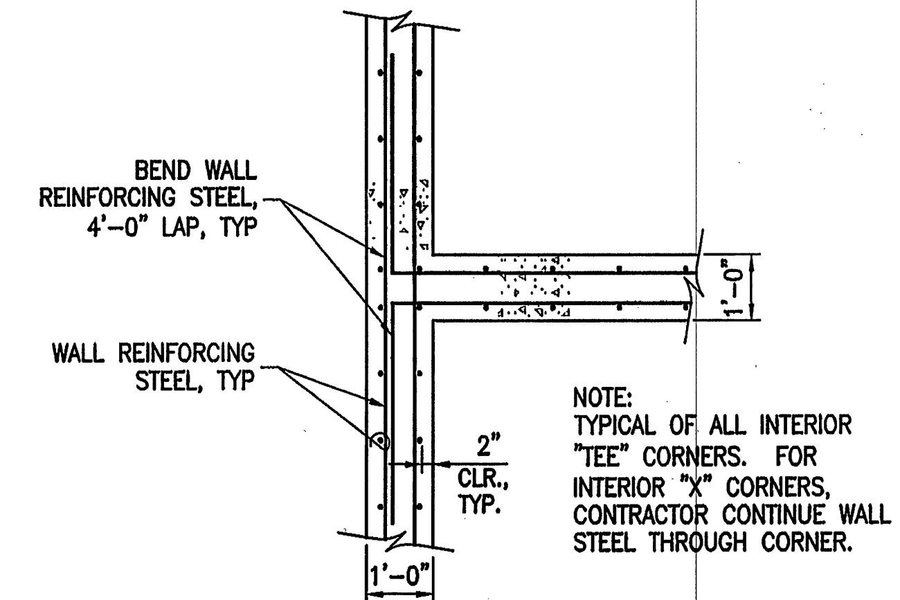
WALL CORNER DETAIL 'C' SCALE: 1/2"=1'-0"
