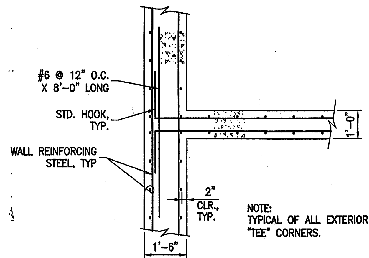
WALL CORNER DETAIL 'B' SCALE: 1/2"=1'-0"
