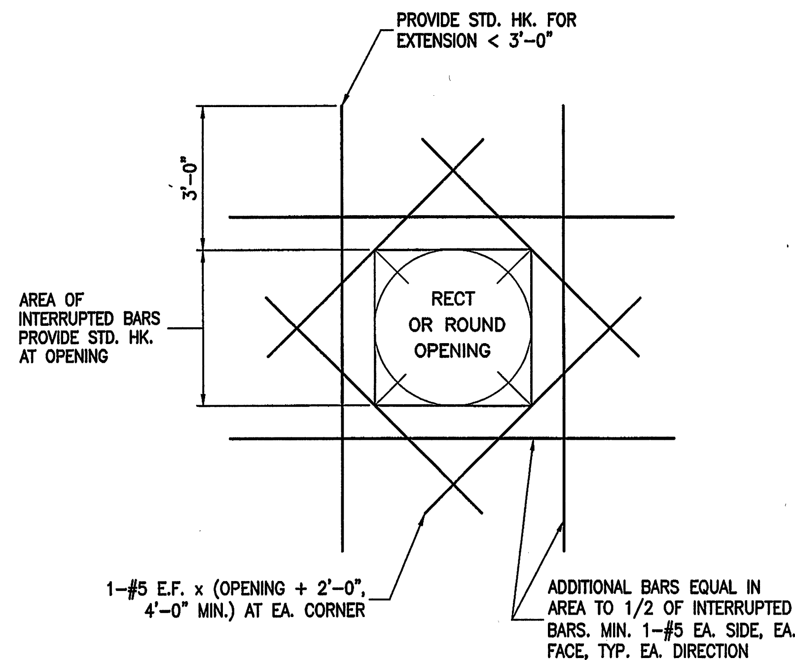
TYPICAL WALL AND SLAB OPENING DETAIL NOT TO SCALE
