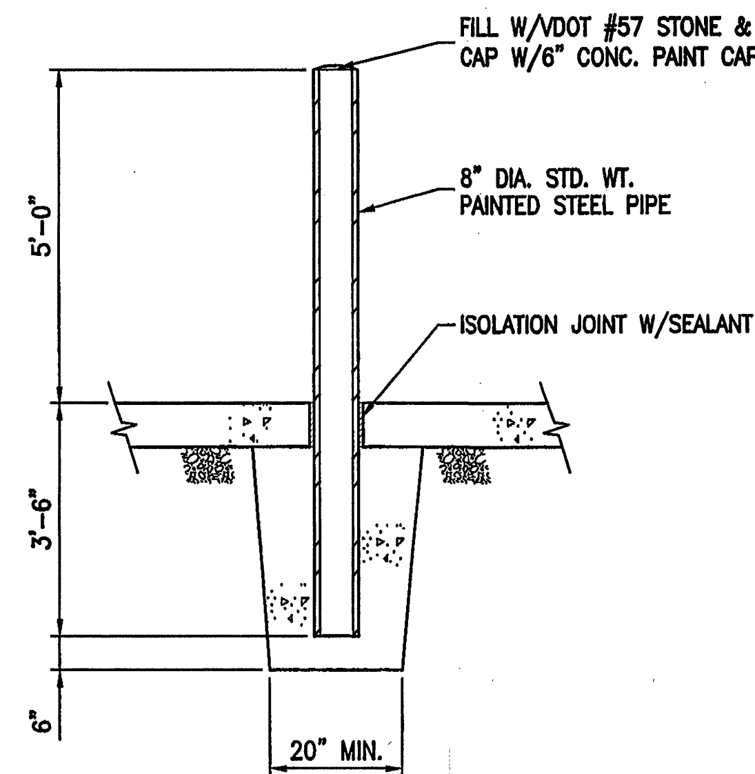
BOLLARD DETAIL NOT TO SCALE
