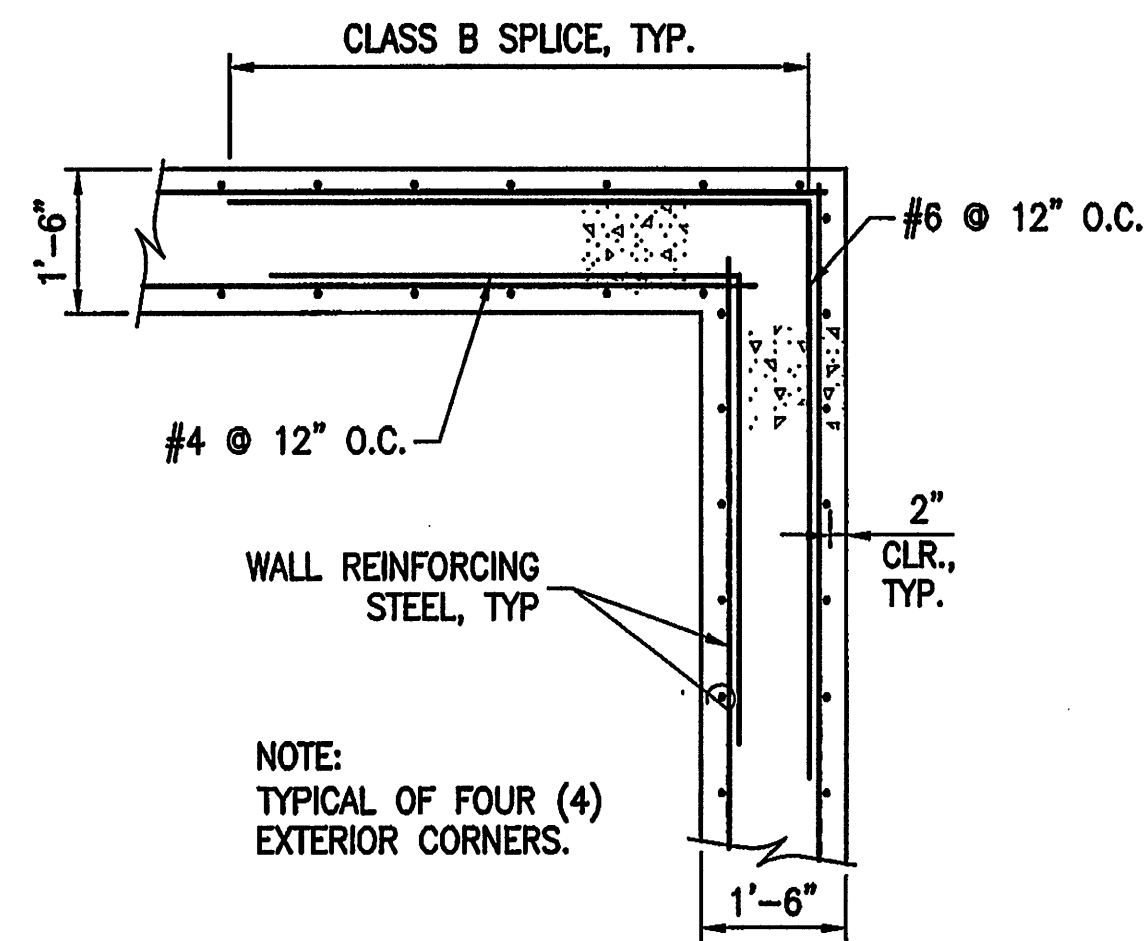
WALL CORNER DETAIL 'A' SCALE: 1/2"=1'-0"
