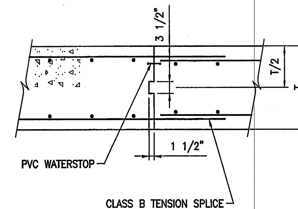
TYP. WALL AND SLAB CONSTRUCTION JOINT DETAIL NOT TO SCALE
