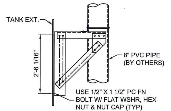
INTERIOR PIPE SUPPORT DETAIL 1
