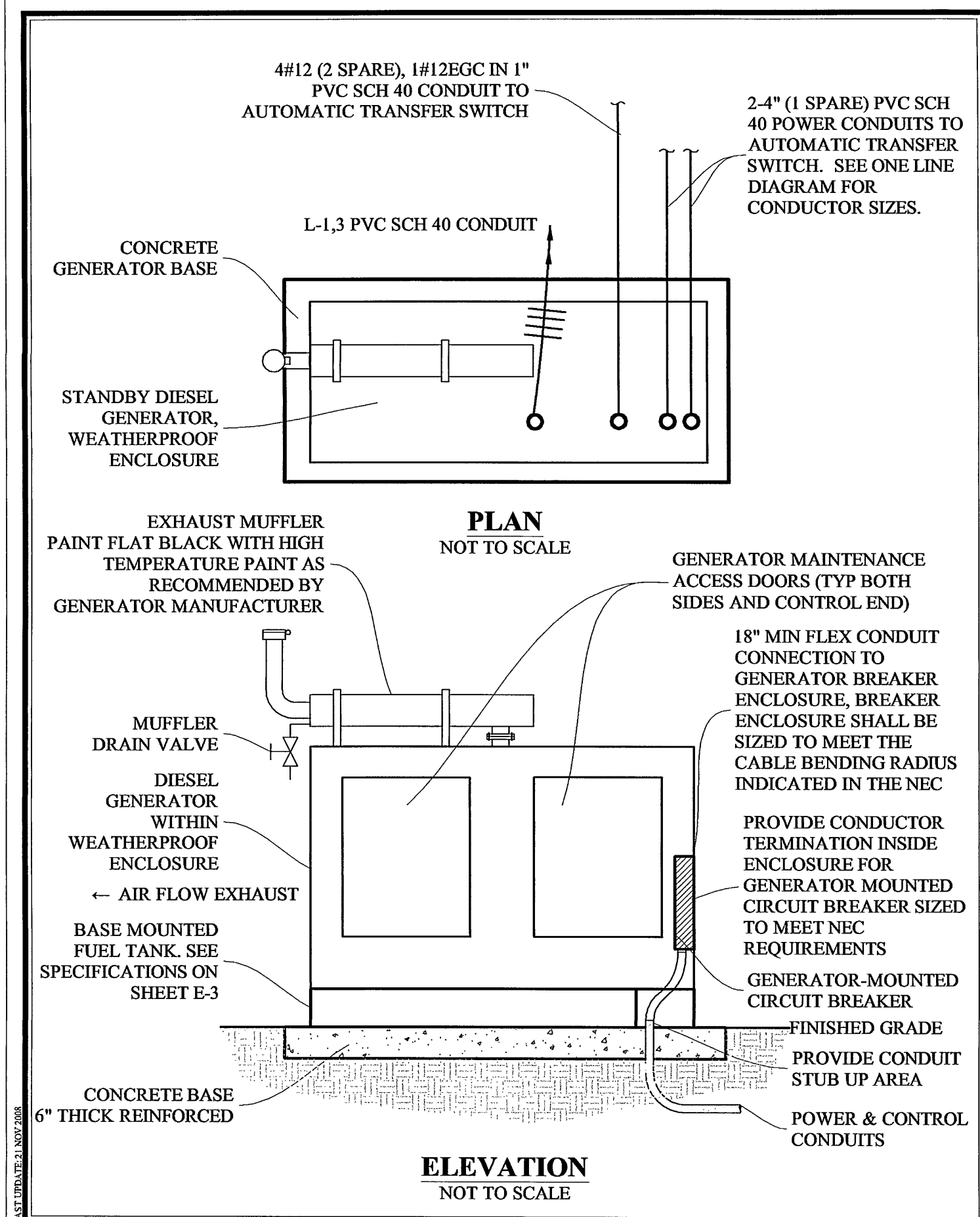
ACS PUMP STATION GENERATOR DESIGN WWW.ACSDESIGNLLC.COM ■ ENGINEERING ■ SURVEYING ■ LANDSCAPE ARCHITECTURE ■ CONSTRUCTION MANAGEMENT
