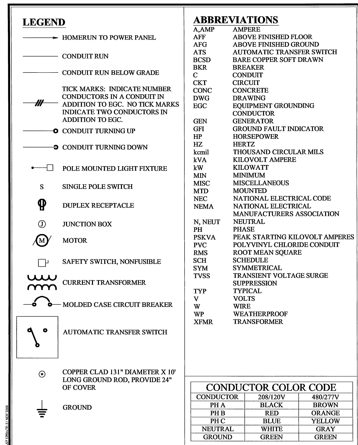
ACS ELECTRICAL DIAGRAM LEGEND AND ABBREVIATIONS DESIGN WWW.ACSDESIGNLLC.COM ■ ENGINEERING ■ SURVEYING ■ LANDSCAPE ARCHITECTURE ■ CONSTRUCTION MANAGEMENT
