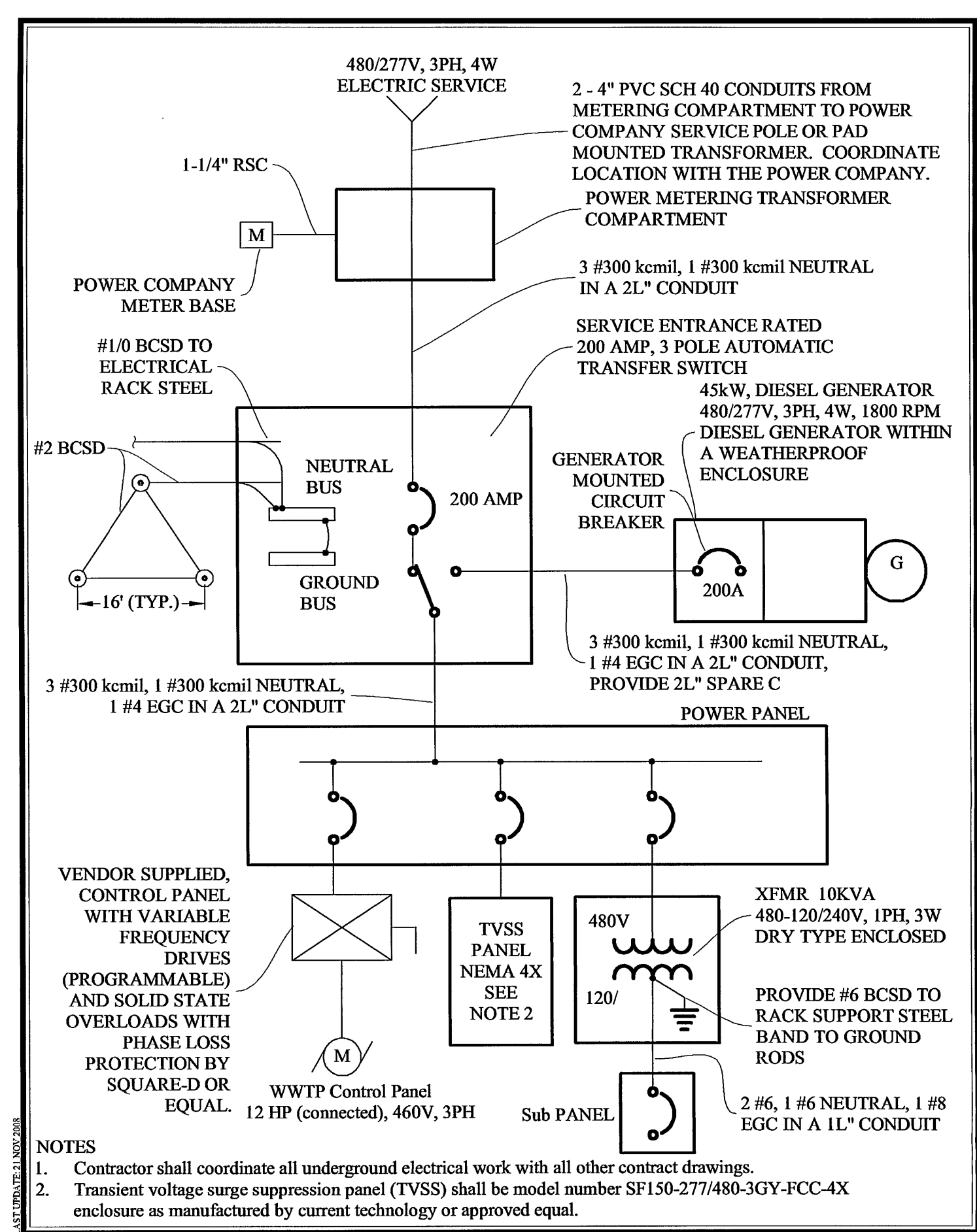
ACS ELECTRICAL SERVICE - ONE LINE DIAGRAM DESIGN WWW.ACSDESIGNLLC.COM ■ ENGINEERING ■ SURVEYING ■ LANDSCAPE ARCHITECTURE ■ CONSTRUCTION MANAGEMENT
