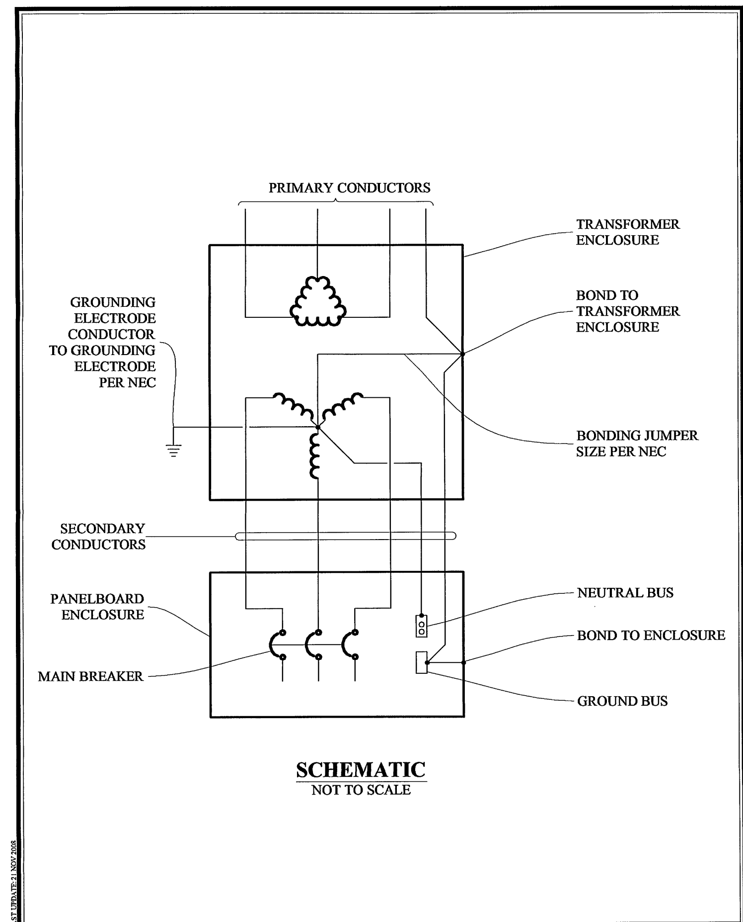
ACS DRY TYPE TRANSFORMER WIRING DIAGRAM DESIGN WWW.ACSDESIGNLLC.COM ■ ENGINEERING ■ SURVEYING ■ LANDSCAPE ARCHITECTURE ■ CONSTRUCTION MANAGEMENT
