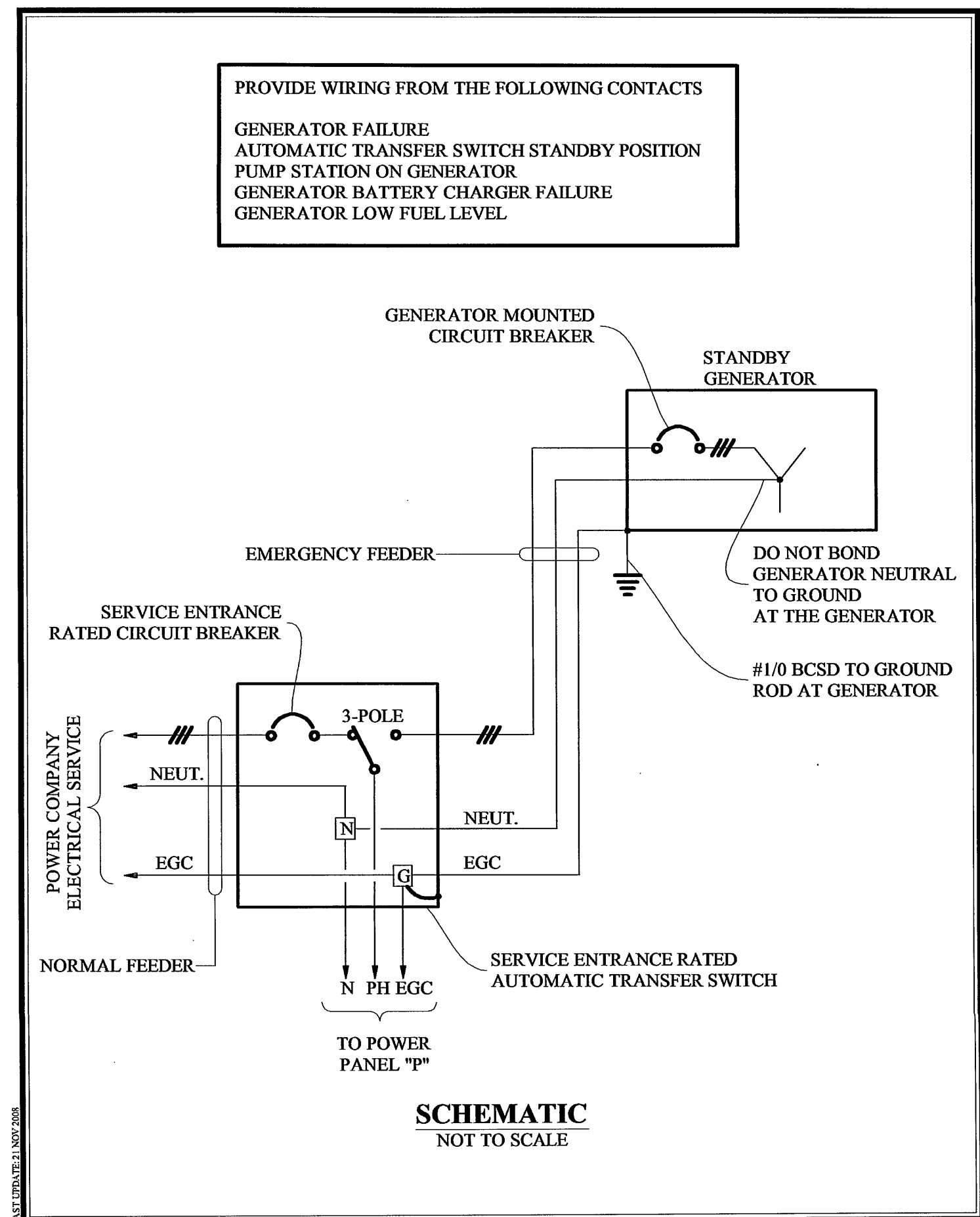
ACS CONNECTION DIAGRAM - NEUTRAL & GROUND CONDUCTORS DESIGN WWW.ACSDESIGNLLC.COM ■ ENGINEERING ■ SURVEYING ■ LANDSCAPE ARCHITECTURE ■ CONSTRUCTION MANAGEMENT
