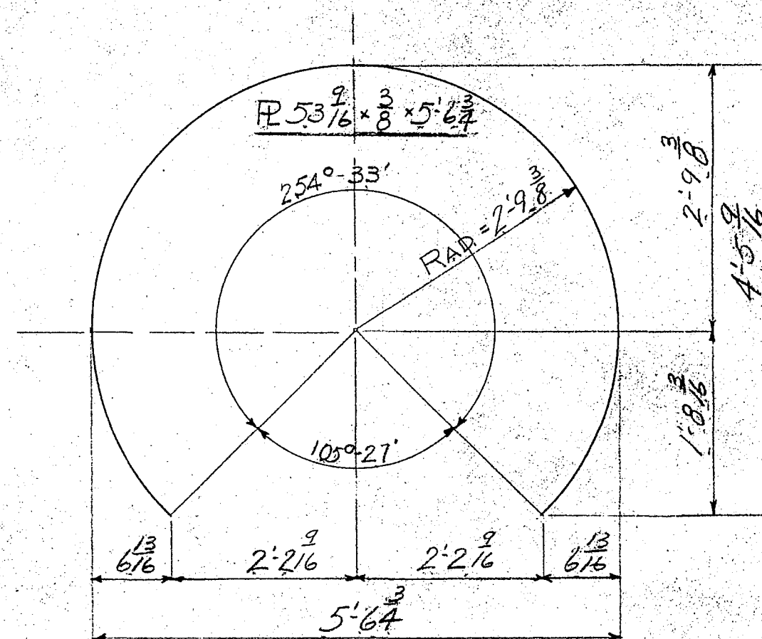
R(pa) DEVELOPED
