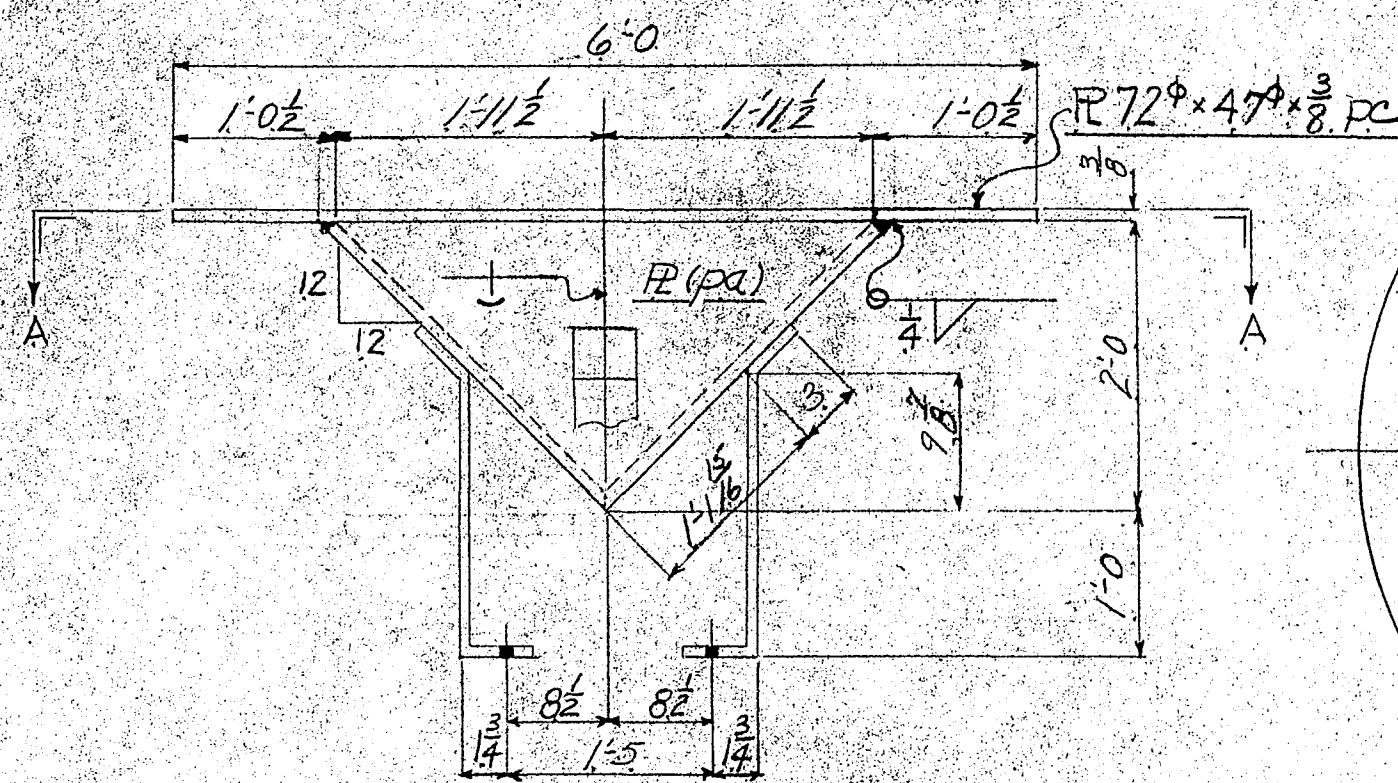
1- DEFLECTOR PLATE - D
