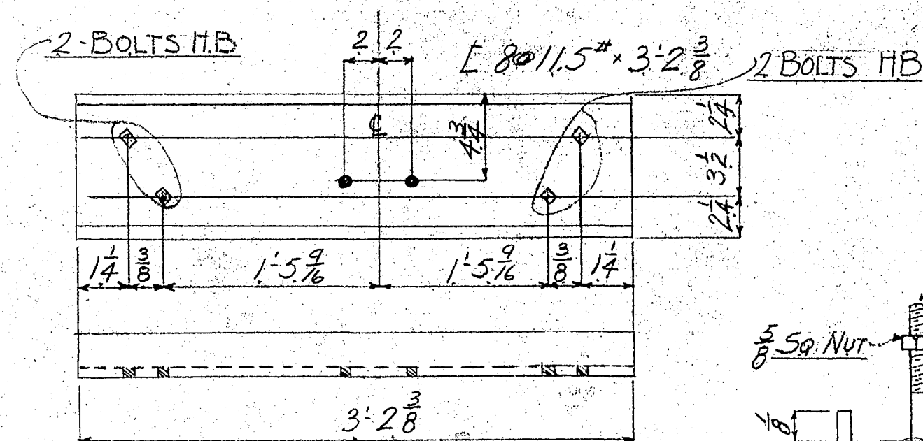
1- FLOAT BRACKET - FB
