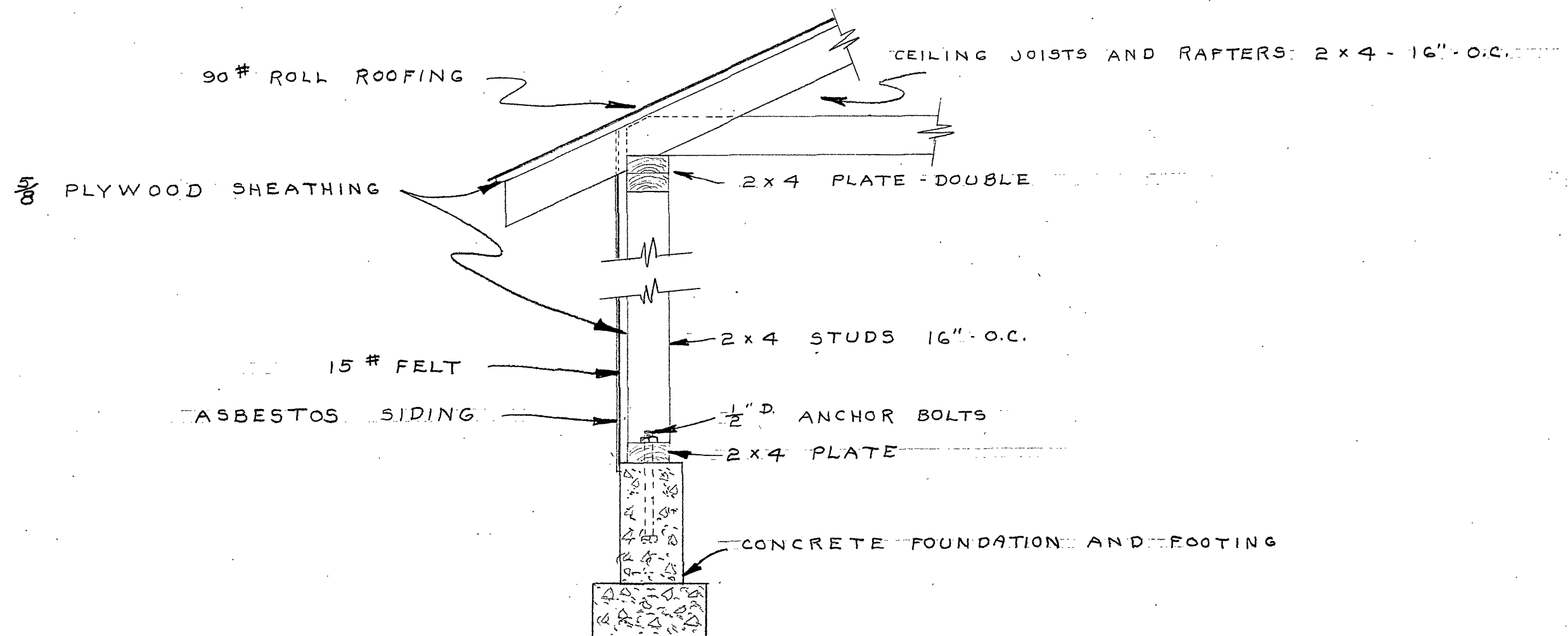
TYPICAL WALL SECTION SCALE 1" = 1'
