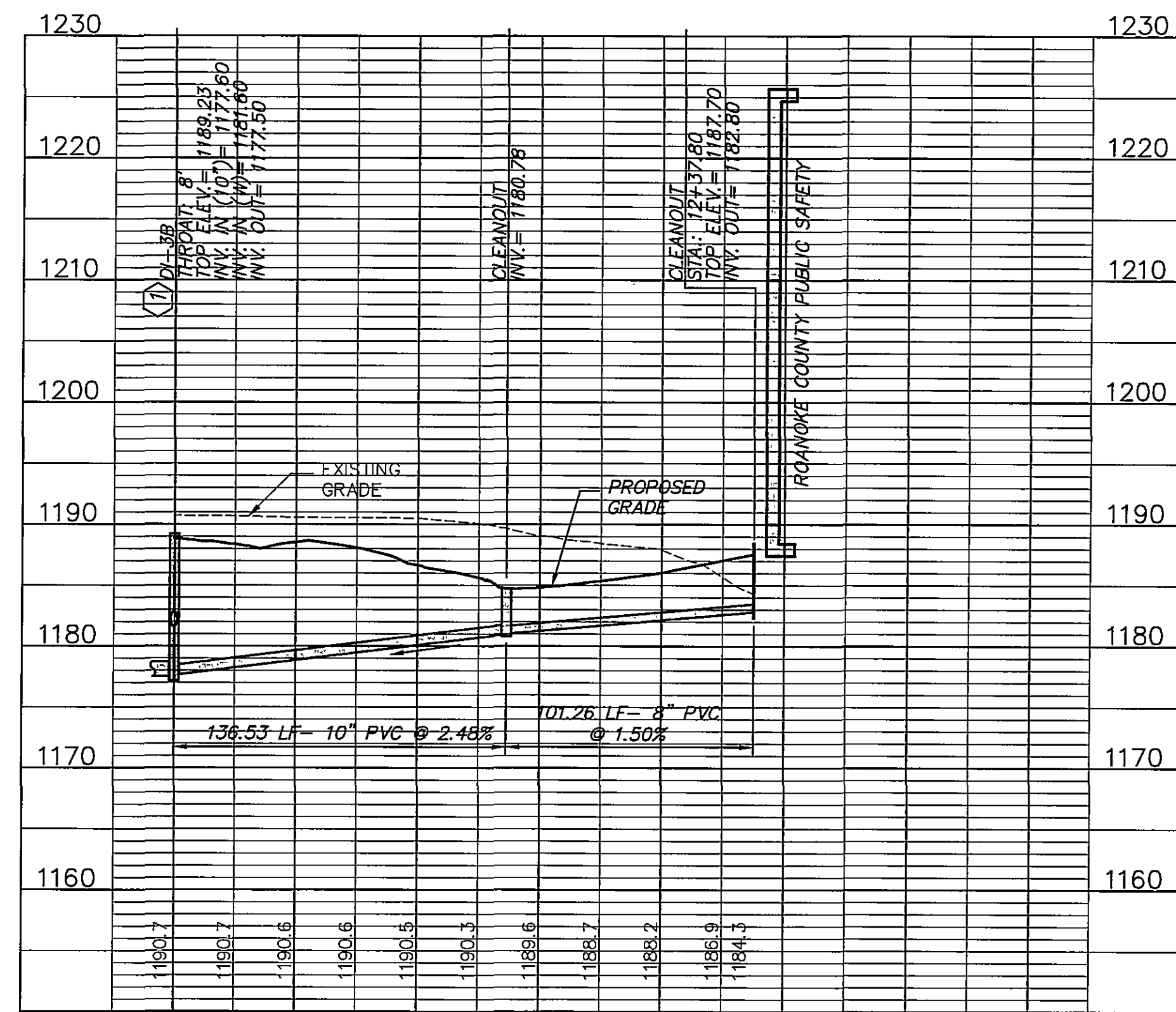
STORM WATER LINE C
