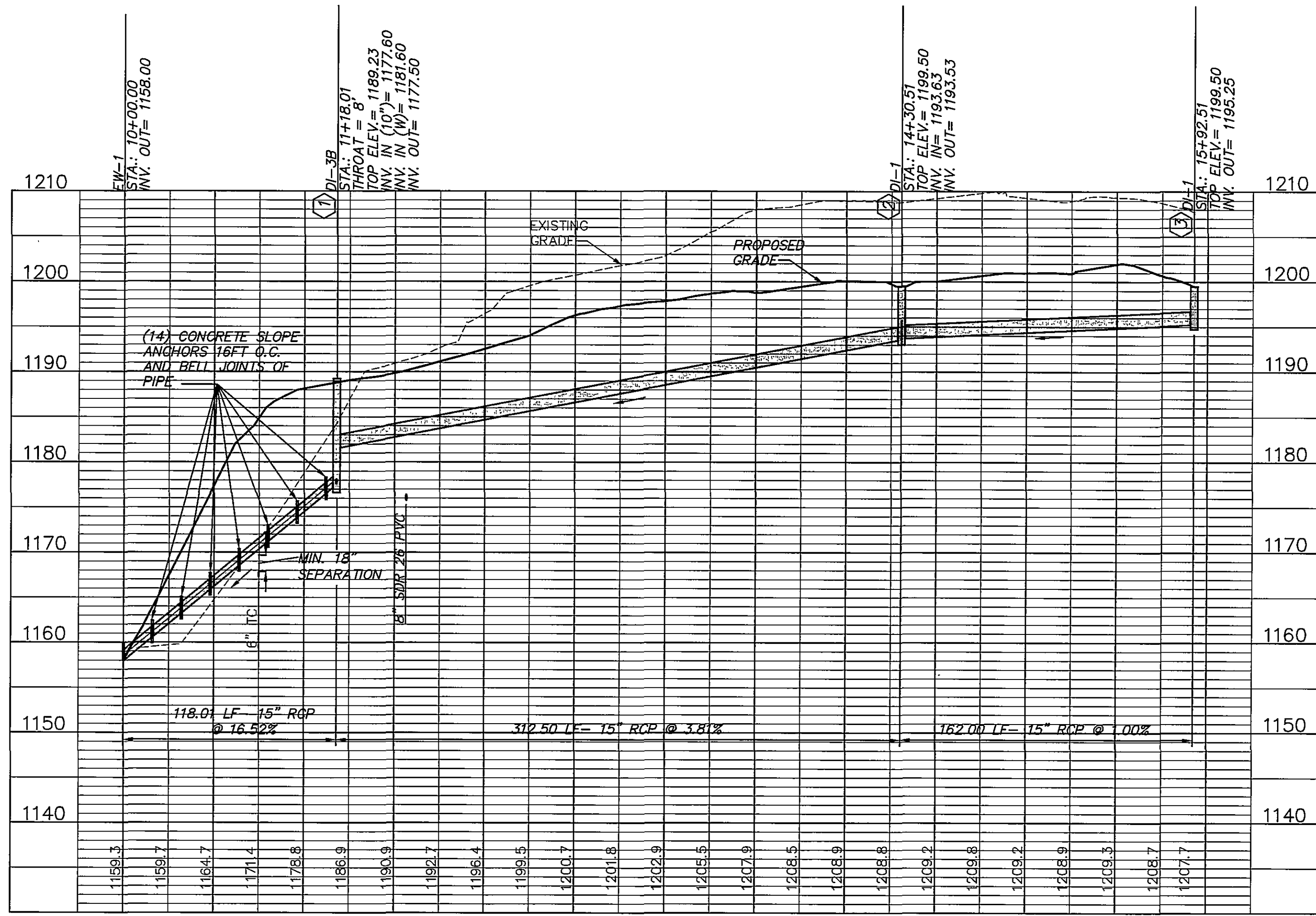
STORM WATER LINE A
