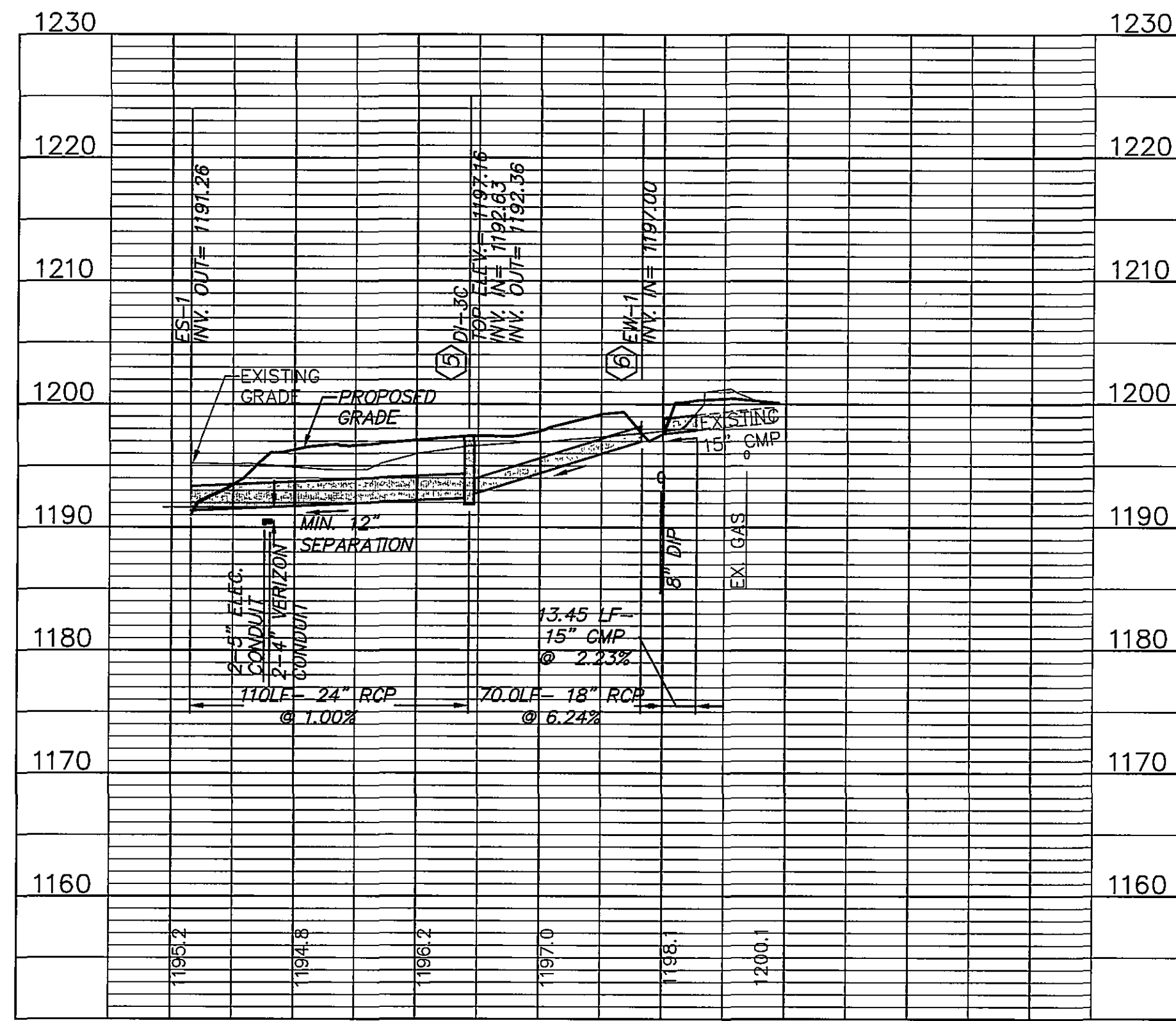
STORM WATER LINE B
