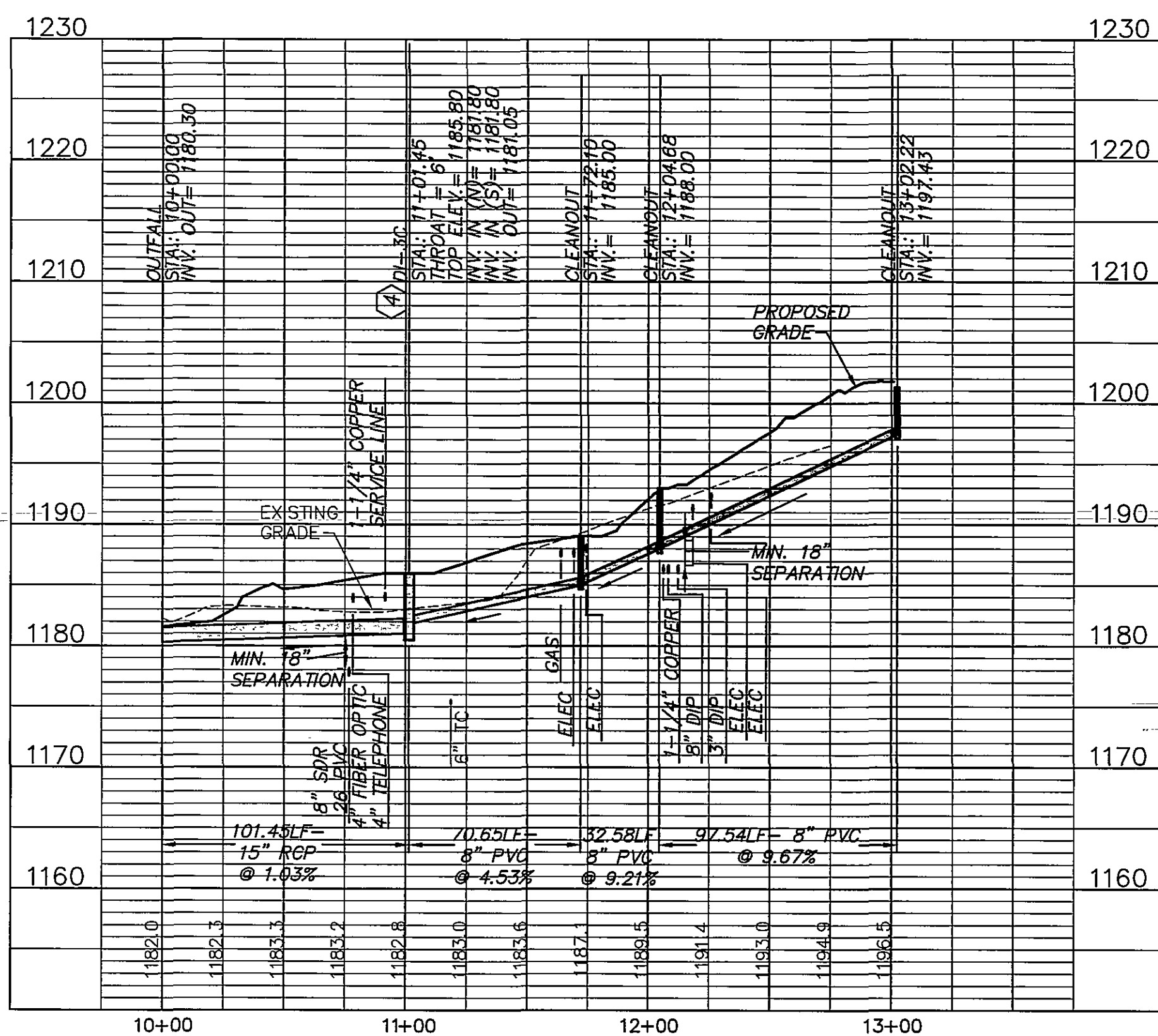
STORM WATER LINE D
