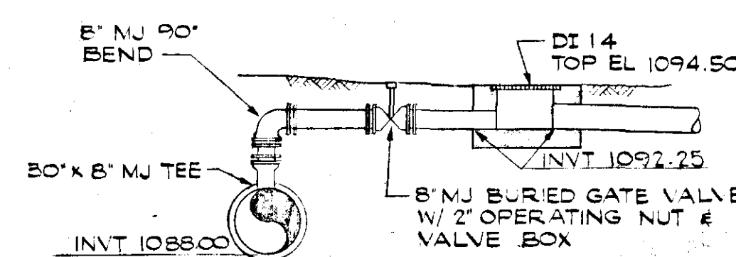
SECTION C1.1 SCALE: 3/16" = 1'-0"
