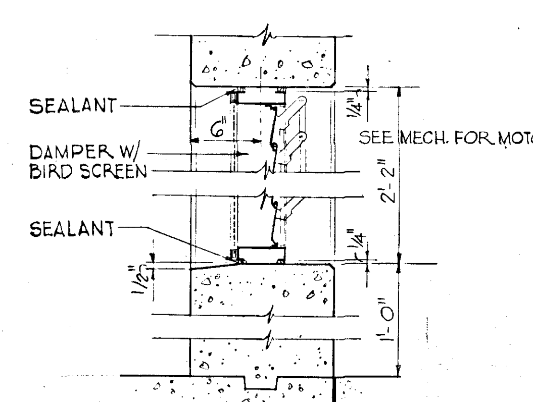
SECTION A3.3 SCALE 1/4" = 1'-0"
