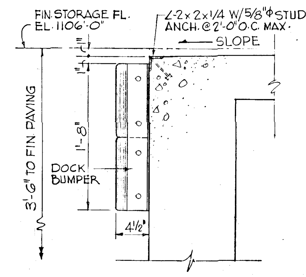
SECTION A3.7 SCALE 1/2" = 1'-0"
