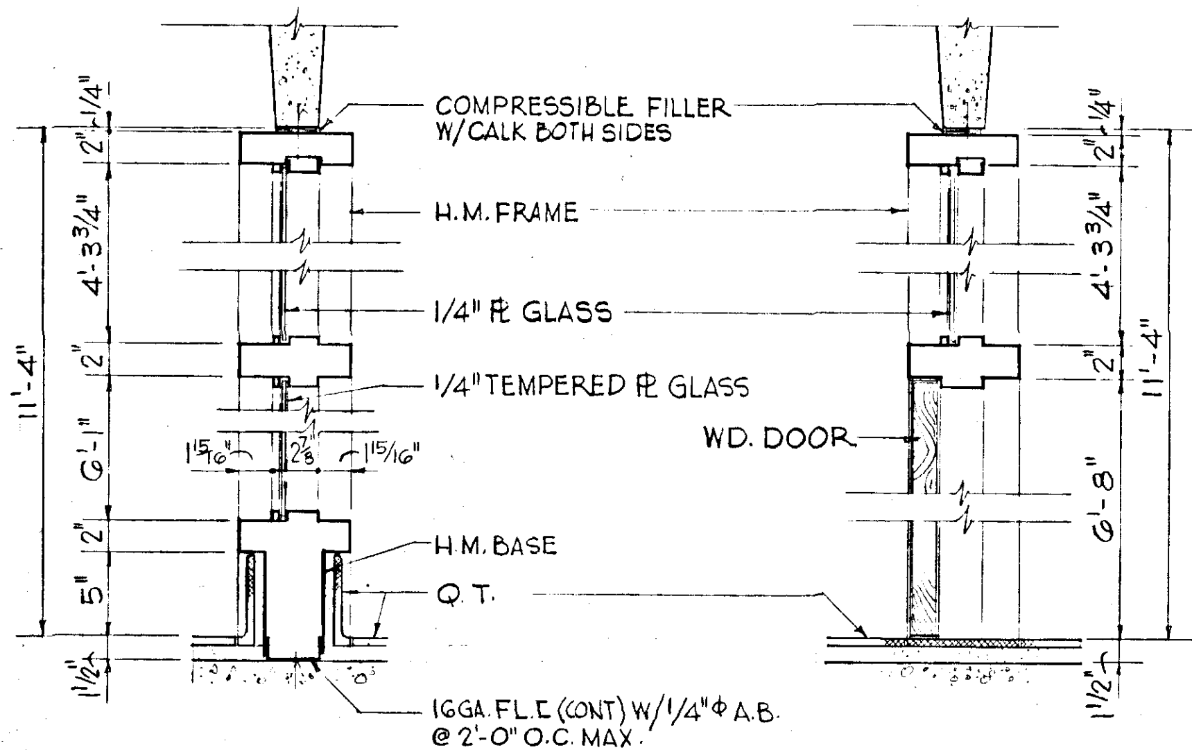
SECTION A3.4 SCALE 1/2" = 1'-0"
