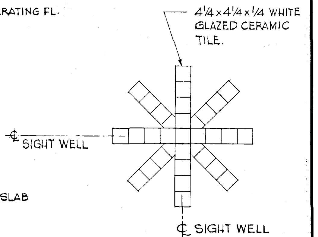
DETAIL A3.10 SCALE 3/4" = 1'-0"
