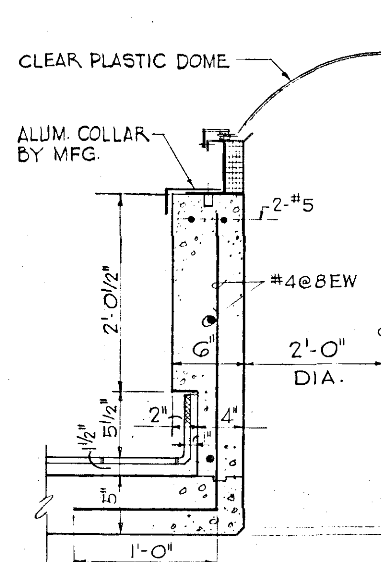
SECTION A3.6 SCALE 1/2" = 1'-0"
