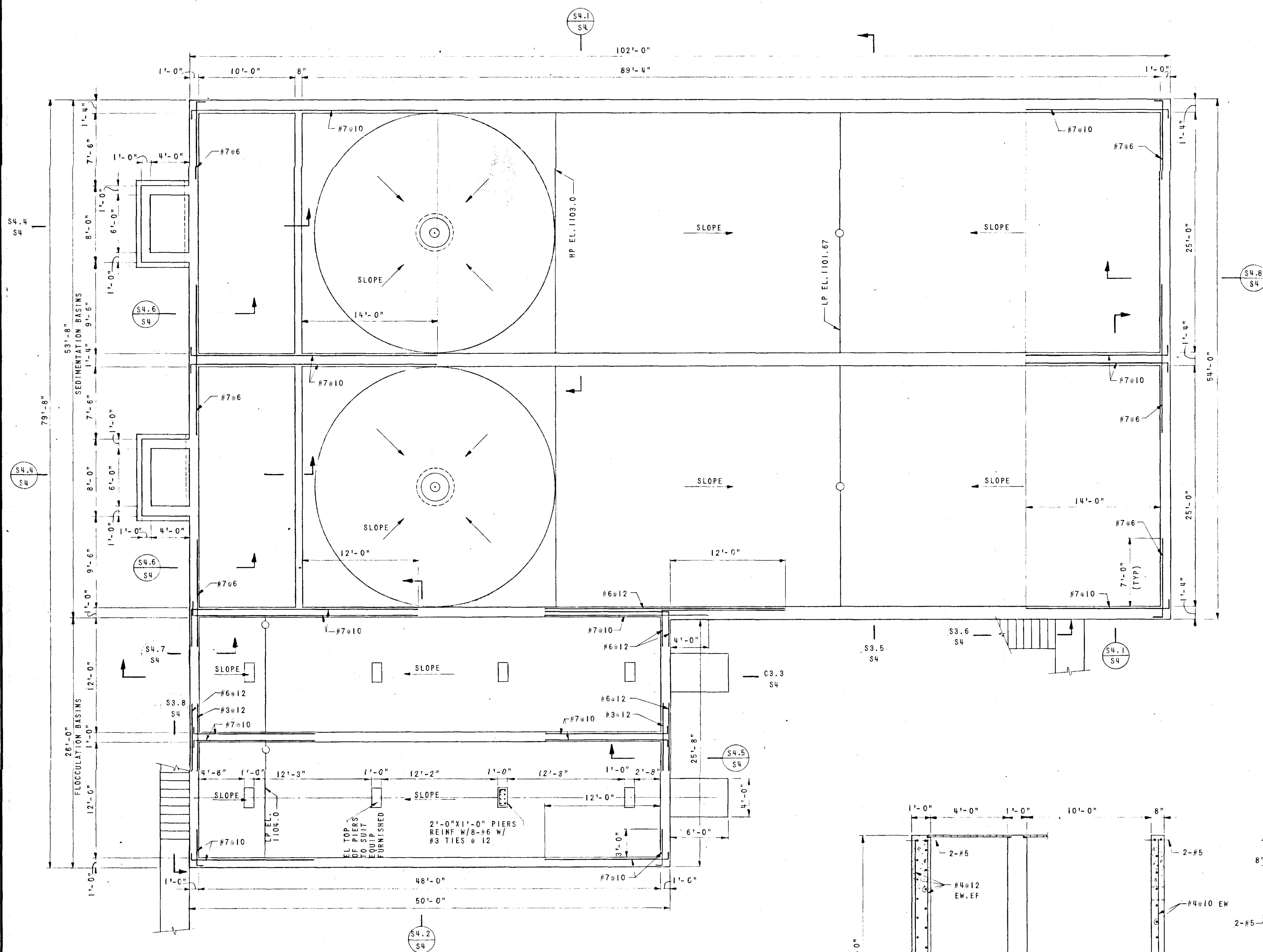
SECTIONAL PLAN FLOCCULATION & SEDIMENTATION BASINS
