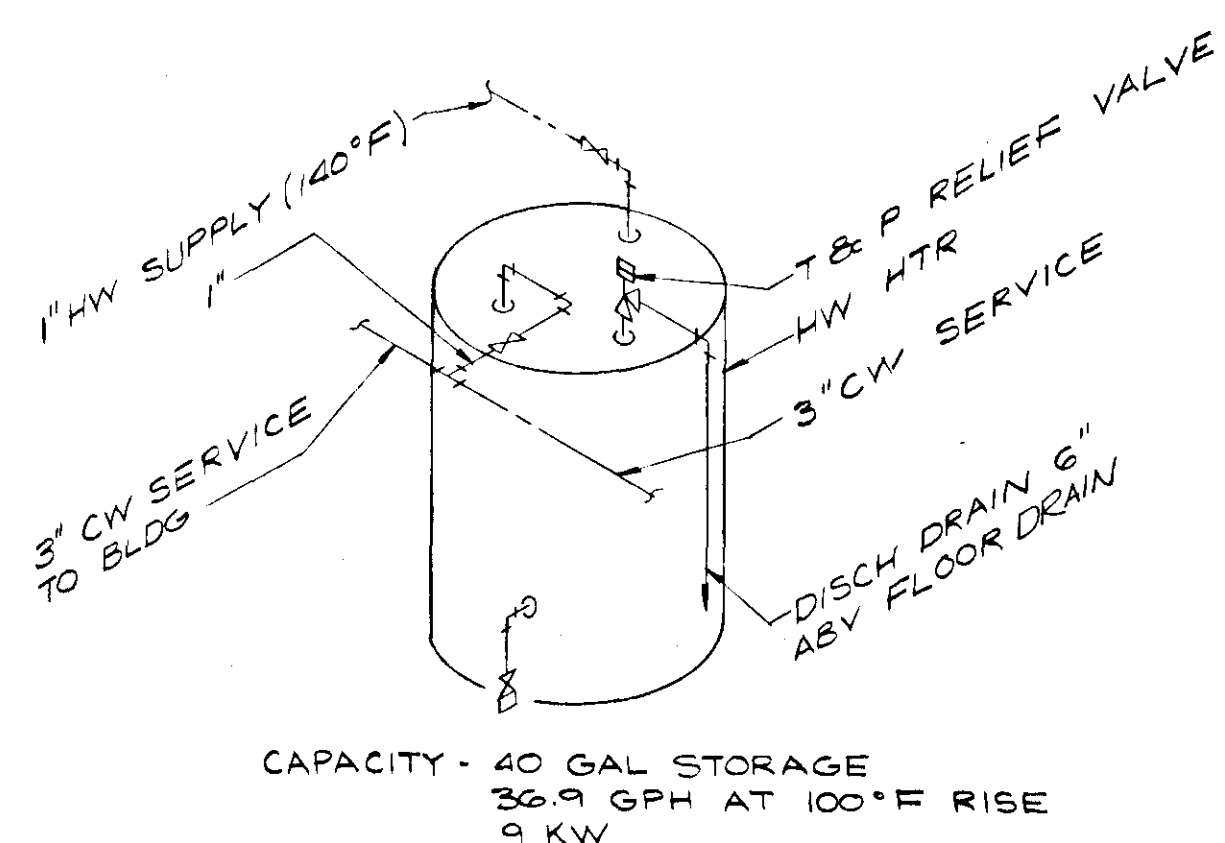
DETAIL - HW HEATER NO SCALE
