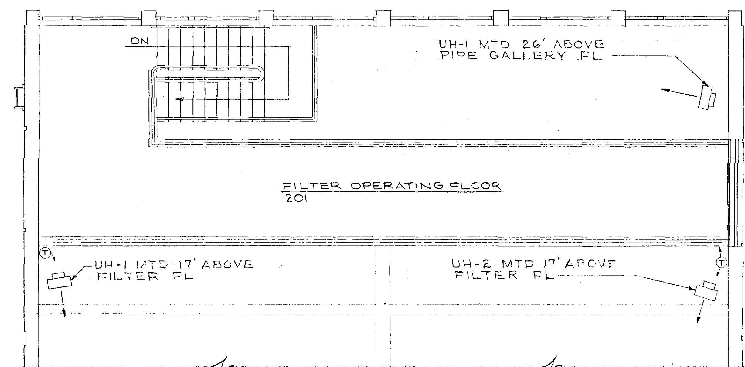
FILTER OPERATING FLOOR PLAN SCALE: 1/4"=1'-0"
