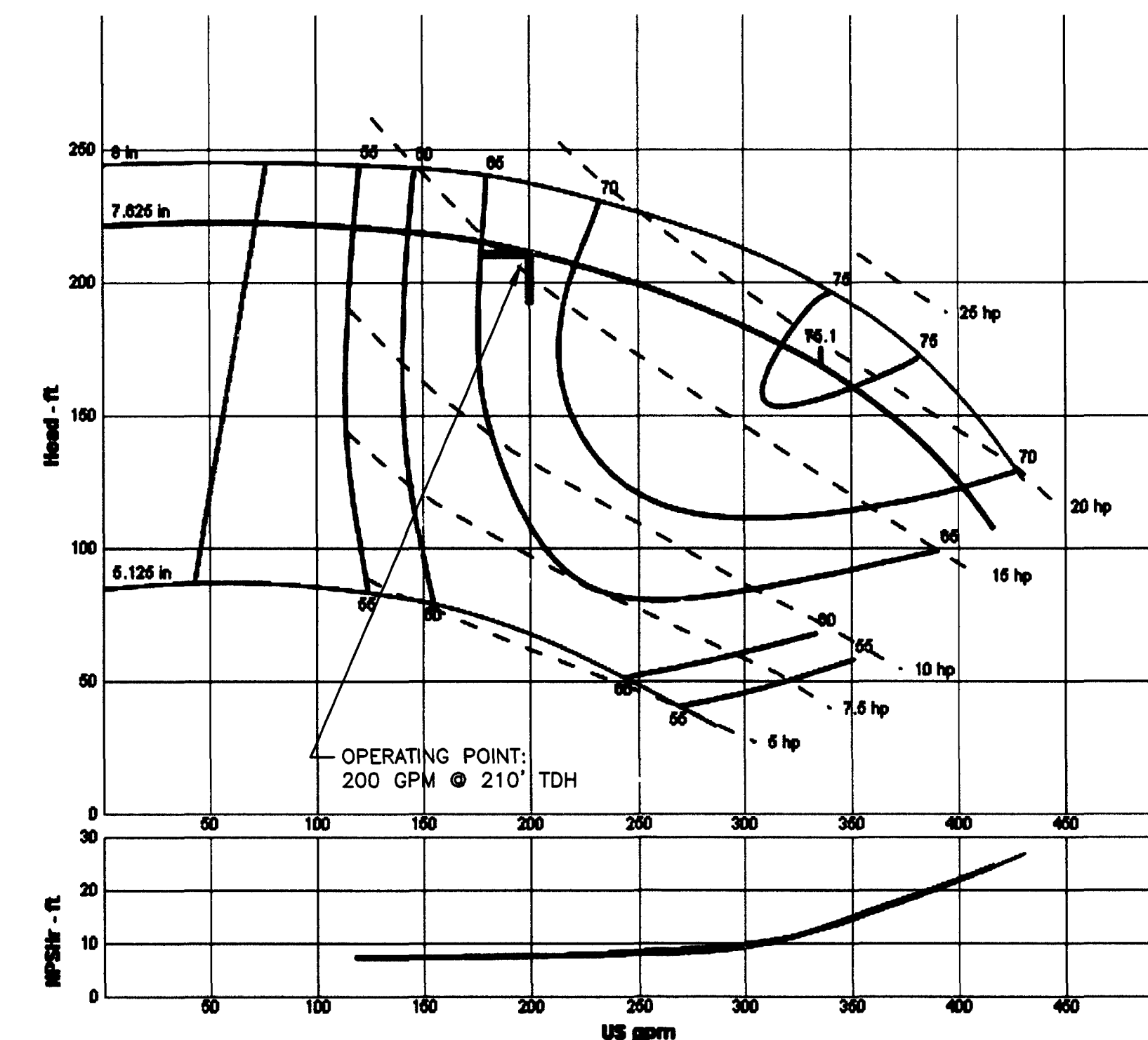
PUMP CURVE
