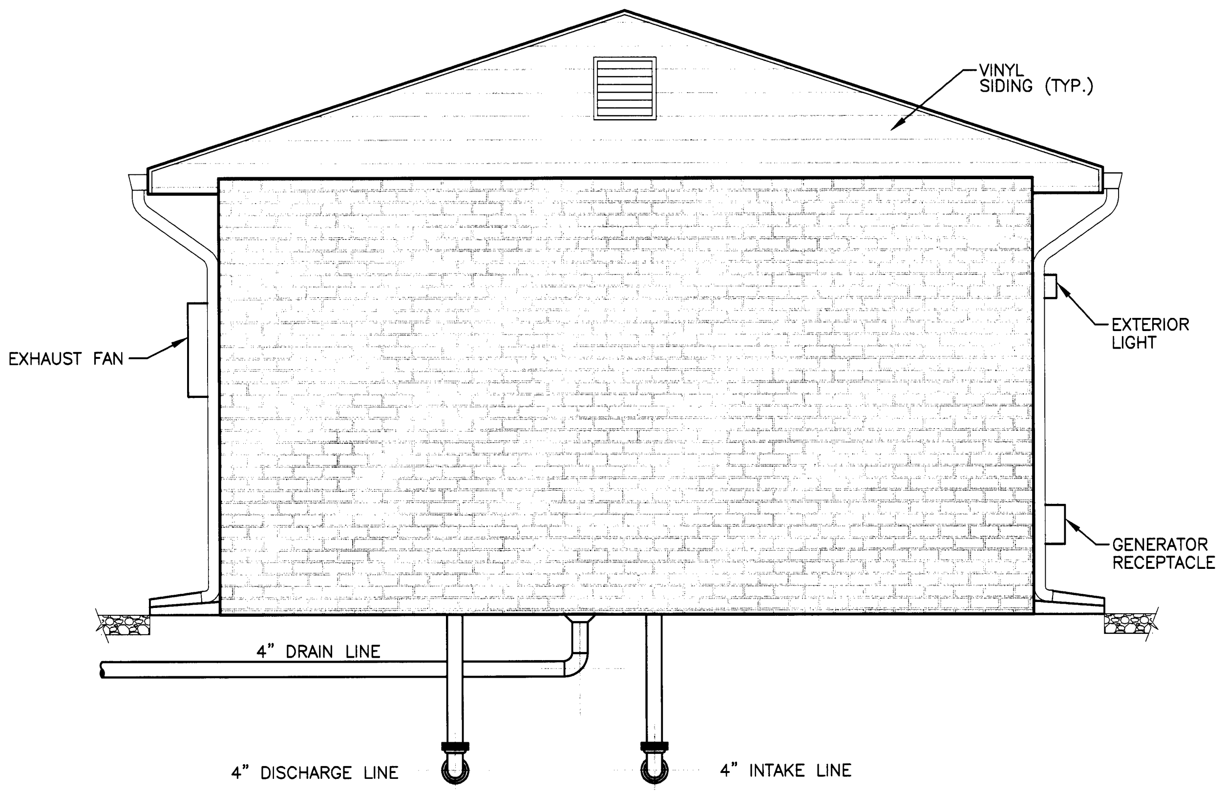
NORTH ELEVATION SCALE: 1/2" = 1'-0"
