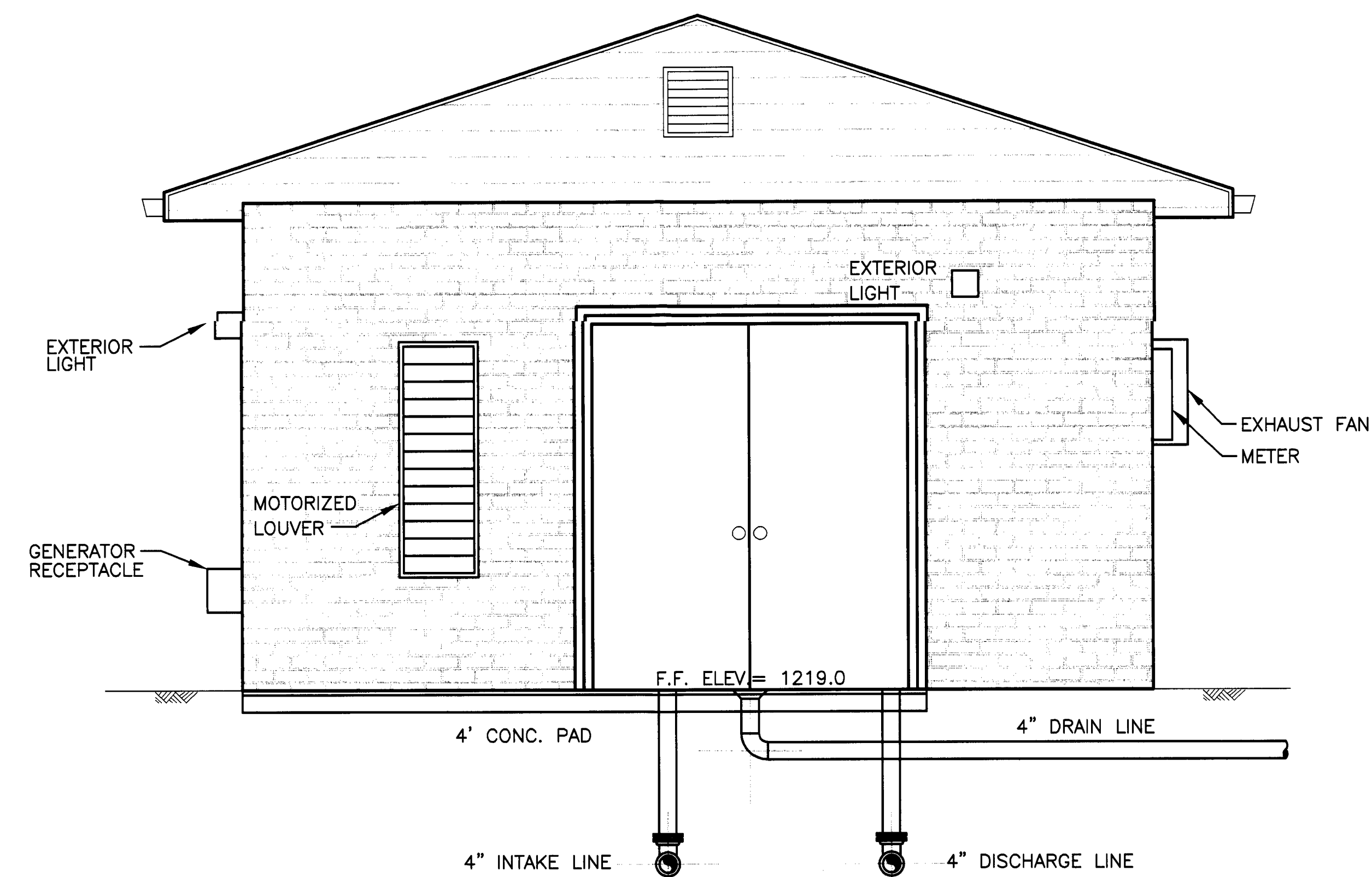
SOUTH ELEVATION SCALE: 1/2" = 1'-0"
