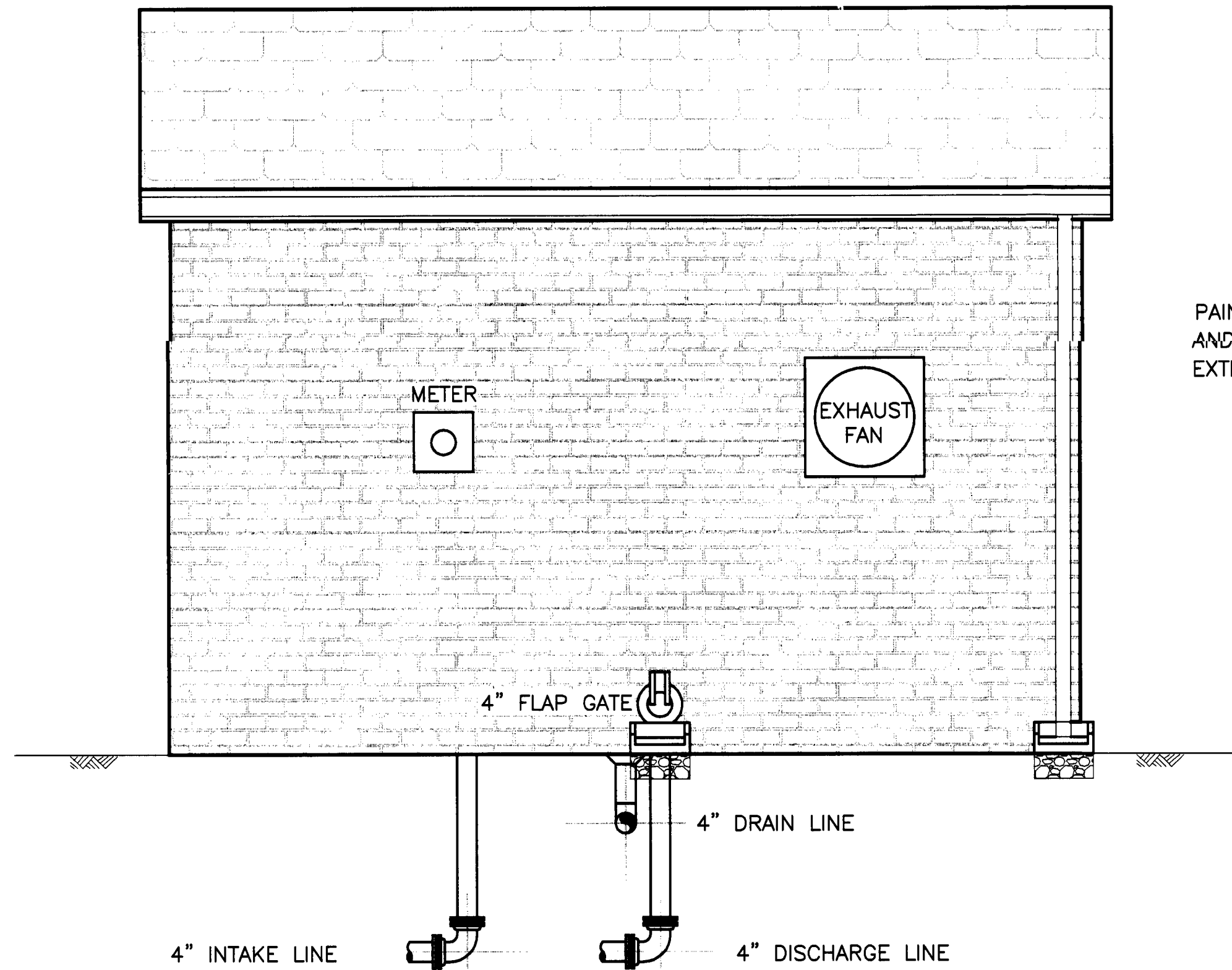
EAST ELEVATION SCALE: 1/2" = 1'-0"
