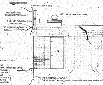
FRONT SCALE 1/4\"/>
