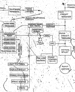
INSTRUMENTATION & PUMP CONTROL DIAGRAM N.T.S.
