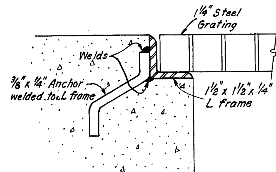
TYPICAL GRATING DETAIL One Half Scale
