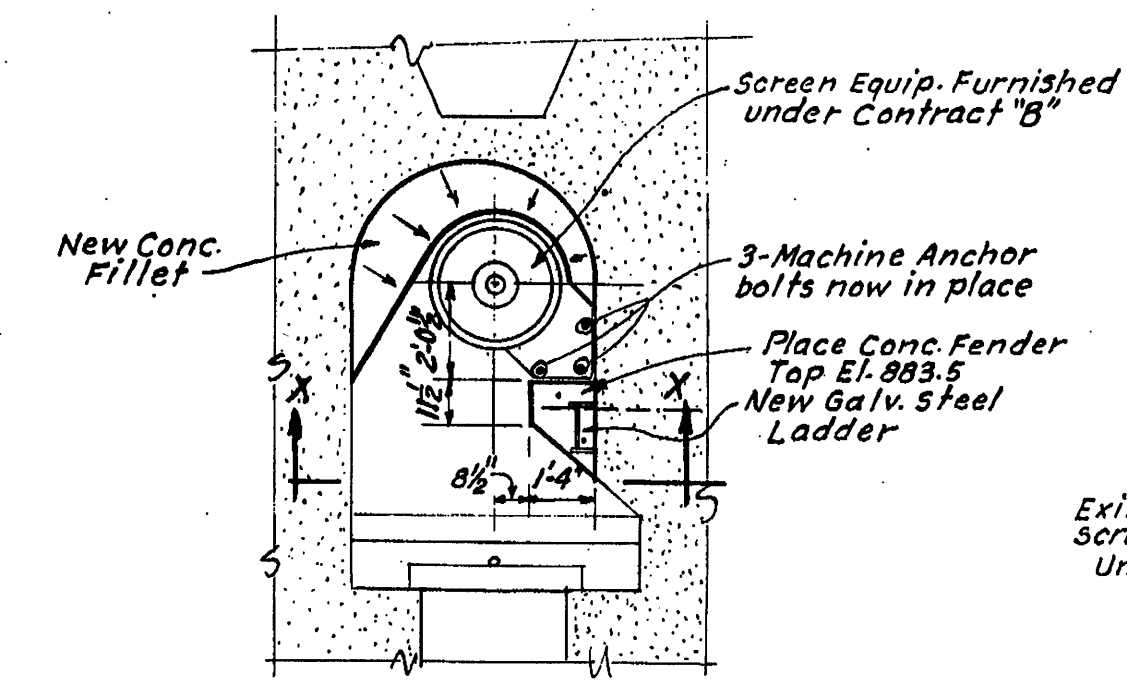
PLAN AT ELEV. 883.5
