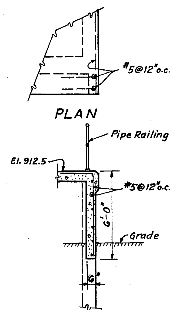
SECTION E-E DETAILS OF CURTAIN WALLS Scale: 1/2"=1'-0"
