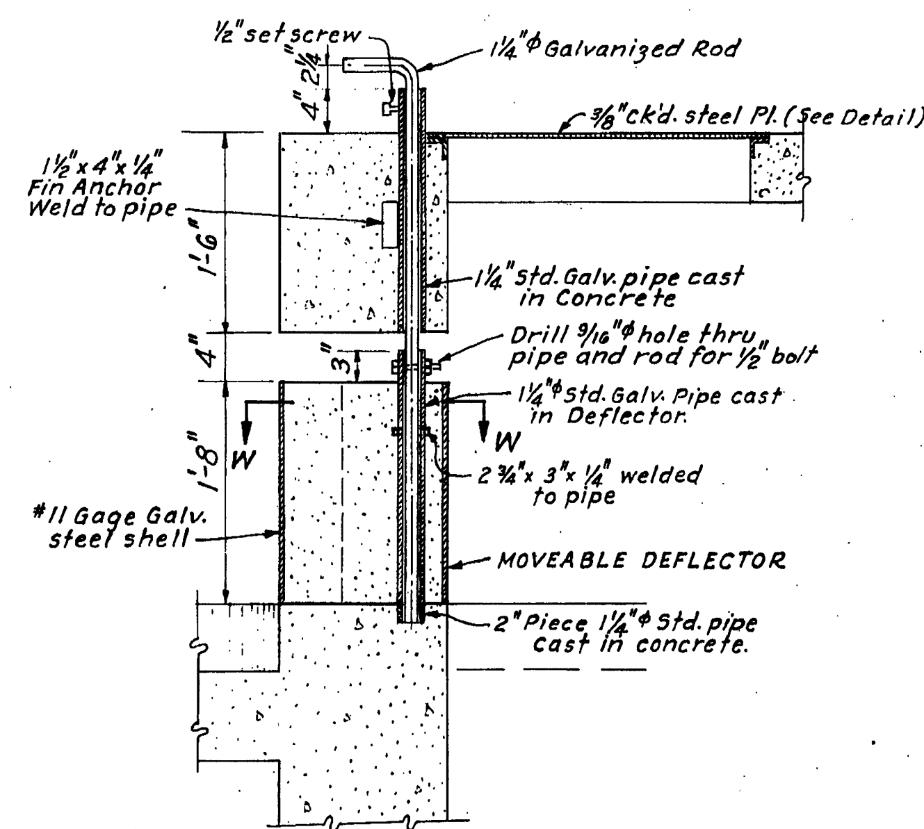
SECTION Y-Y
