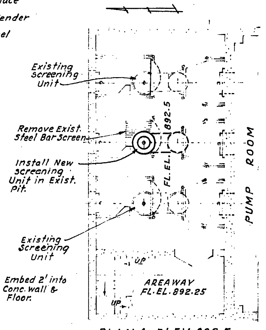
PLAN AT ELEV. 892.5 Scale: 1/2"=1'-0"
