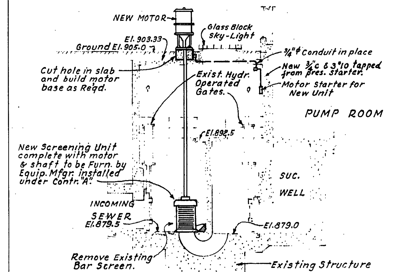
SECTION THRU NEW UNIT DETAILS OF NEW SCREENING UNIT INSTALLATION Scale: 1/2"=1'-0"
