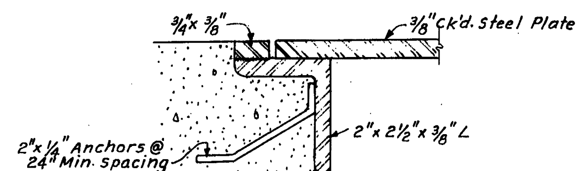
TYPICAL DETAIL OF FLOOR PLATE One Half Scale
