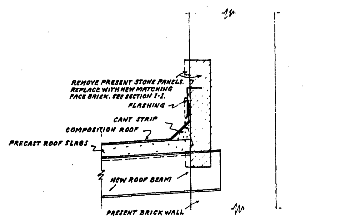
SECTION THRU PRESENT STONE PANELS SCALE 1" = 1'-0"
