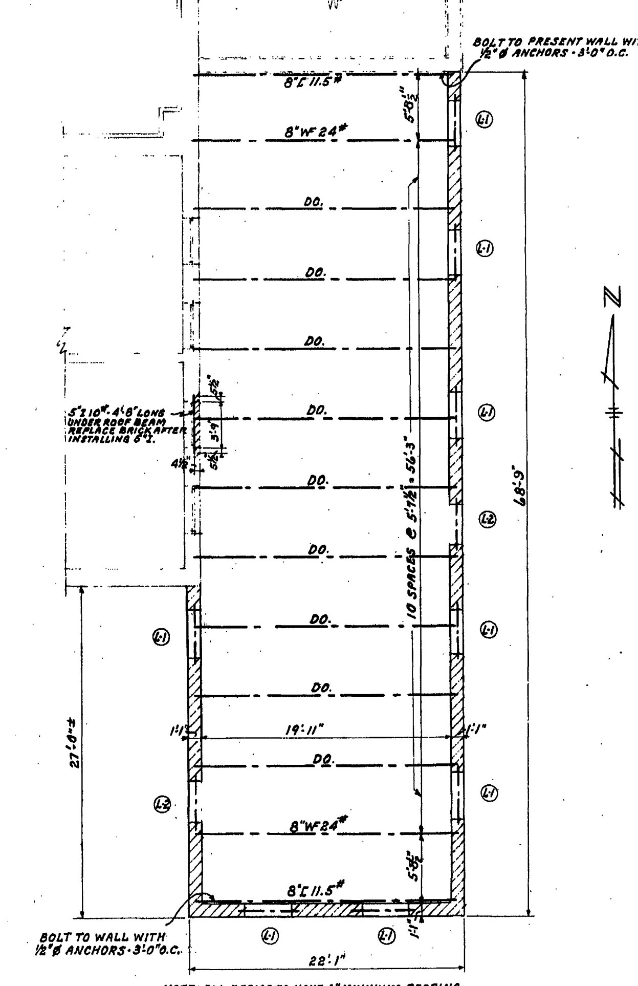
ROOF FRAMING PLAN SCALE 1/8" = 1'-0"
