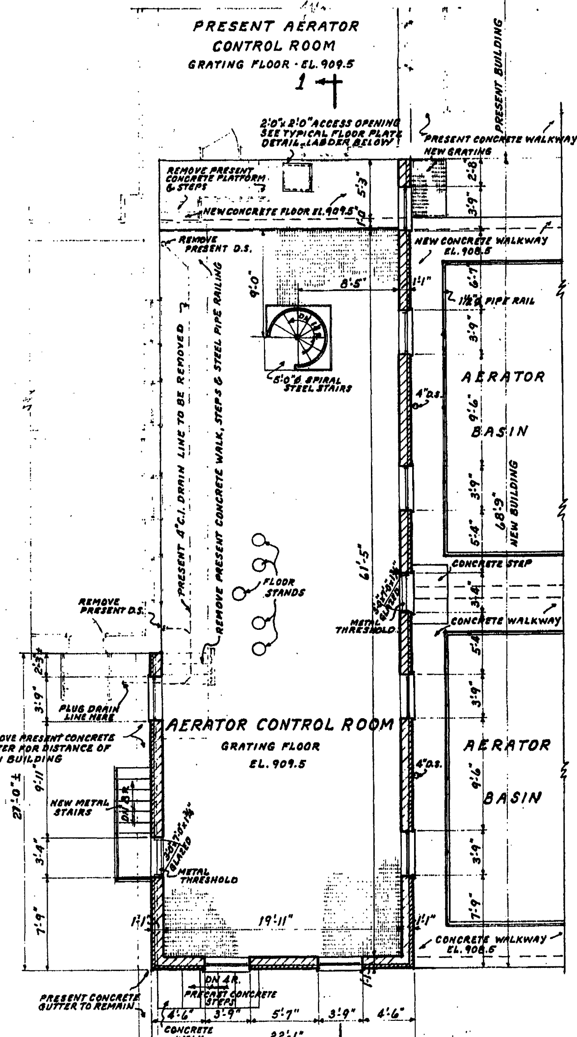
MAIN FLOOR PLAN SCALE 1/8" = 1'-0"
