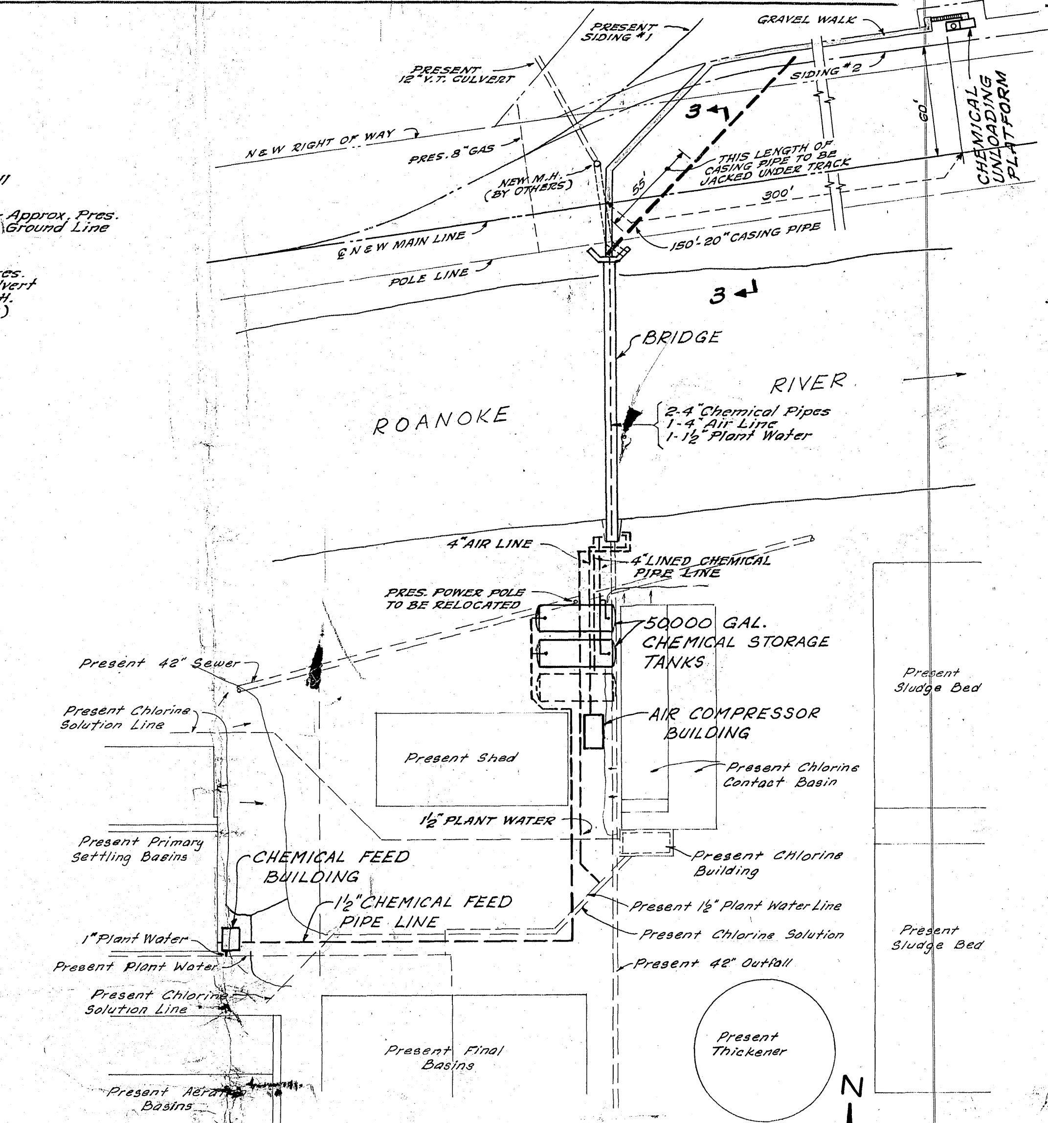
SITE PLAN Scale: 1" = 50'
