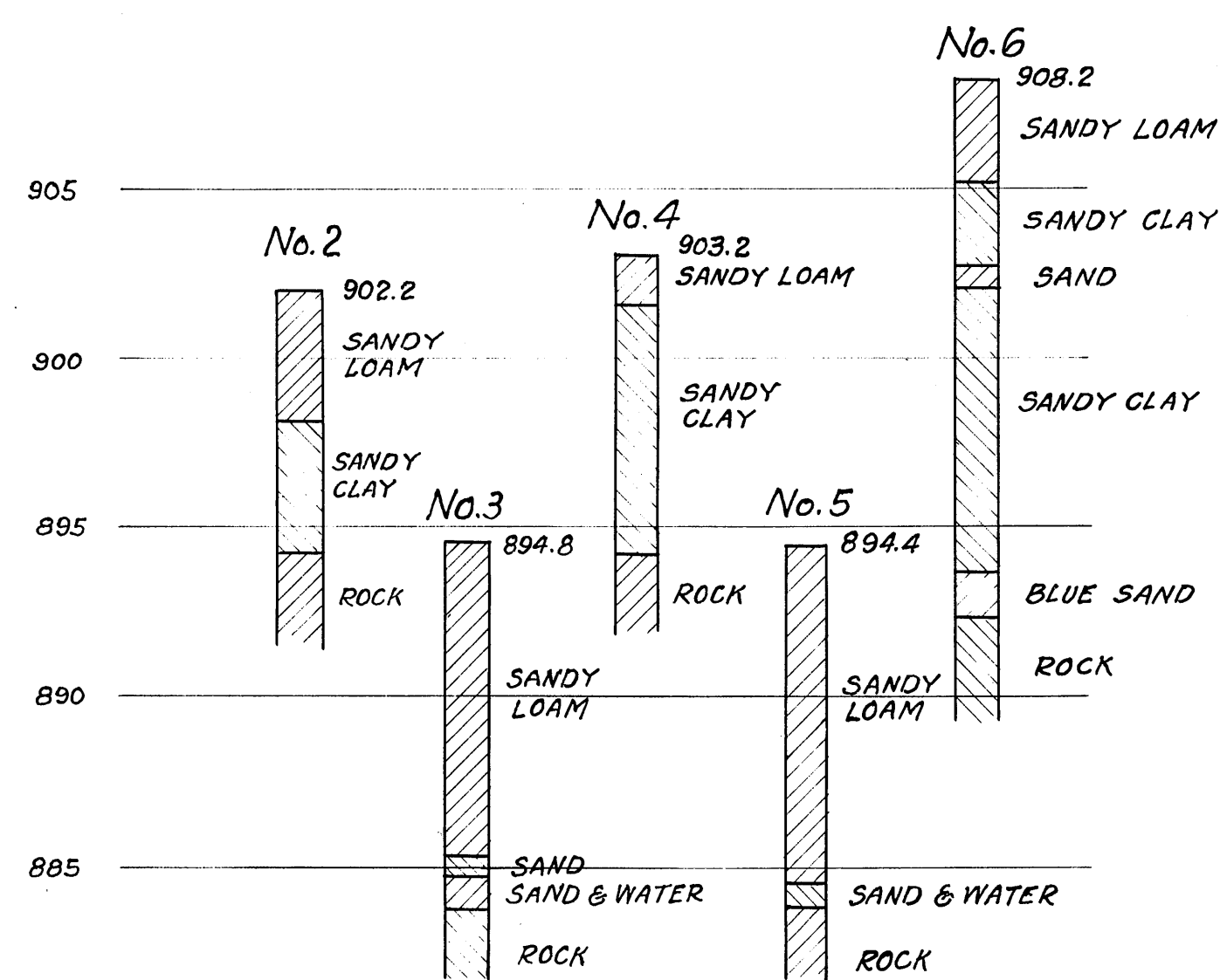
LOG OF TEST BORING
