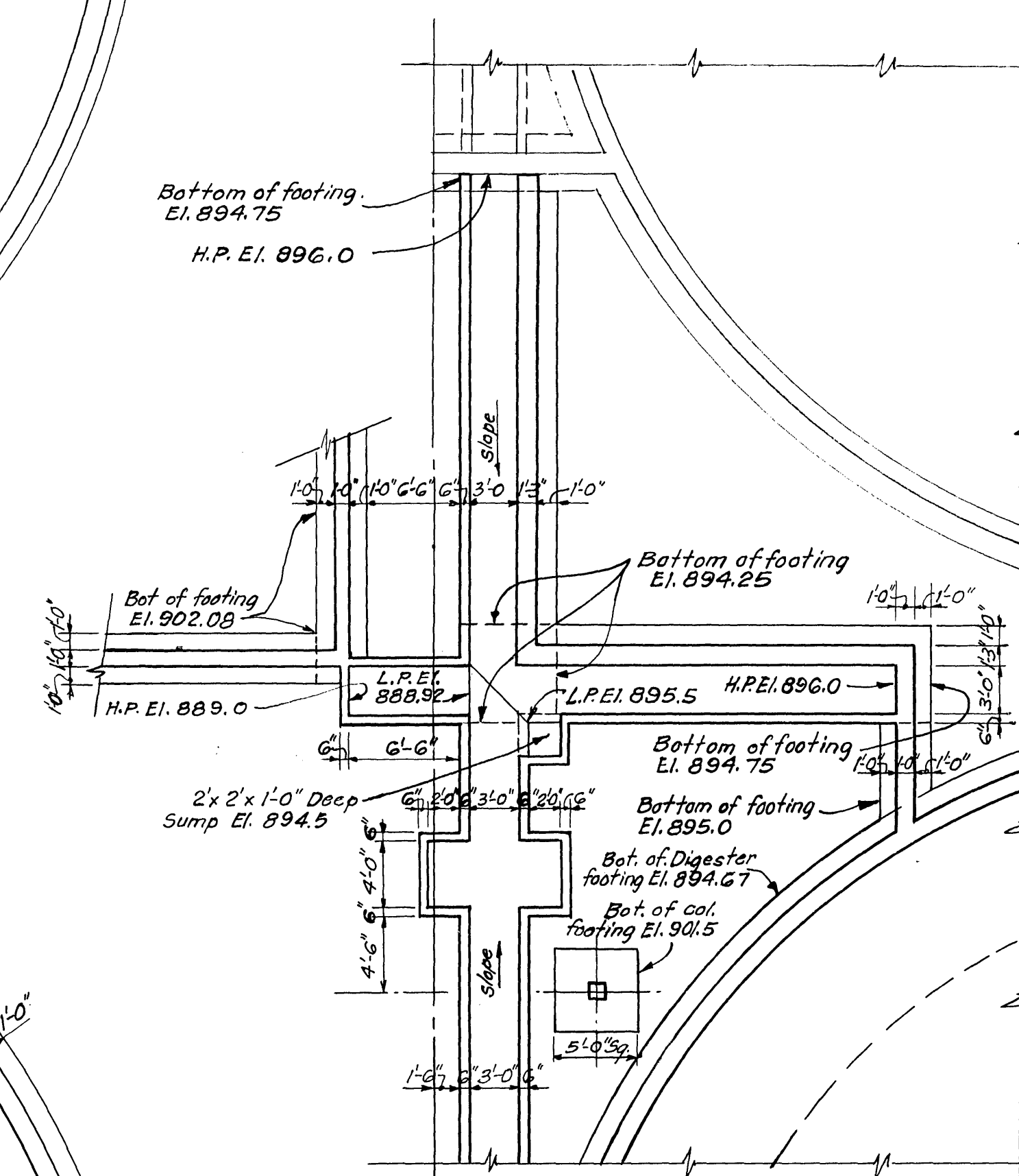
DETAIL PLAN LOWER FOOTING PLAN @ ELEV. 901± (DIGESTER CONTROL HOUSE) Scale: 1/8" = 1'-0"
