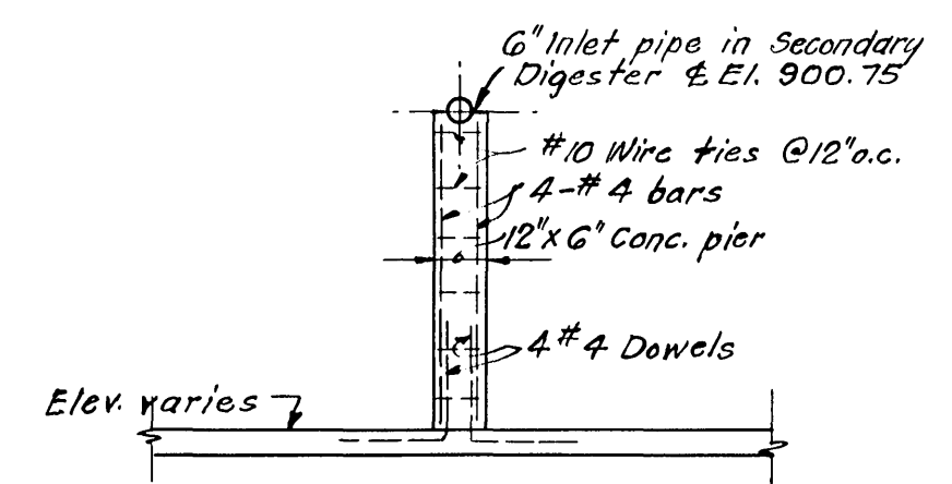
INLET PIPE PIER DETAIL Scale: 1/4" = 1'-0"
