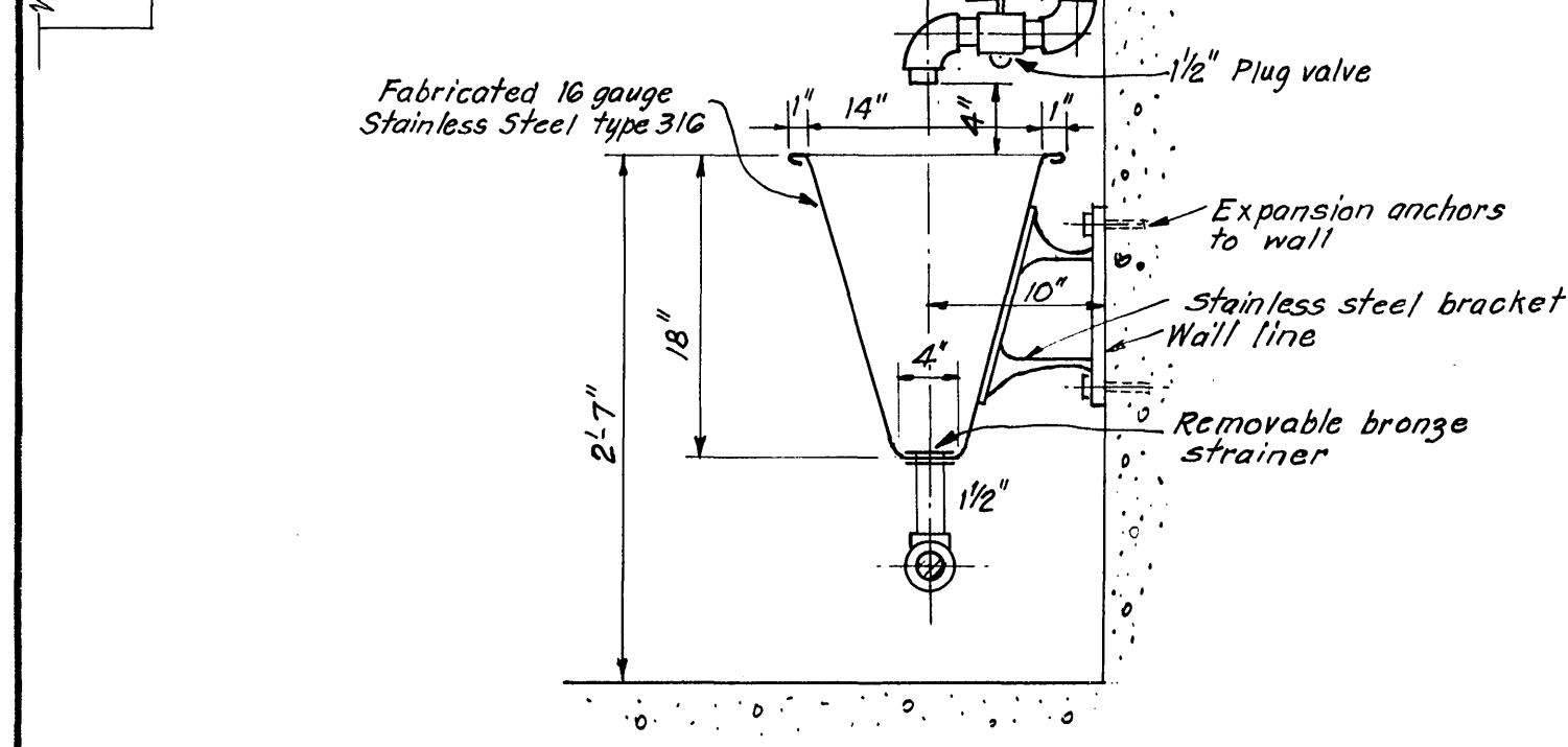
SAMPLE SINK DETAIL Scale: 1" = 1'-0"
