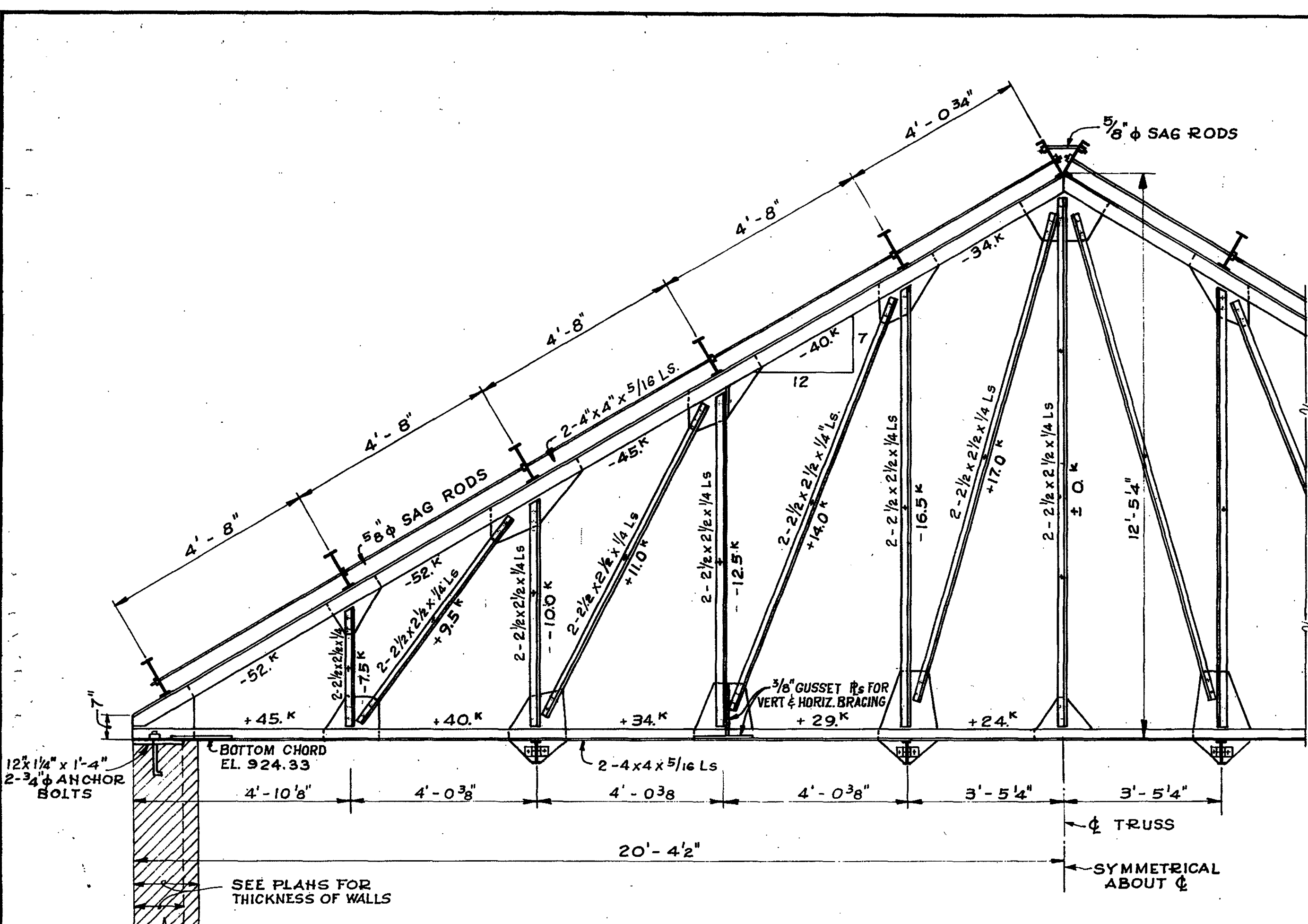
ROOF TRUSS OVER AIR INTAKE SPACE SCALE: 1/2" = 1'-0"
