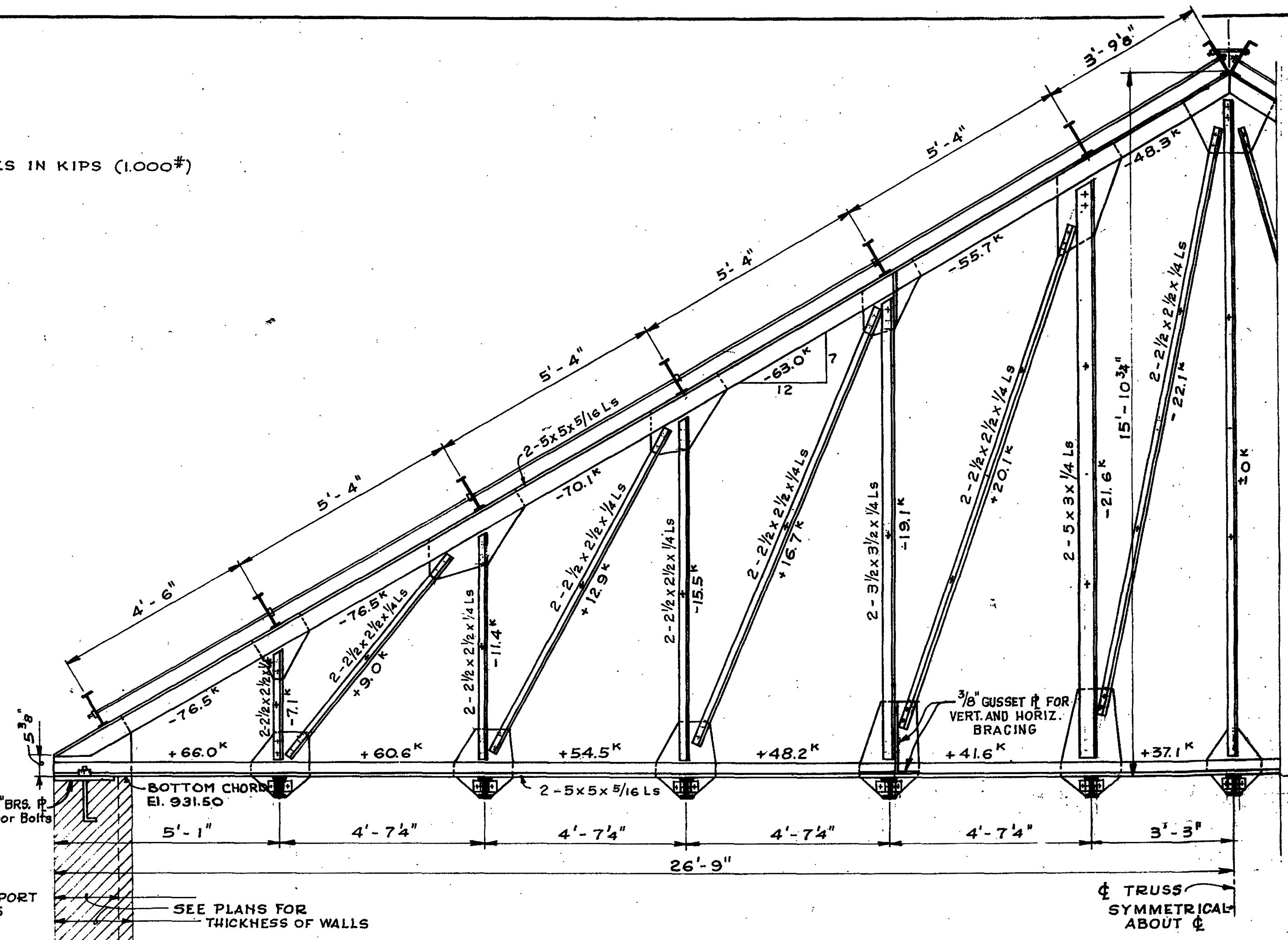
ROOF TRUSS OVER MEZZANINE SCALE: 1/2" = 1'-0"
