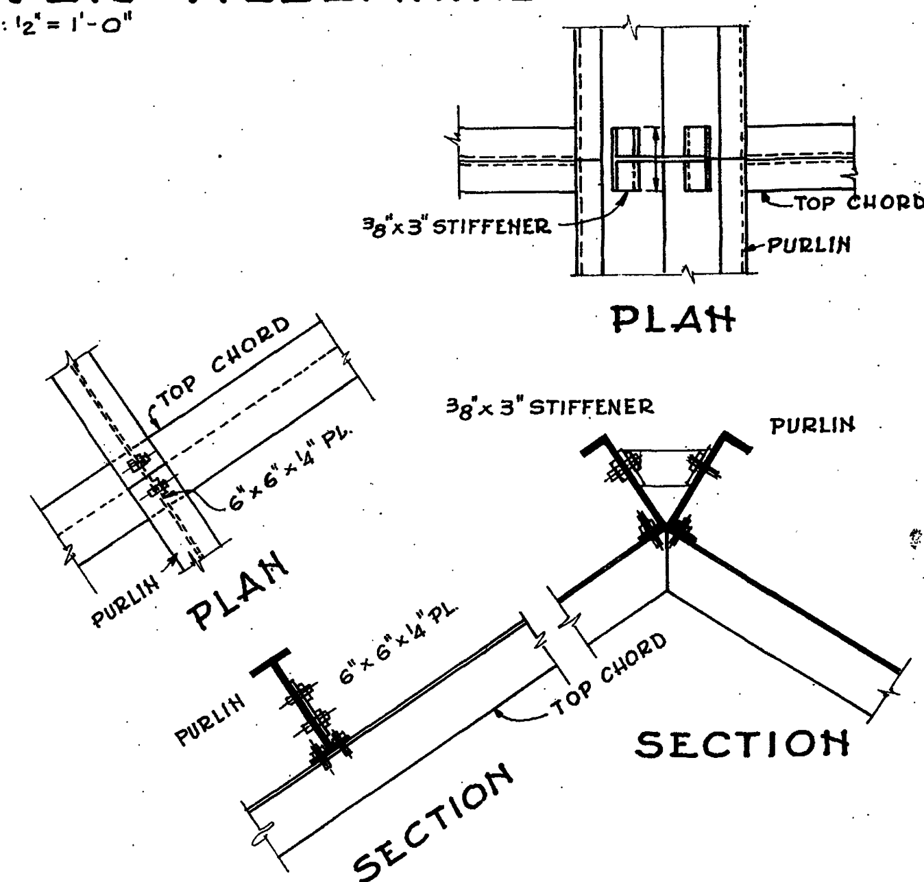
DETAILS OF PURLIN CONNECTIONS TO TRUSSES SCALE: 1'-1'-0"
