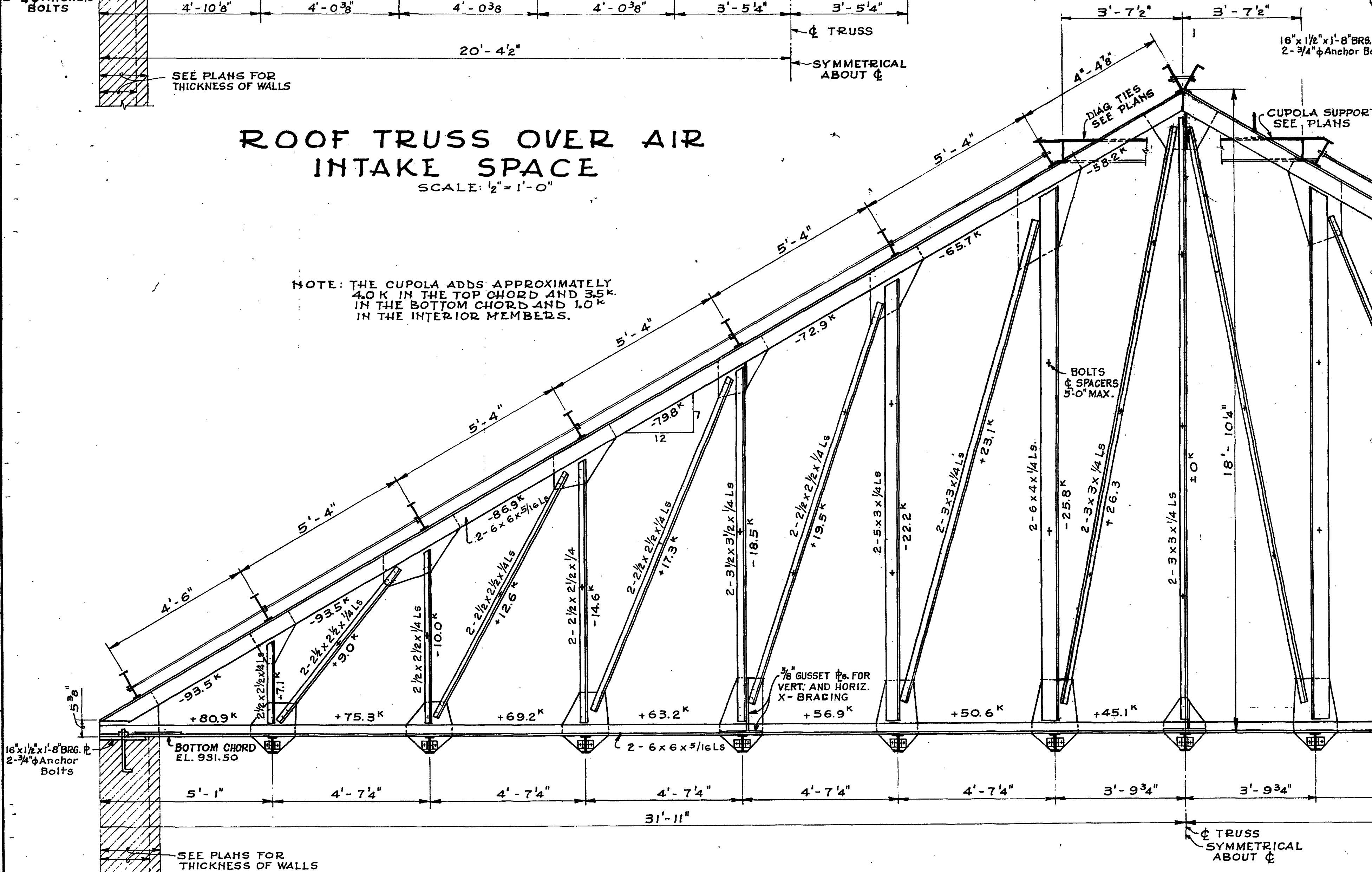
ROOF TRUSS OVER BLOWER ROOM SCALE: 1/2" = 1'-0"
