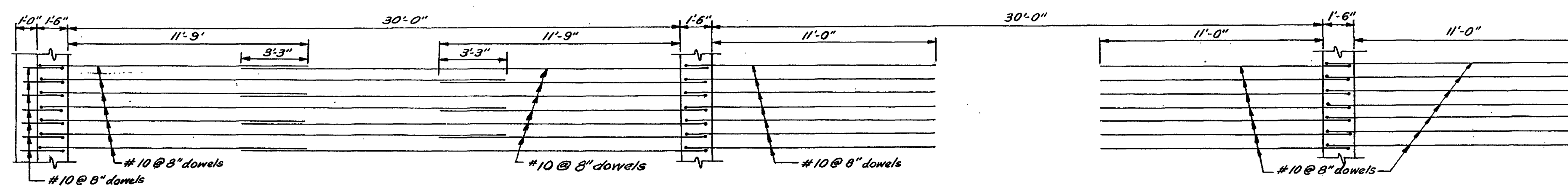
*TYPICAL REINFORCING IN BOTTOM OF FLOOR SLAB Scale: 1/4" = 1'-0"
