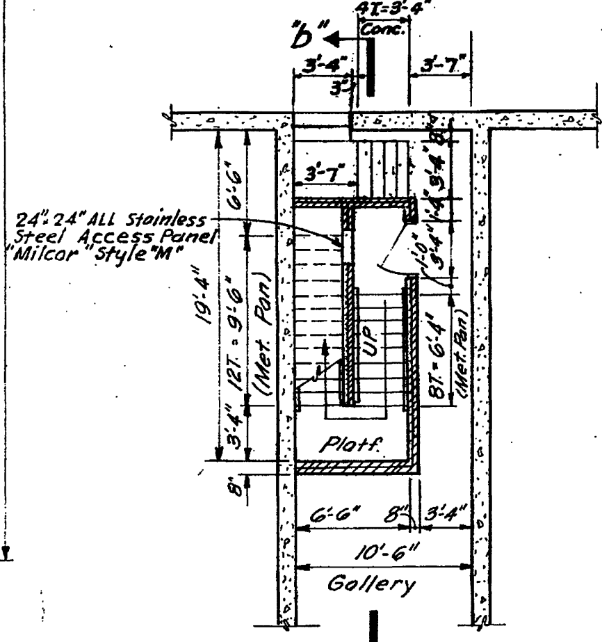
PLAN (Lower Level)
