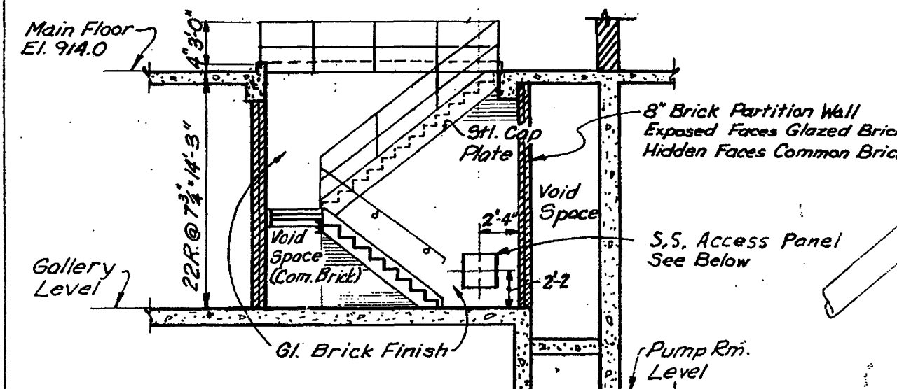
SECTION B-B
