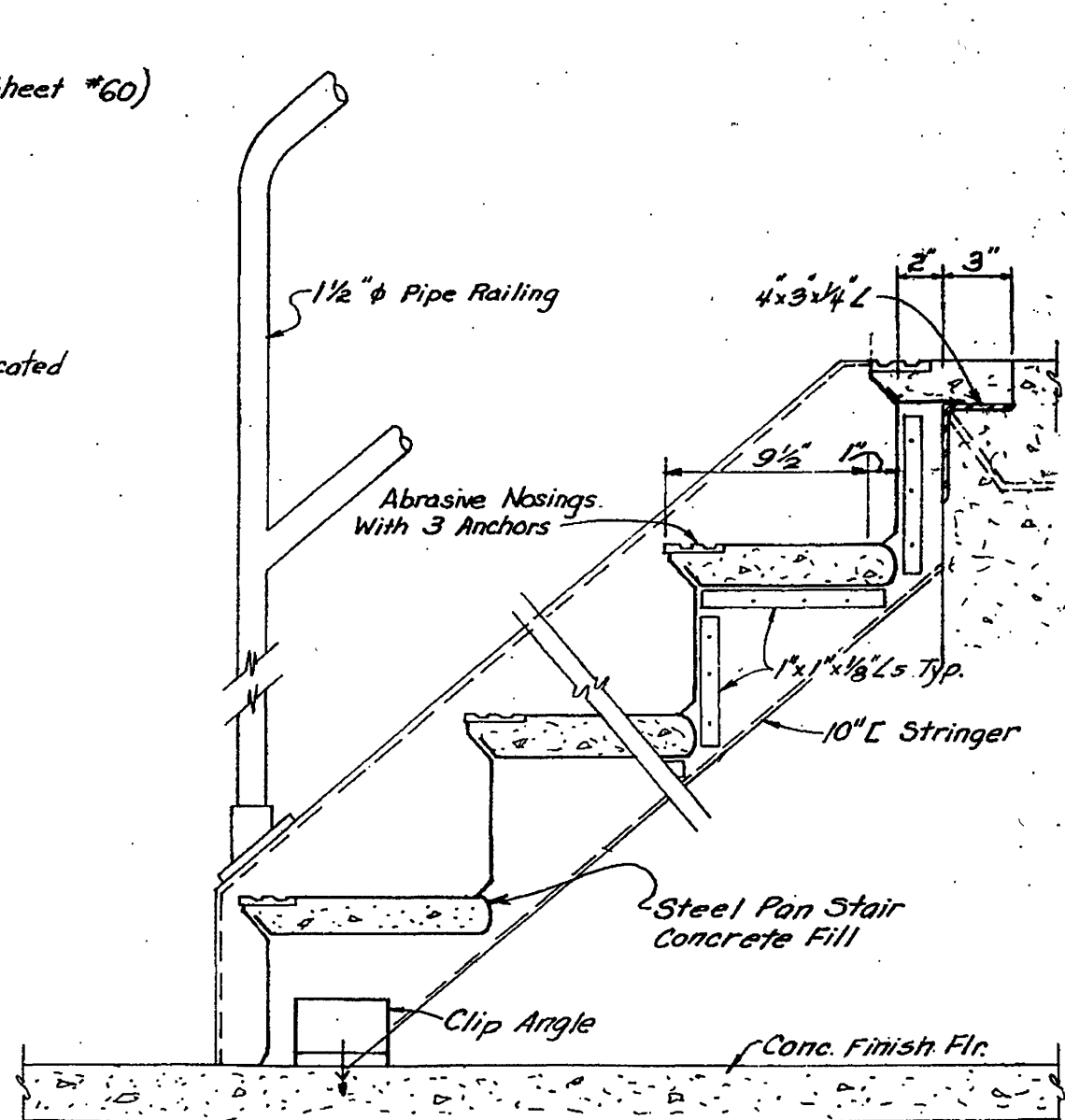
MET. PAN STAIR DETAIL SCALE: 1 1/2" = 1'-0" CONTR. "E"
