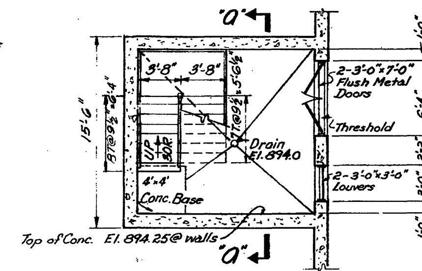
PLAN (Lower Level)
