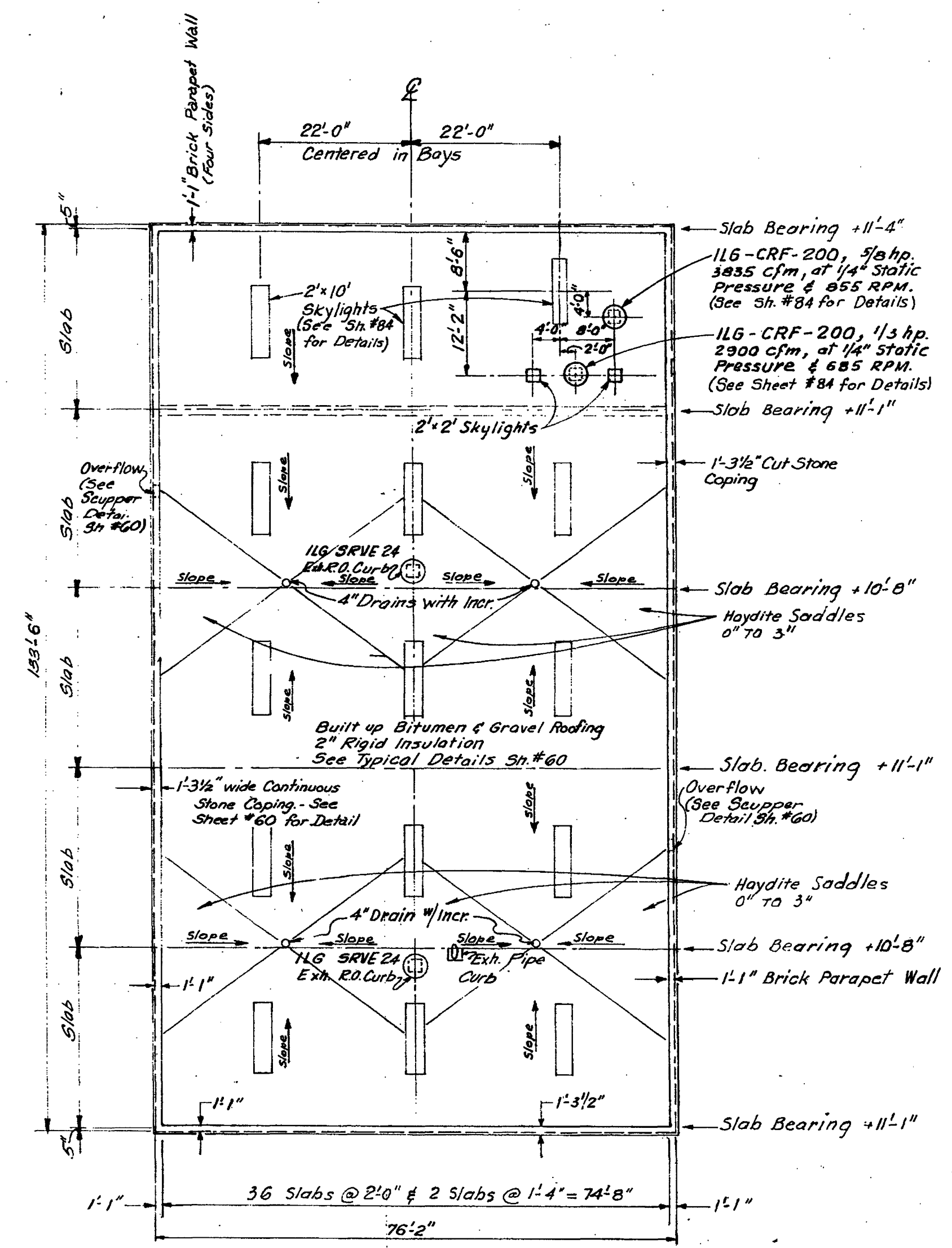
ROOF PLAN (See Coping & Curb Details Sheet #60) SCALE: 1/4" = 1'-0"
