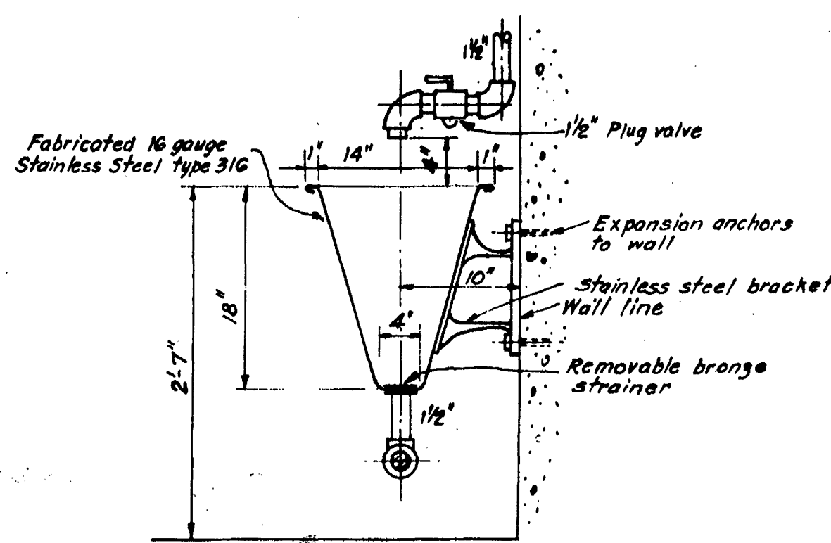
SAMPLE SINK DETAIL Scale: 1" = 1'-0"
