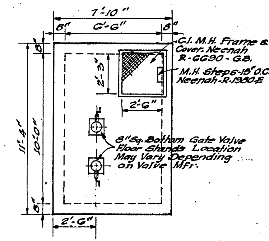
TOP OF CONC. PLAN Scale: 1/4" = 1'-0"
