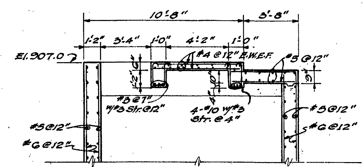
SECTION Z-Z
