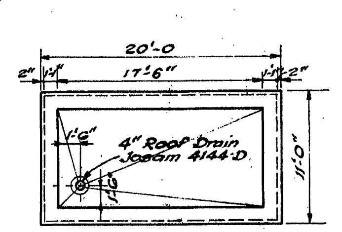
ROOF PLAN Scale: 1/8" = 1'-0"
