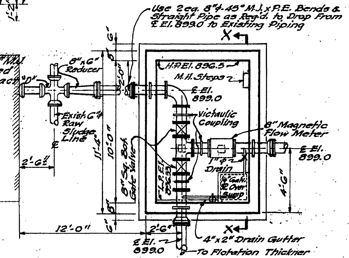
SECTIONAL PLAN Scale: 1/4" = 1'-0"
