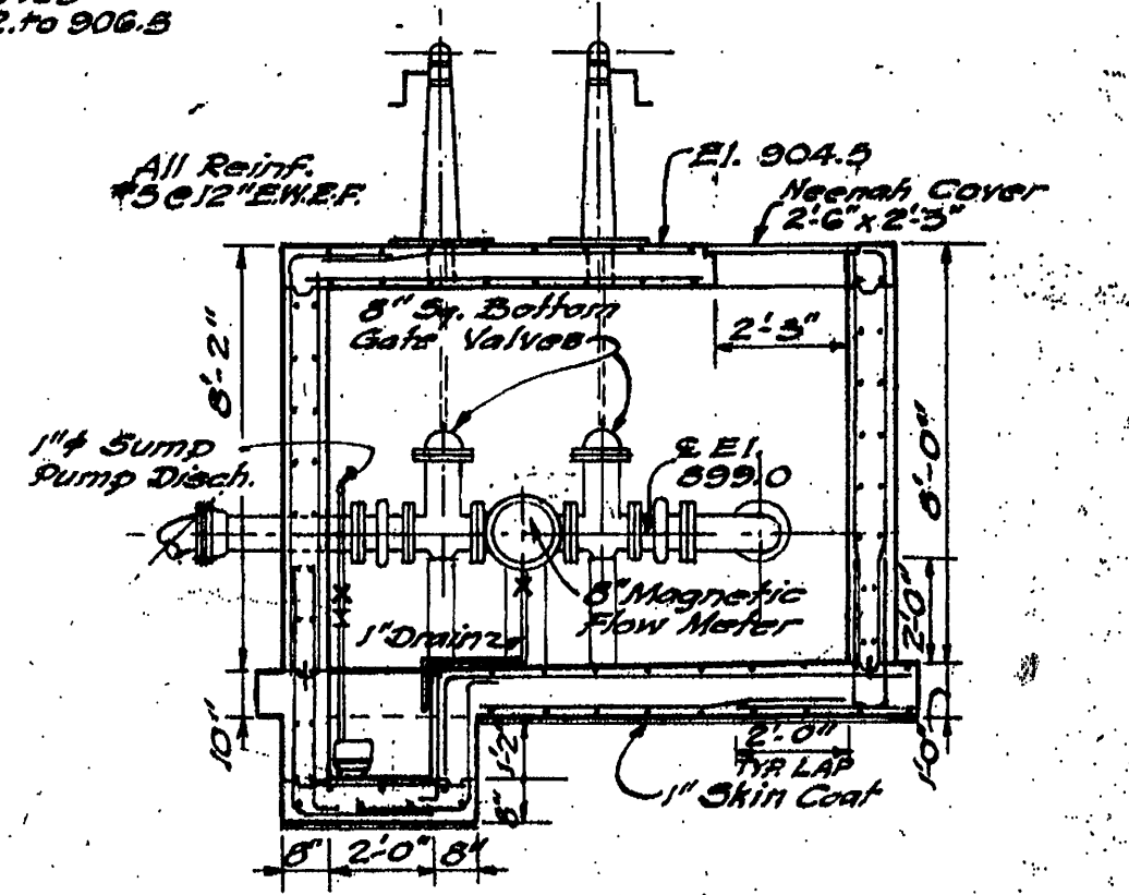
SECTION X-X DETAILS OF COAG. SLUDGE METER VAULT
