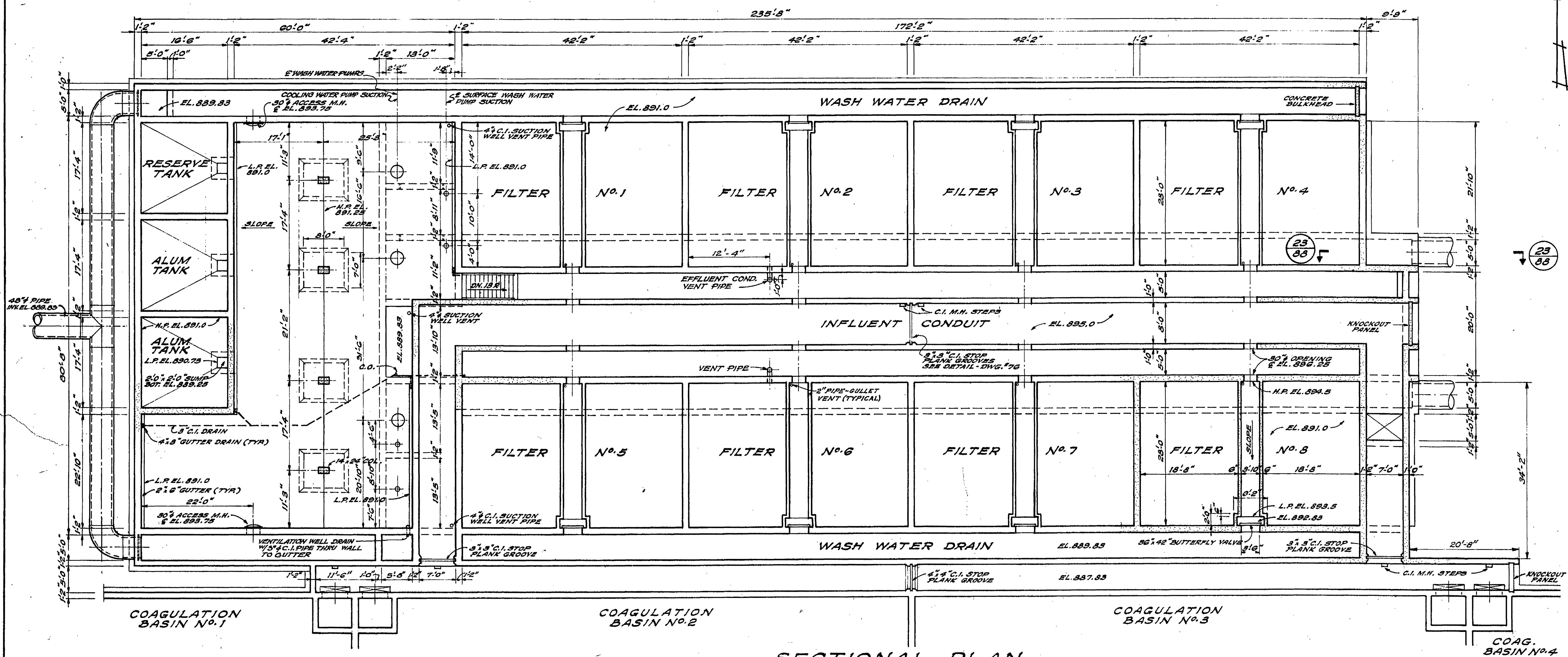
SECTIONAL PLAN
