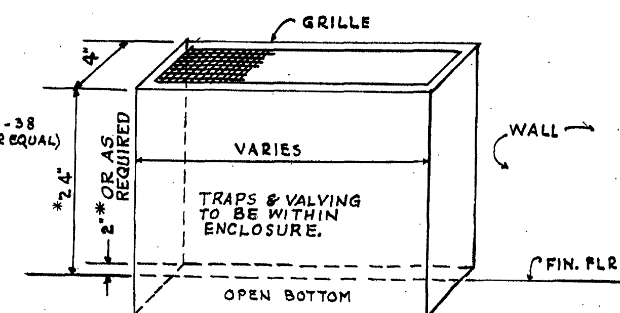
CONVECTOR TYPICAL FIN TUBE WALL MOUNT INSTALLATION NO SCALE
