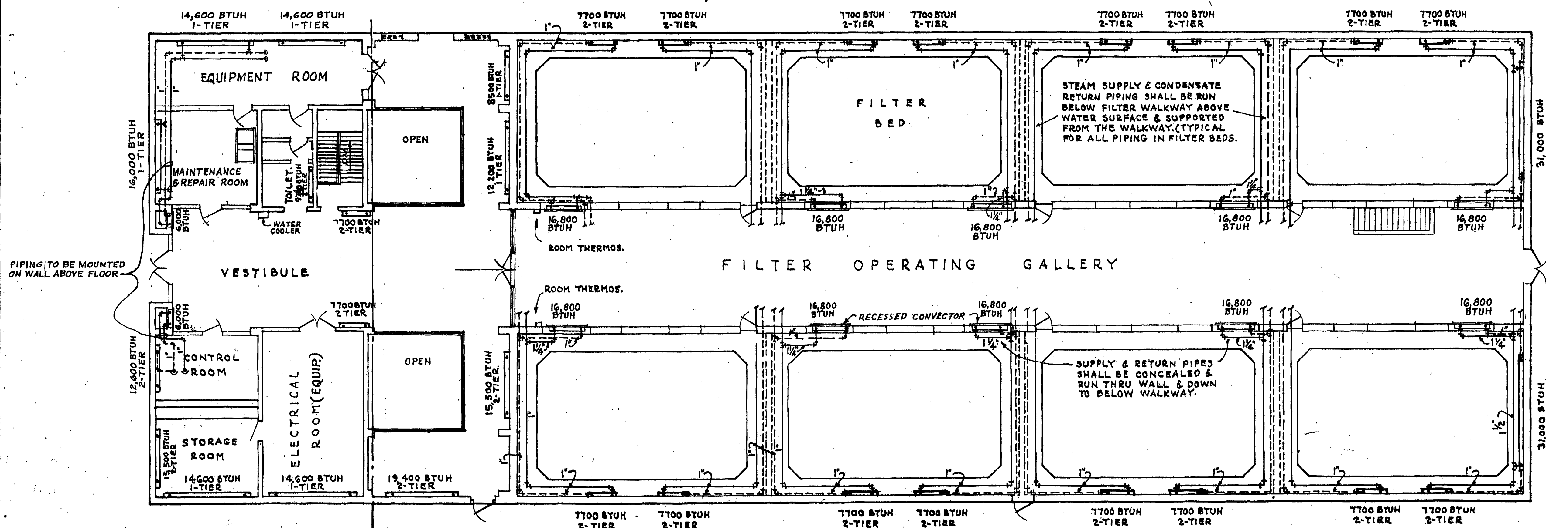
PLAN OF OPERATING GALLERY SCALE: 1" = 10'
