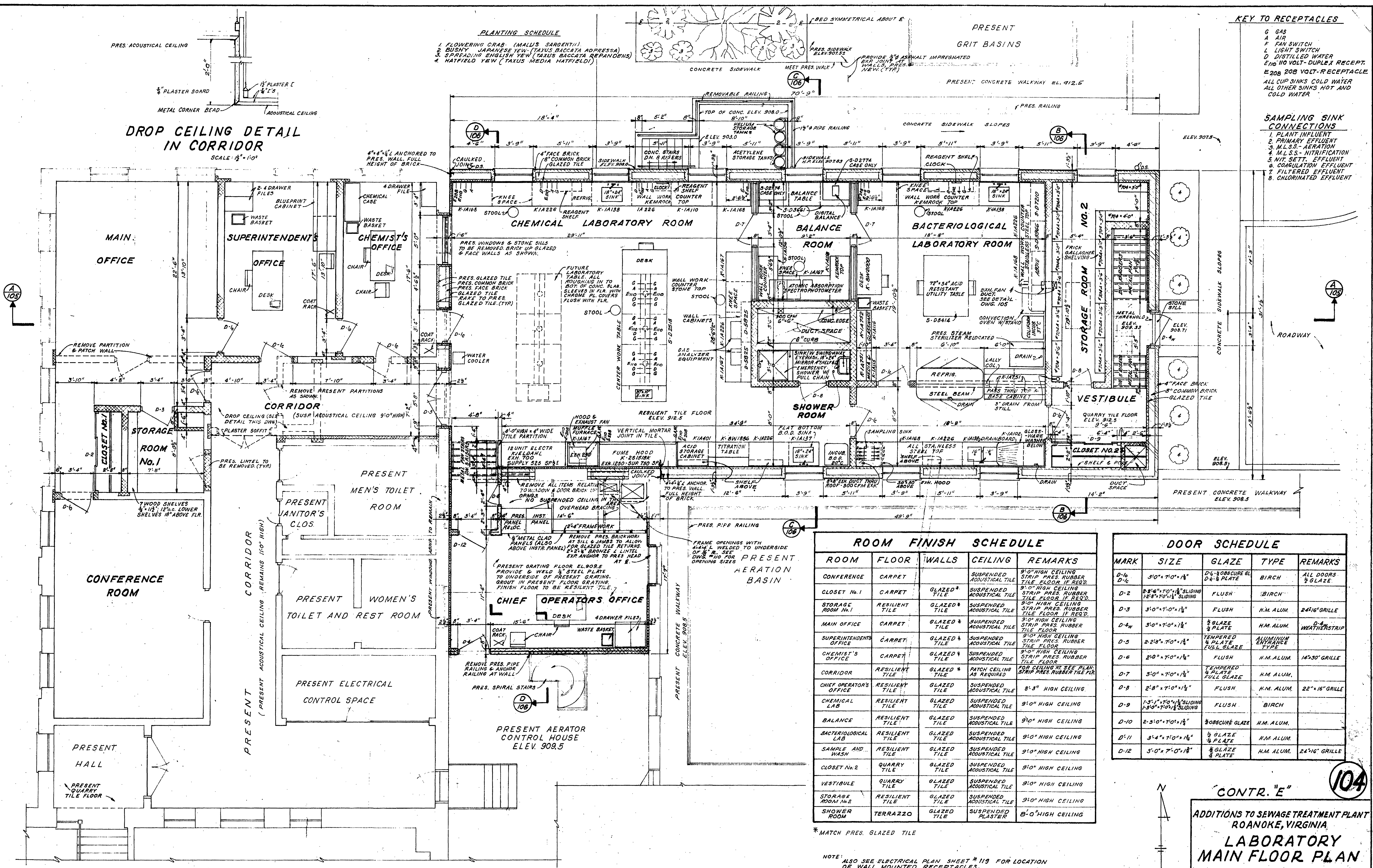
MAIN FLOOR PLAN SCALE: 1/8" = 1'-0"
